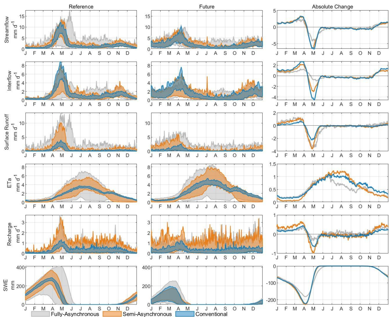
Figure E2. Same as E1, but for Ouelle catchment.
