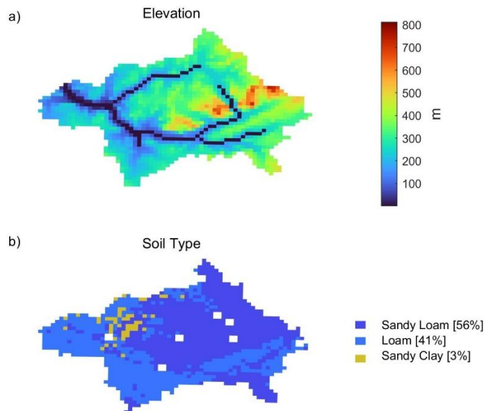
830 Figure F1. Topographic and soil type characteristics of the Matane catchment. Panel (a) shows the elevation map, with elevations ranging from 100 to 800 meters above sea level. Higher elevations are indicated in warmer colors (reds and oranges), while lower elevations are shown in cooler colors (blues and greens). Panel (b) displays the distribution of soil types within the catchment, with sandy loam covering 56% of the area (dark blue), loam covering 41% (light blue), and sandy clay occupying 3% (yellow).
