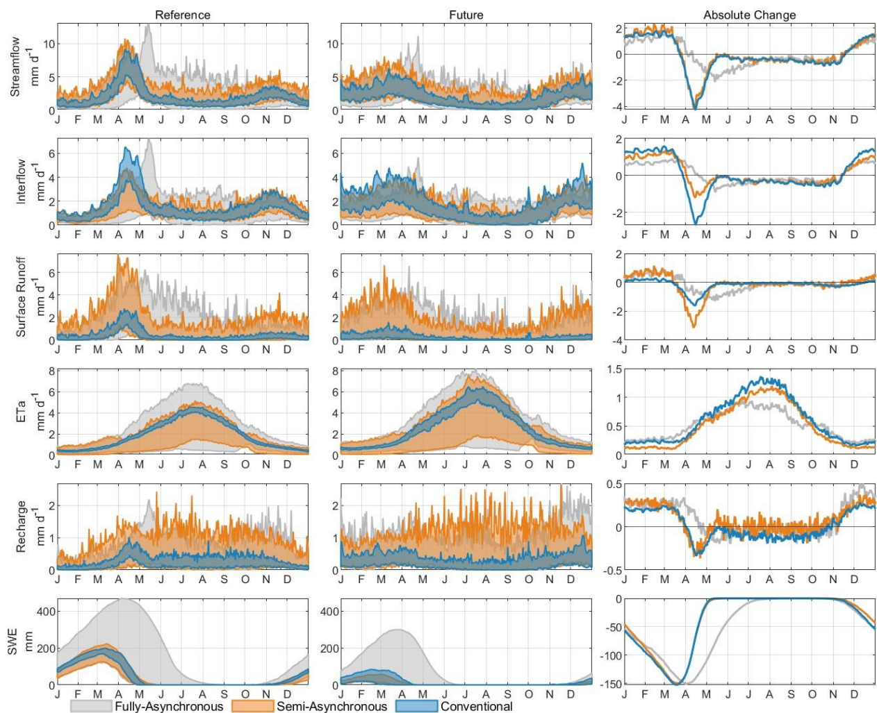
Figure E4. Same as E1, but for Nicolet Sud-Ouest catchment.
