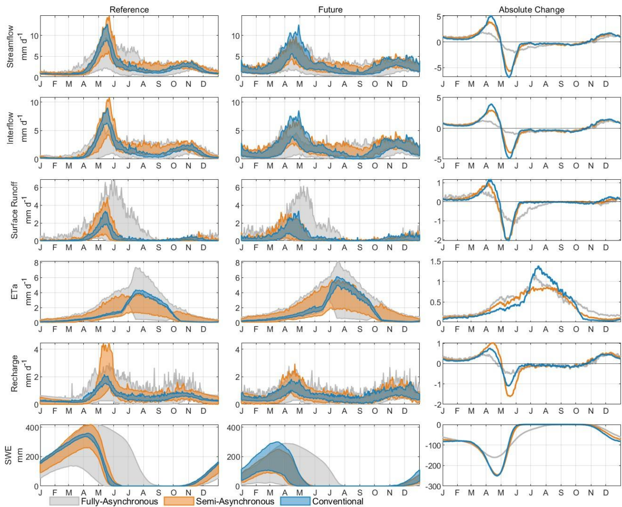
825 Figure E8. Same as E1, but for Valin catchment.
