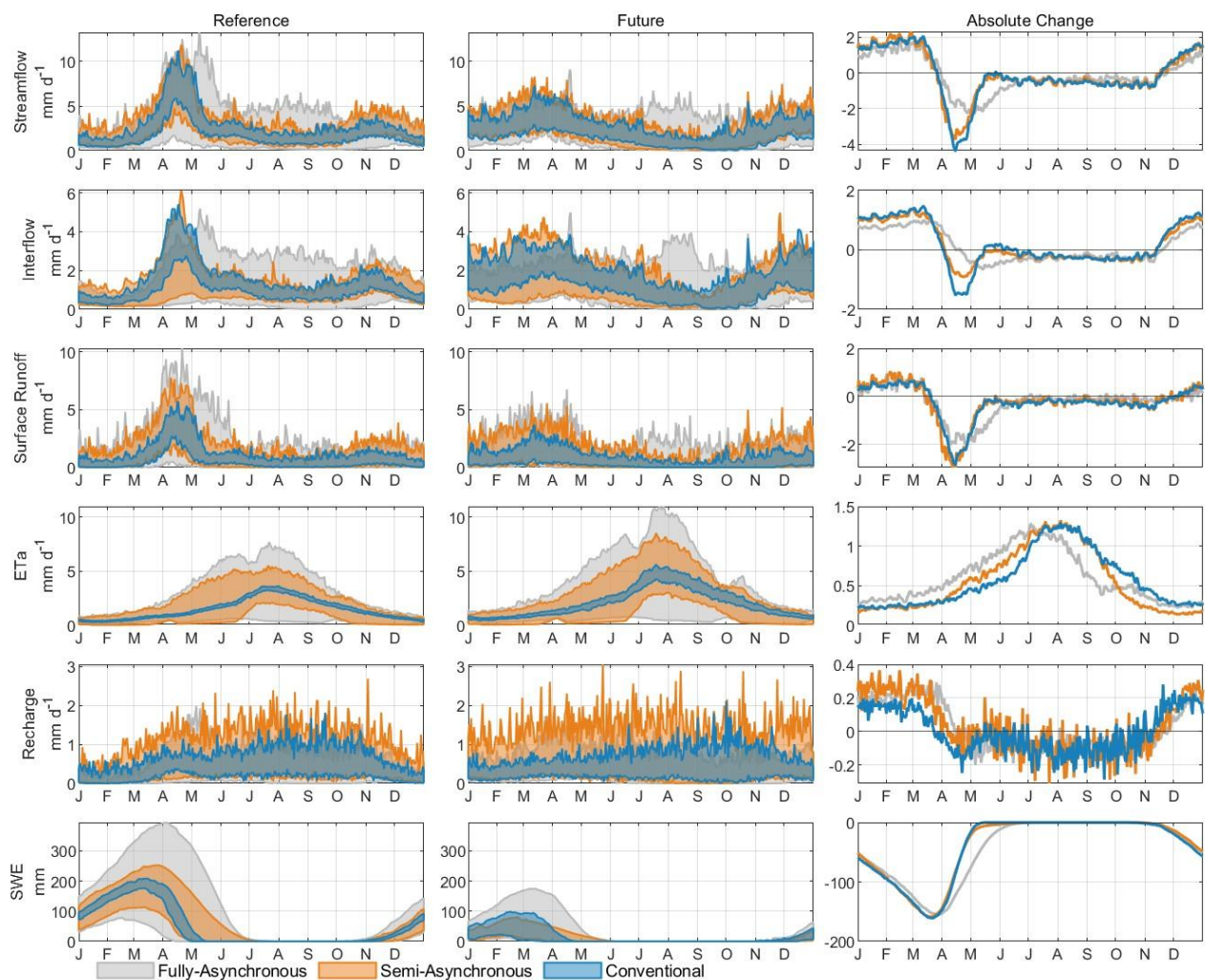
Figure E5. Same as E1, but for Au Saumon catchment.
