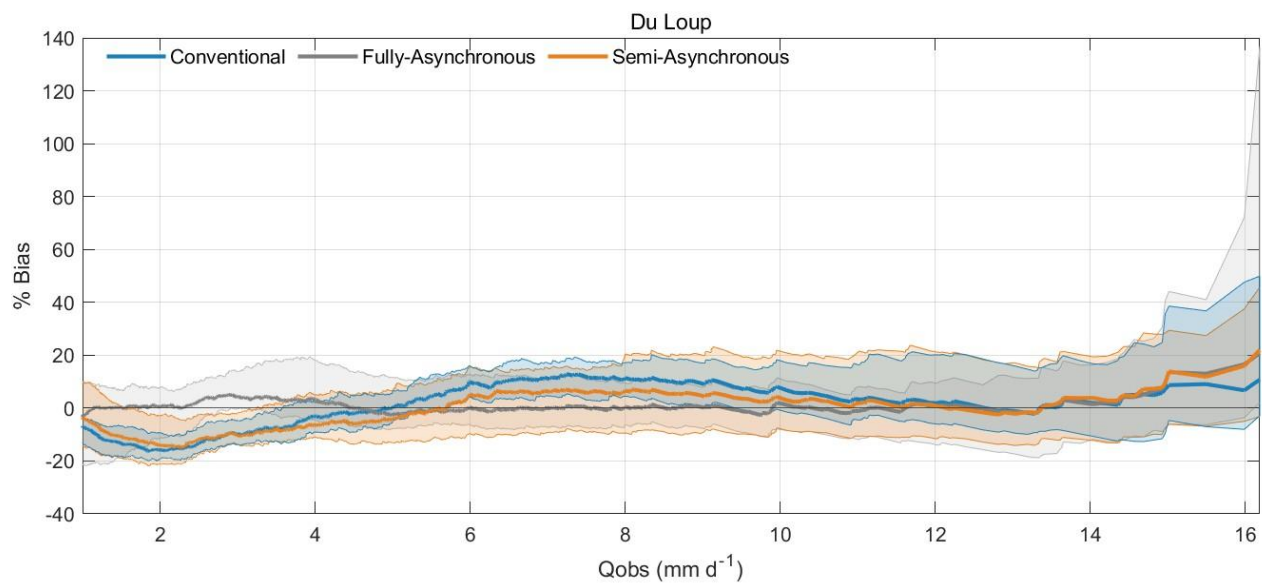
790 Figure C7. Same as Fig. C1, but for Du Loup catchment.
