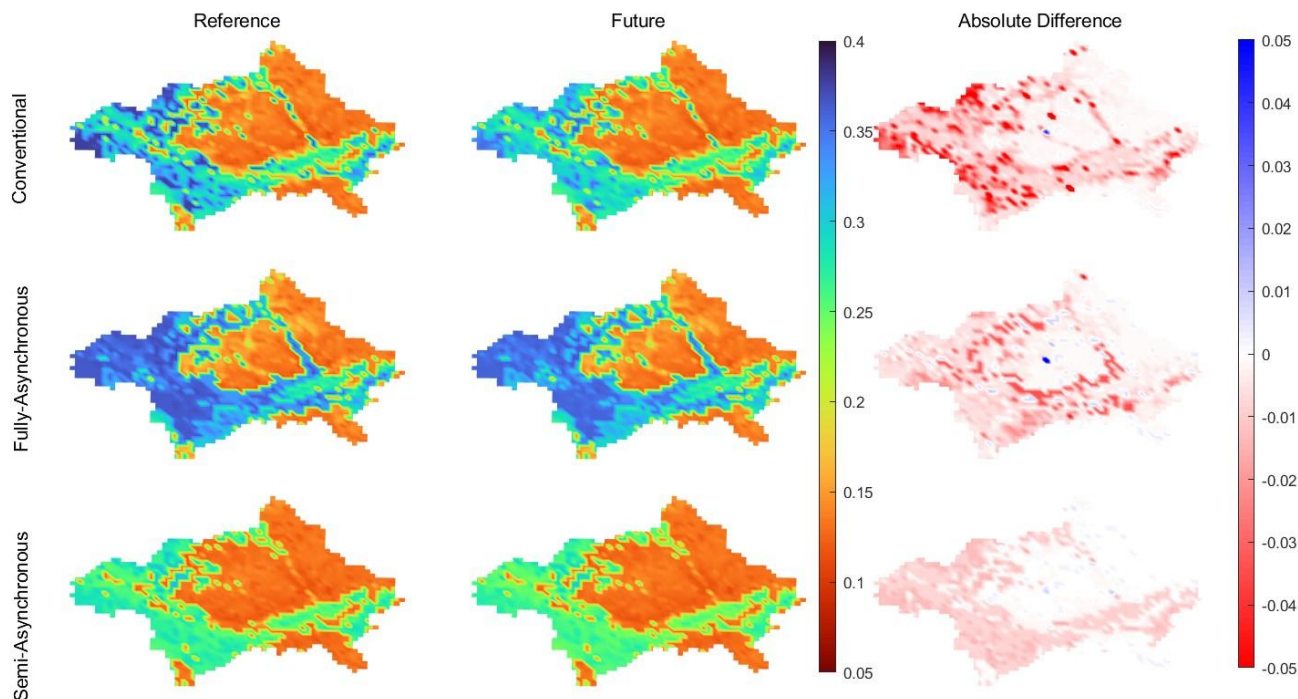
565 Figure 9. Spatial distribution of relative soil moisture in the Matane catchment for the reference period (1981–2010) and future period (2070–2099).
