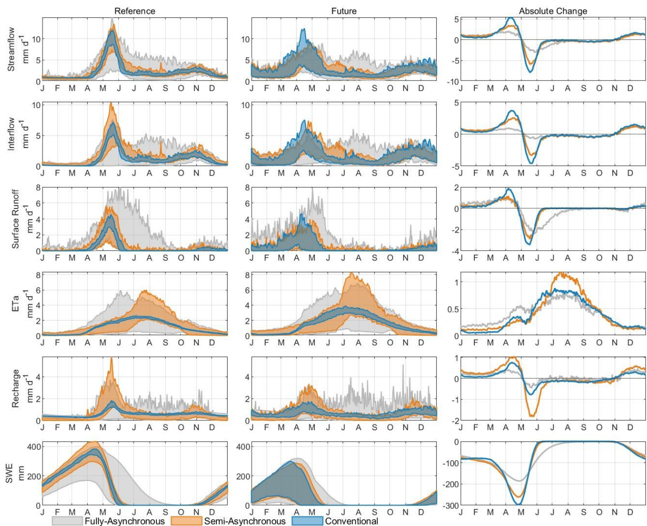
Figure E9. Same as E1, but for Godbout catchment.
