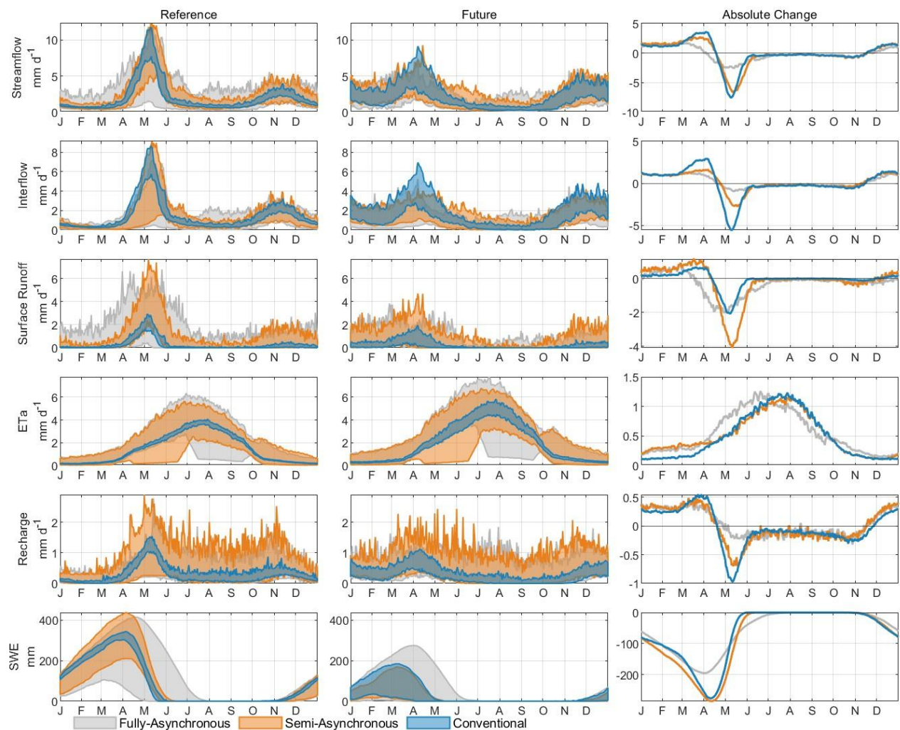
810 Figure E1. Seasonal distribution of key hydroclimatic variables for the reference period (1981–2010), future period (2070–2099), and their average absolute changes across the Bonaventure catchment.
