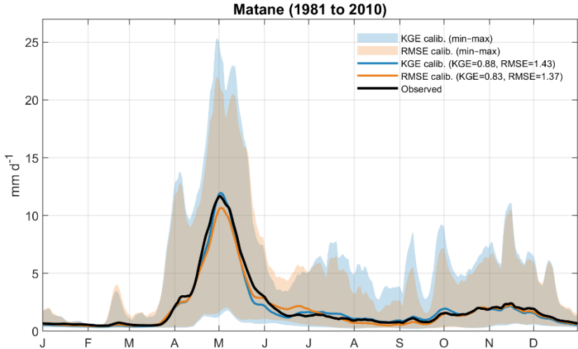
Figure G2. Seasonal streamflow comparison between the conventional method calibrated using RMSE and KGE and observed data across the Matane catchment.
