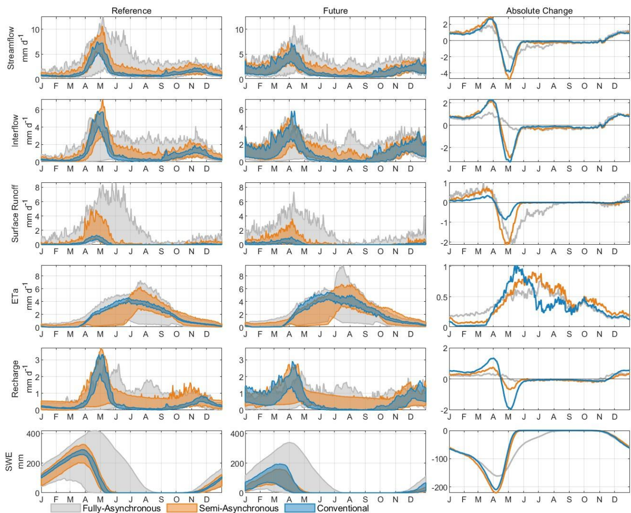
Figure E7. Same as E1, but for Du loup catchment.
