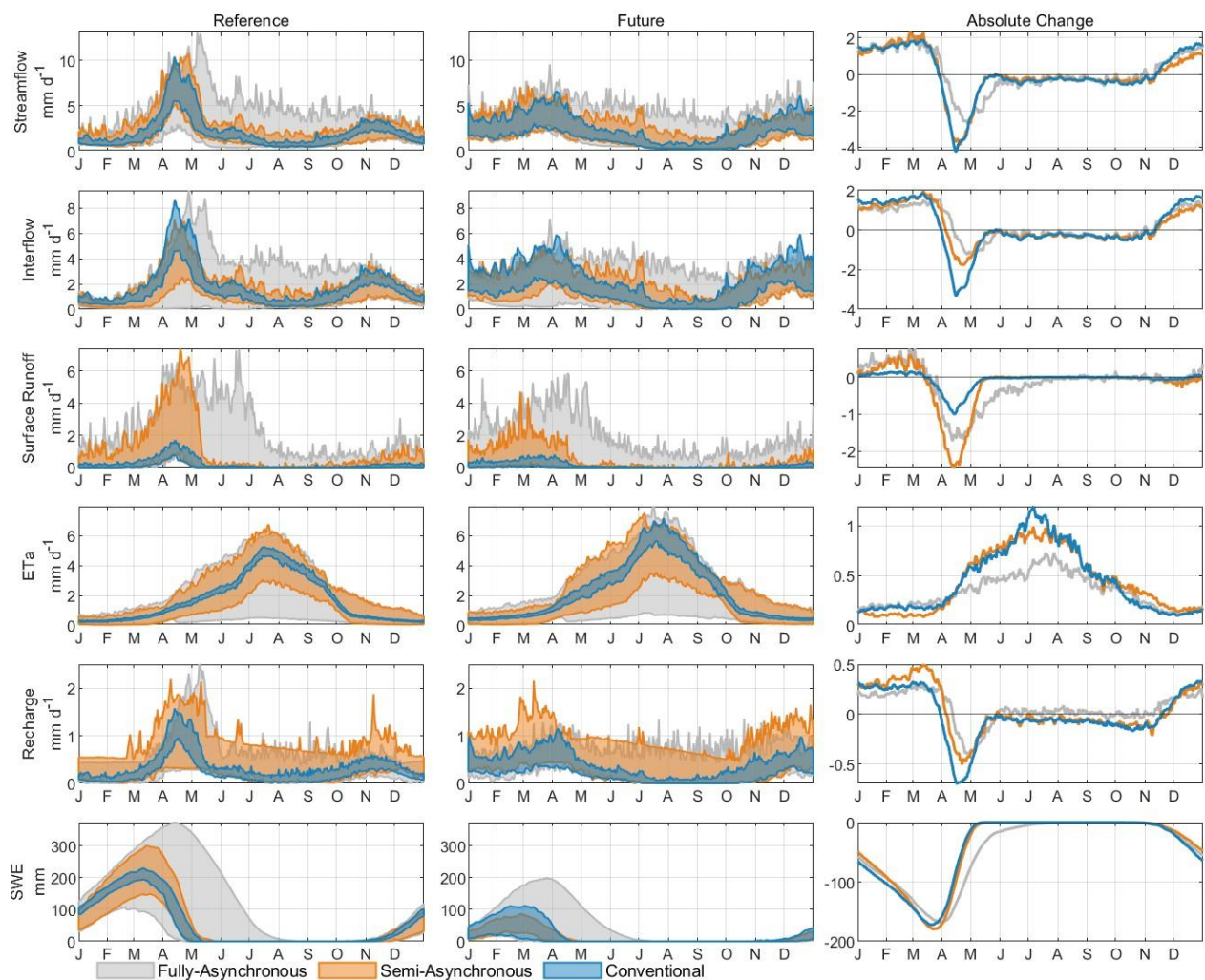
815 Figure E3. Same as E1, but for Bécancour catchment.
