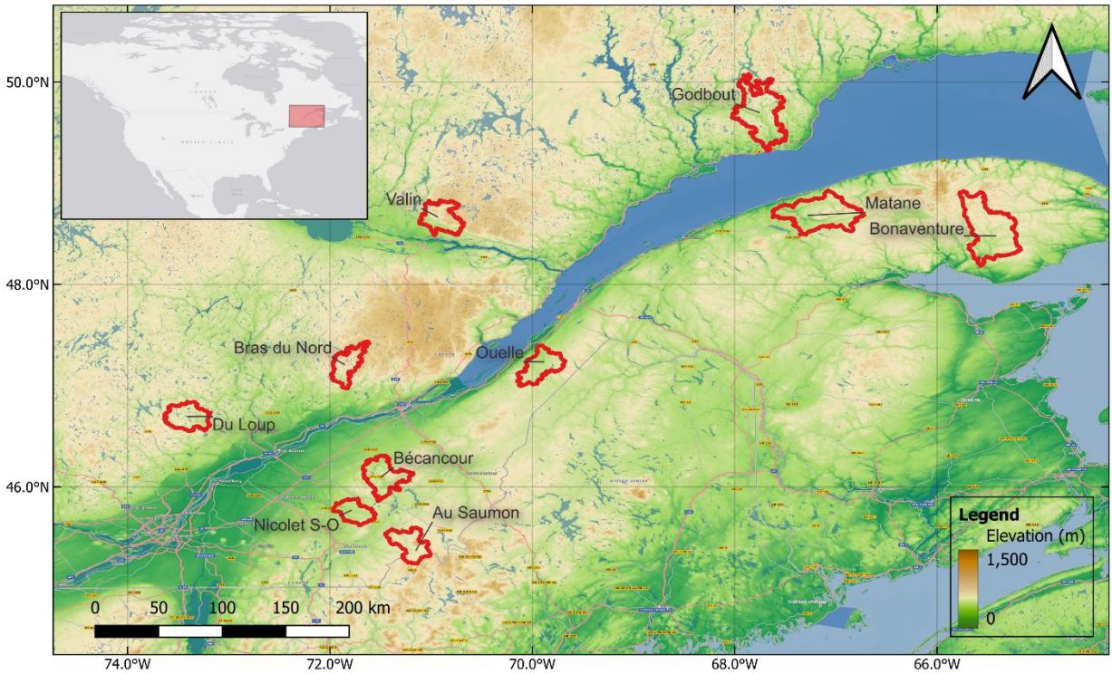
125 Figure 1. Locations of the selected catchments within Southern Quebec, Canada, outlined in red. The inset map provides the location of the study area within North America.
