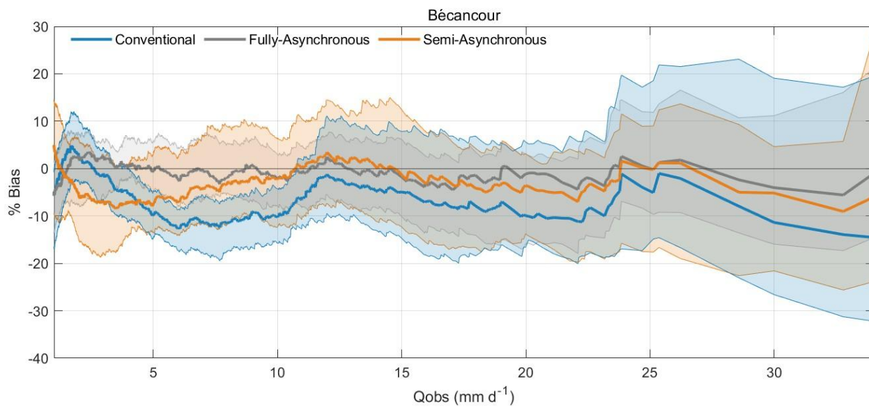
830 Figure C3. Same as Fig. C1, but for Bécancour catchment.
