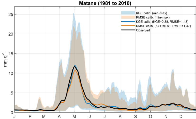
890 Figure G2. Seasonal streamflow comparison between the conventional method calibrated using RMSE and KGE and observed data across the Matane catchment.
