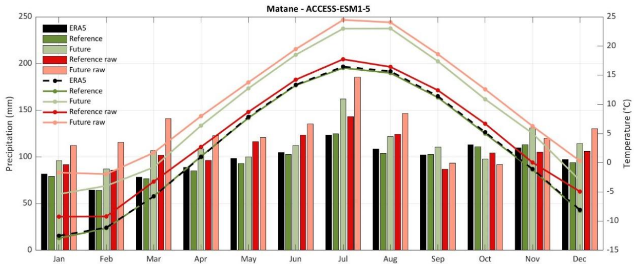
Figure 6. Comparison of average monthly precipitation and temperature for the Matane catchment. Bars represent monthly total precipitation (mm), while lines represent monthly mean temperature (°C). Black corresponds to the ERA5 reference dataset. Green shades represent bias-corrected climate model simulations (reference and future periods), while red shades represent raw climate model outputs (i.e., without bias correction). Darker colors indicate the reference period (1981–2010), and lighter colors indicate the future period (2070–2099) under the SSP5-8.5 scenario. This figure displays the average monthly temperature and precipitation for the Matane catchment during the reference period (1981–2010) and the future period (2070–2099) under the Shared Socioeconomic Pathway 5-8.5 (SSP585) scenario.
