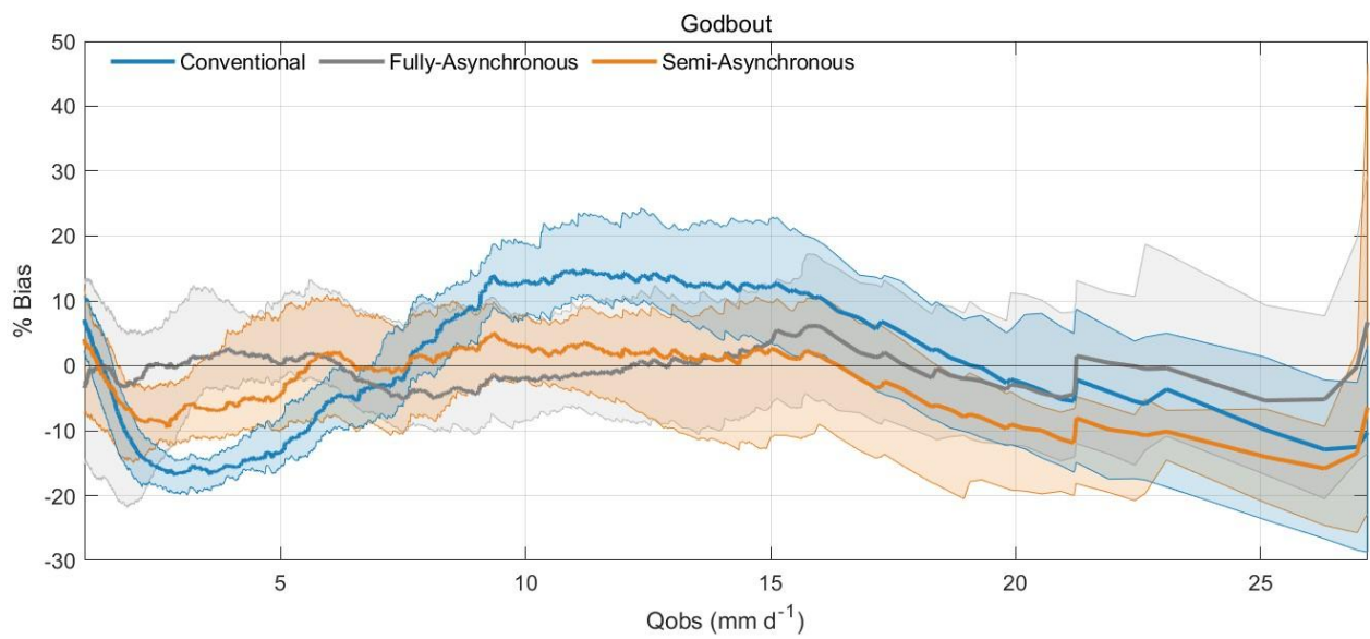
Figure C9. Same as Fig. C1, but for Godbout catchment.
