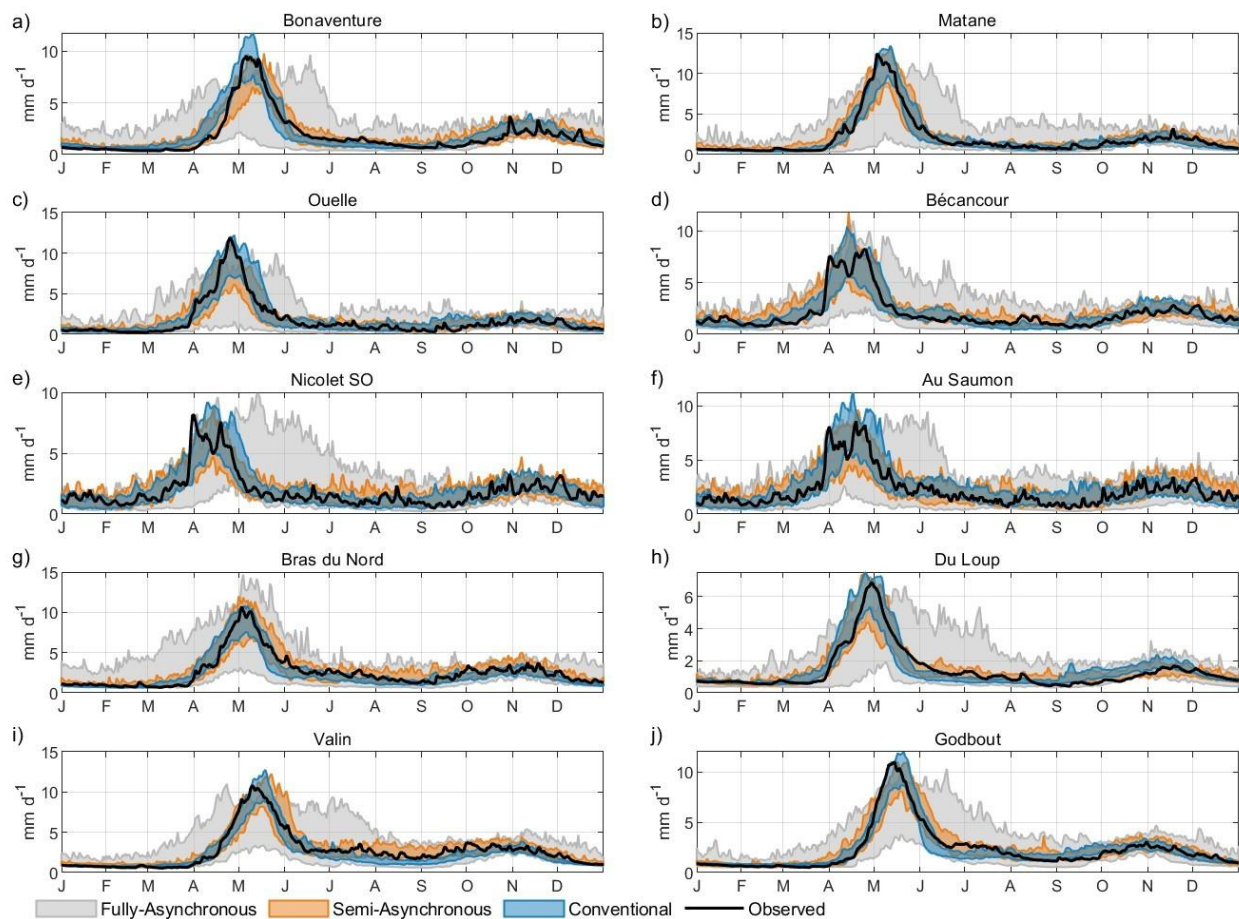
Figure 3. Seasonal streamflow comparison between the fully asynchronous, semi-asynchronous and conventional methods and observed data across ten catchments during the reference period (1981–2010). The panels (a-j) represent the catchments of Bonaventure, Matane, Ouelle, Bécancour, Nicolet SO, Au Saumon, Bras du Nord, Du Loup, Valin, and Godbout, respectively.
