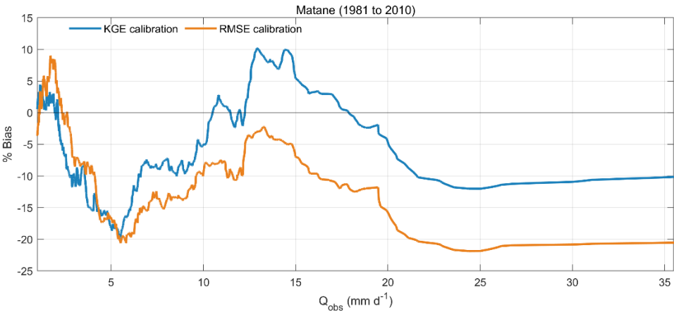
885 Figure G1. Performance comparison between the conventional method calibrated using RMSE and KGE for the Matane catchment during the reference period (1981–2010). The figure shows the percentage bias between observed and simulated streamflows obtained using meteorological observations.
