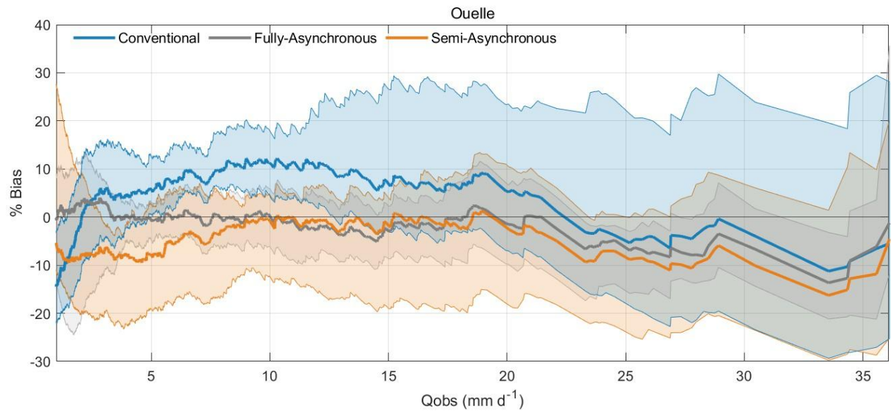
Figure C2. Same as Fig. C1, but for Ouelle catchment.
