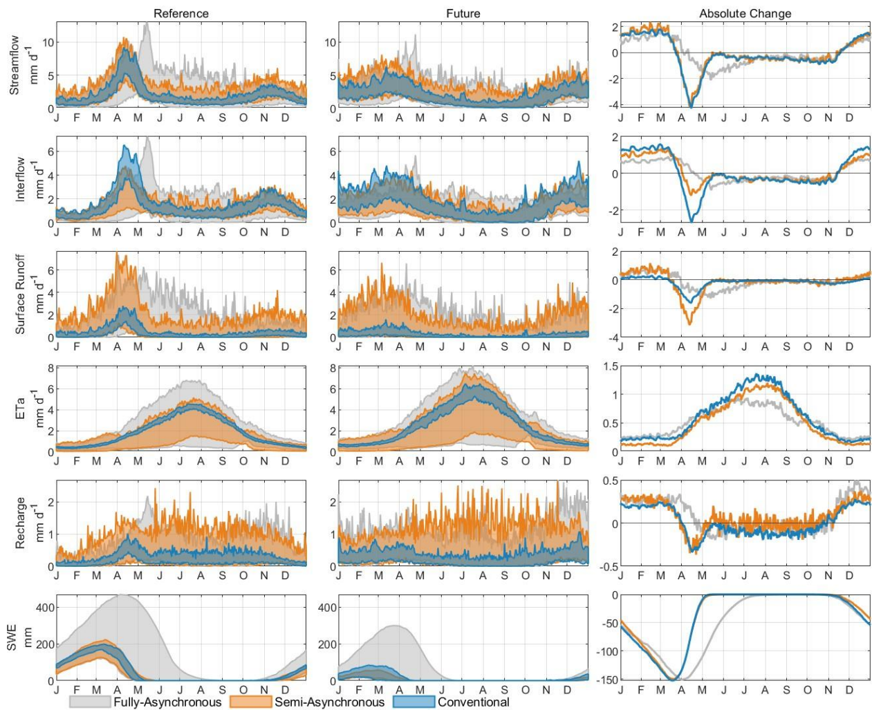
865 Figure F4E4. Same as F4E1 , but for Nicolet Sud-Ouest catchment.
