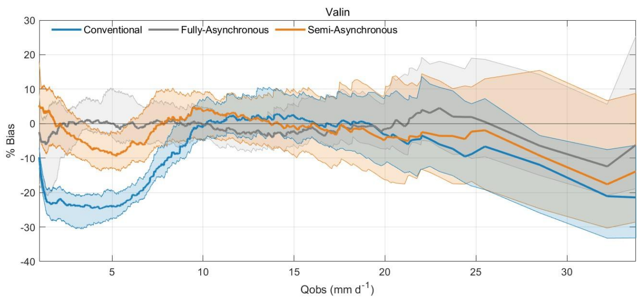
840 Figure C8. Same as Fig. C1, but for Valin catchment.
