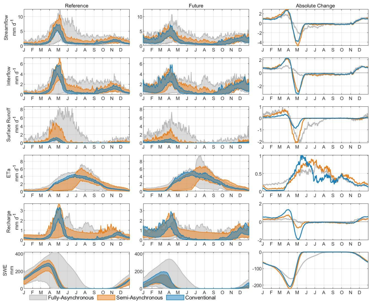
Figure F7E7. Same as F4E1, but for Du loup catchment.
