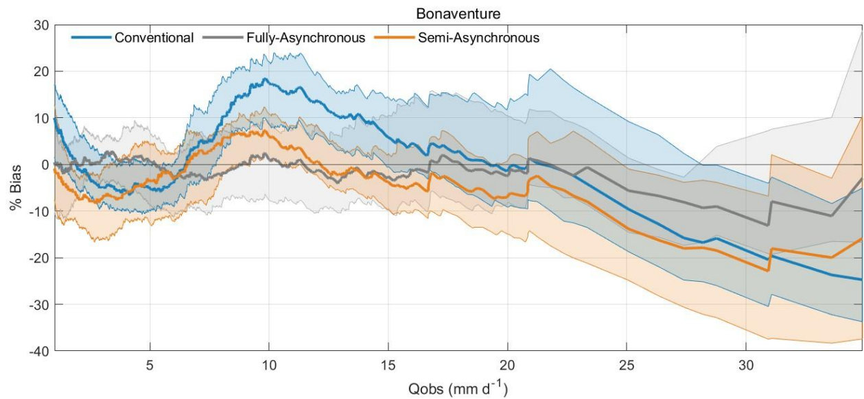
825 Figure C1. Performance comparison between the conventional, fully asynchronous and semi-asynchronous methods for the Bonaventure catchment during the reference period (1981–2010). The figure shows the percentage bias between observed and simulated streamflows, with the x-axis representing the observed daily streamflow and the y-axis displaying the percentage bias relative to the observed values. The shaded regions illustrate the variability among climate models around the mean bias for each method.
