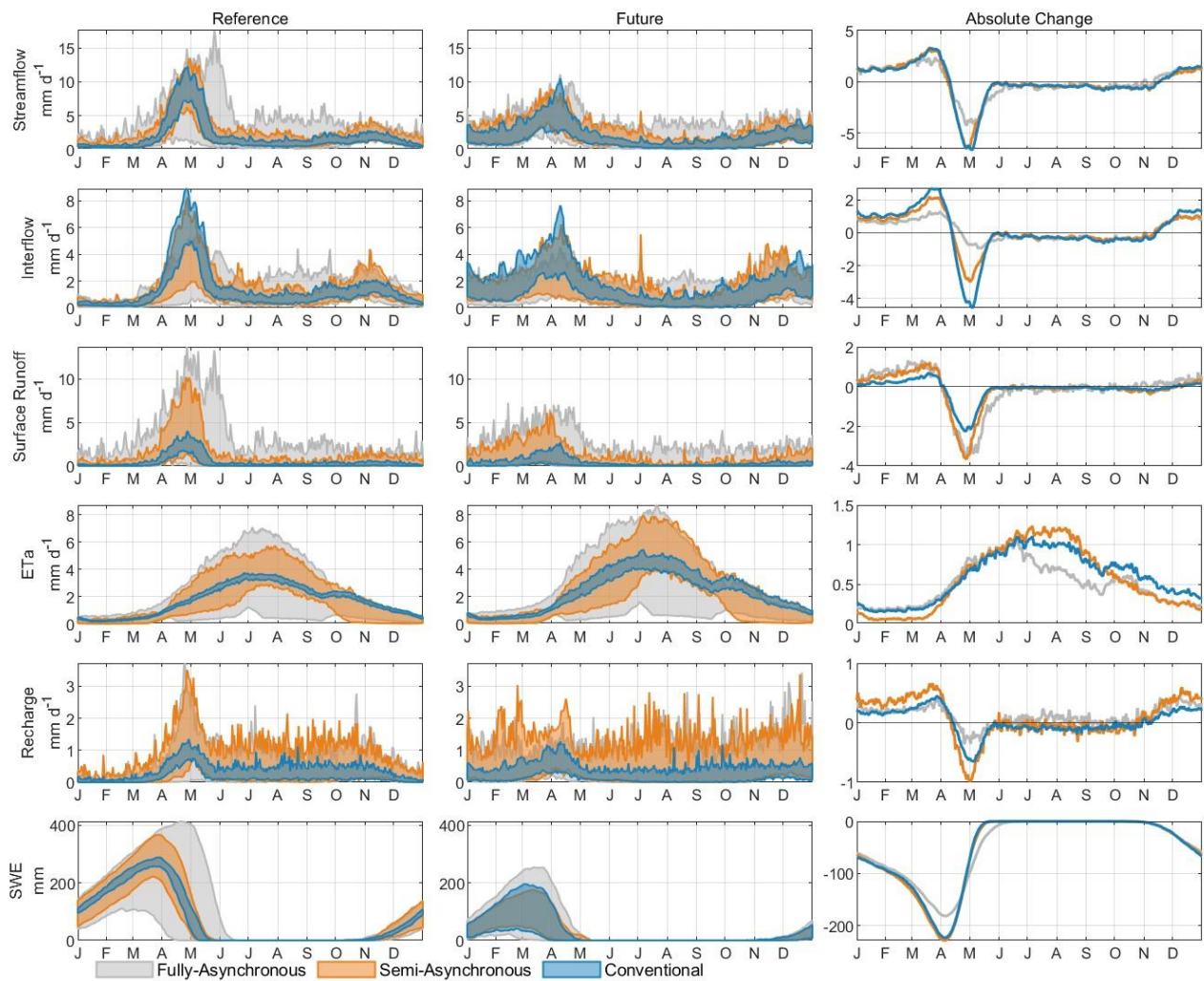
Figure EF2. Same as EF1, but for Ouelle catchment.
