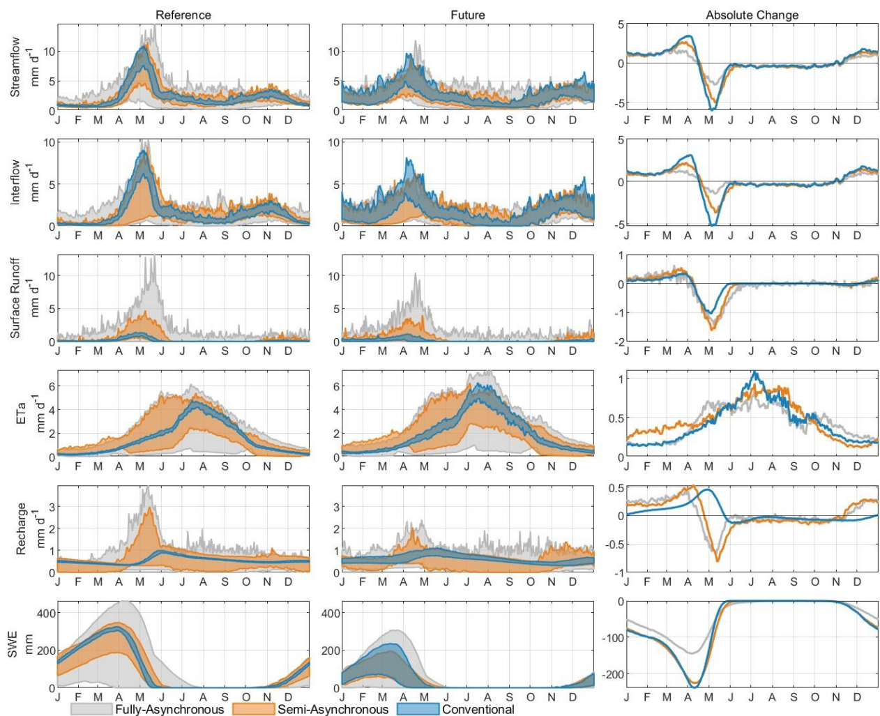
Figure F6E6. Same as F1E1E1, but for Bras du Nord catchment.
