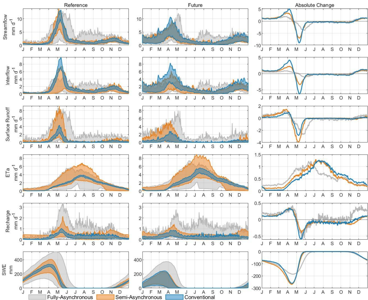
Figure 7. Seasonal distribution of key hydroclimatic variables for the reference period (1981–2010), future period (2070–2099), and their average absolute changes across the Matane catchment. The left column shows simulations during the reference period, the middle column corresponds to the future period, and the right column displays the absolute change between the two. Shaded areas represent the spread across the 18 climate models.
