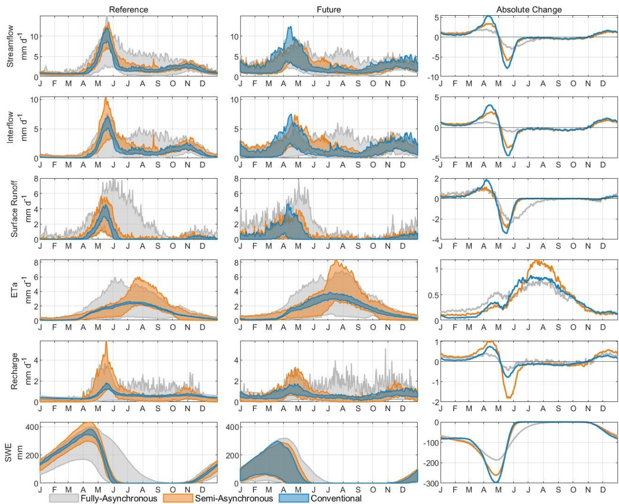
875 Figure F9E9. Same as F4E1 , but for Godbout catchment.
