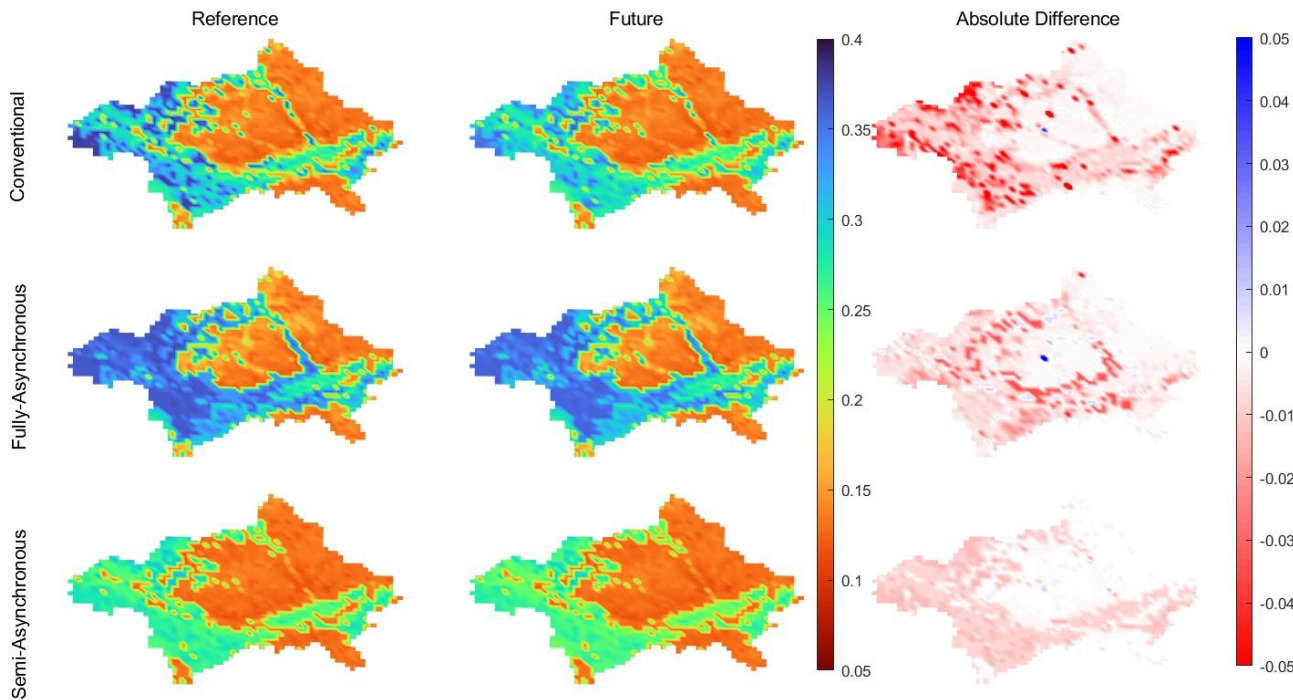
Figure 9. Spatial distribution of relative soil moisture in the Matane catchment for the reference period (1981–2010) and future period (2070–2099).
