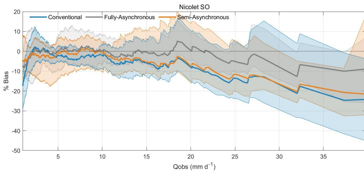
Figure C4. Same as Fig. C1, but for Nicolet Sud-Ouest catchment.
