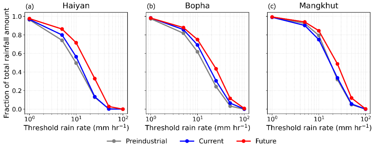
Figure 5. Fraction of total storm rainfall contributed by precipitation exceeding increasing rain-rate thresholds for (a) Haiyan, (b) Bopha, and (c) Mangkhut under pre-industrial (gray), current (blue), and future (red) climates. Future simulations shift rainfall contributions toward higher intensities, indicating increasing dominance of extreme precipitation events.
