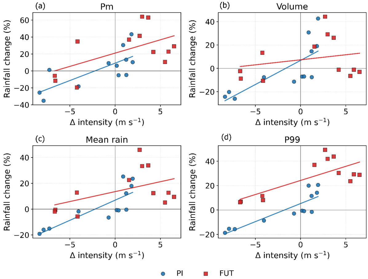
Figure 11. Relationship between changes in tropical cyclone intensity ( \Delta intensity, \text{m s}^{-1} ) and rainfall response for pre-industrial (PI; blue) and future (FUT; red) simulations. Panels show percent changes in (a) azimuthally averaged maximum rainfall rate (Pm), (b) rainfall volume, (c) mean rainfall rate, and (d) extreme rainfall (P99). Solid lines indicate linear fits for each climate state, highlighting a stronger and more consistent positive scaling between intensity and rainfall under future warming compared to pre-industrial conditions.
