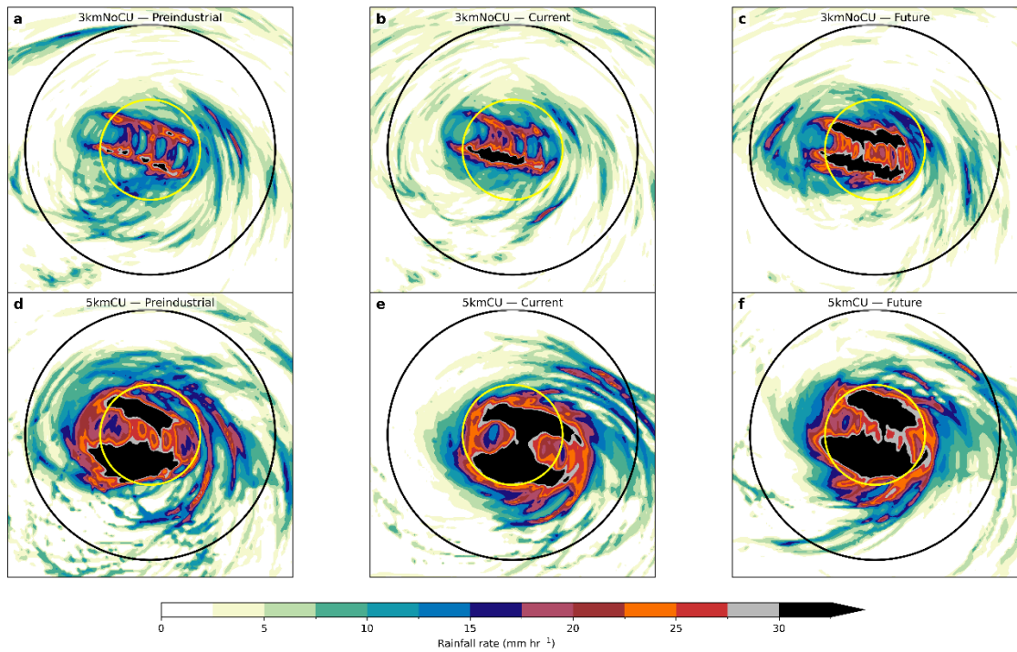
Figure 6. Simulated precipitation rate (mm/hr) at simulated peak intensity for Haiyan on 7 November 2013 12UTC for the 3kmNoCU runs (upper panel) and the 5kmCU runs (lower panel) under the pre-industrial (left), current (middle), and future climate conditions. The black circle indicates the 2.5° radius from the center, and the yellow circle indicates the 1° radius from the center.
