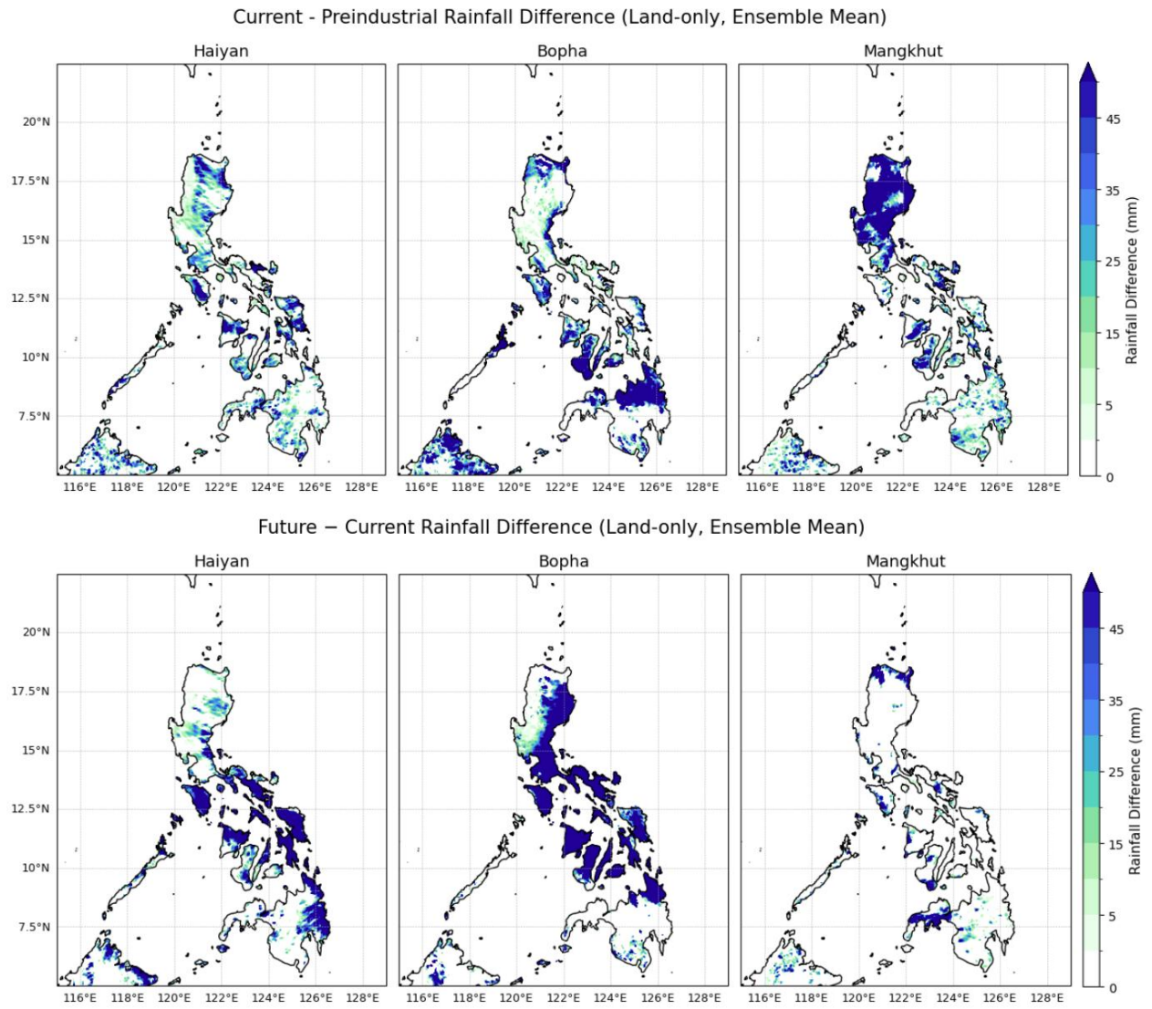
Figure 2. Difference in the ensemble-mean accumulated precipitation (a-c, top panels) Current minus Pre-industrial; (d-f, bottom panels) Future minus Current for Typhoons Haiyan (left), Bopha (middle) and Mangkhut (right) under the 3kmNoCU simulations.
