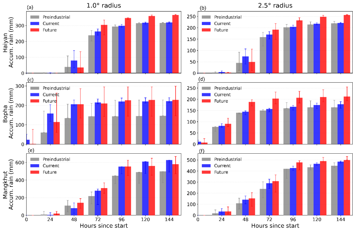
Figure 1. Total accumulated precipitation rainfall within 1.0° (left column) and 2.5° (right column) radii from the TC center for Typhoons Haiyan, Bopha, and Mangkhut under pre-industrial (gray), current (blue), and future (red) thermodynamic conditions.
