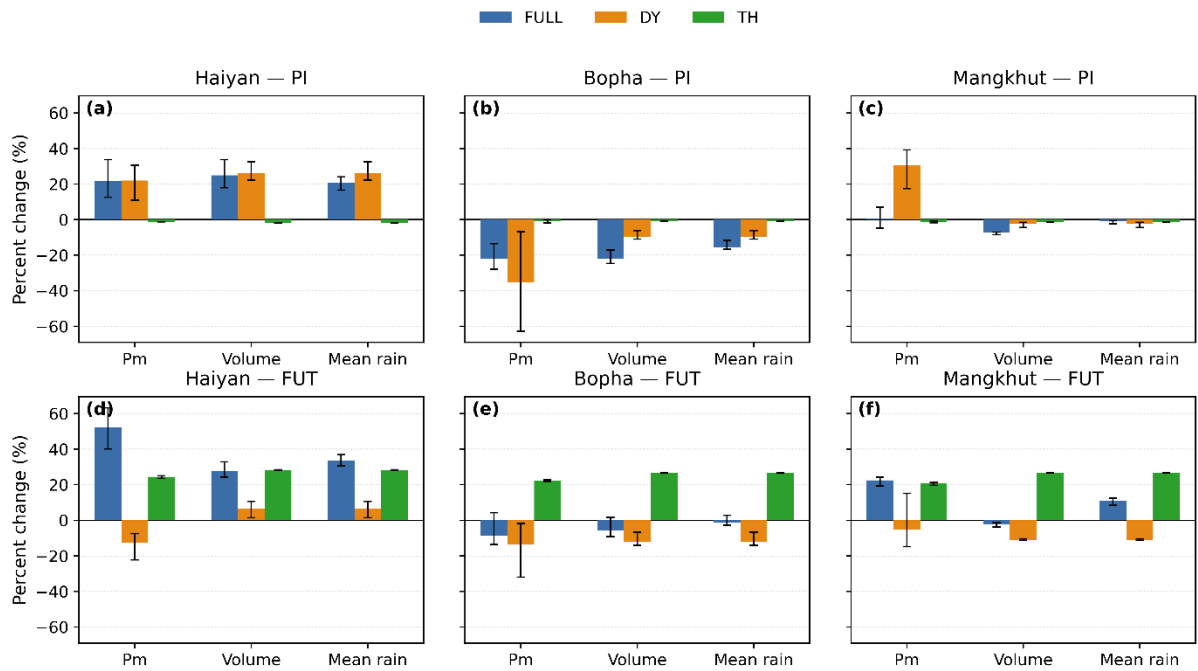
Figure 10. Decomposition of tropical cyclone rainfall changes into full (FULL), thermodynamic (TH), and dynamic (DY) contributions for Haiyan, Bopha, and Mangkhut, shown for pre-industrial (PI) and future (FUT) climates relative to present-day conditions. Bars indicate percent changes in azimuthally averaged maximum rainfall rate (Pm), rainfall volume, and mean rainfall rate within 500 km of the storm centre; error bars denote ensemble spread (IQR).
