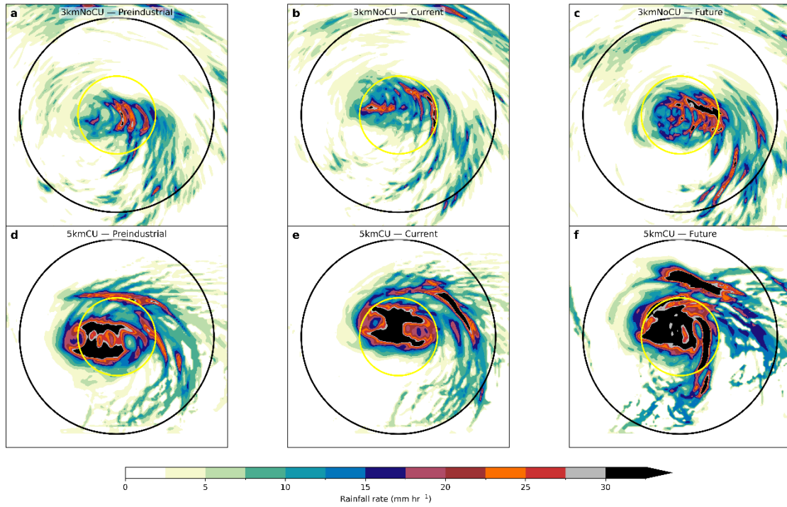
Figure 7. Same as Figure 6, but for Bopha
