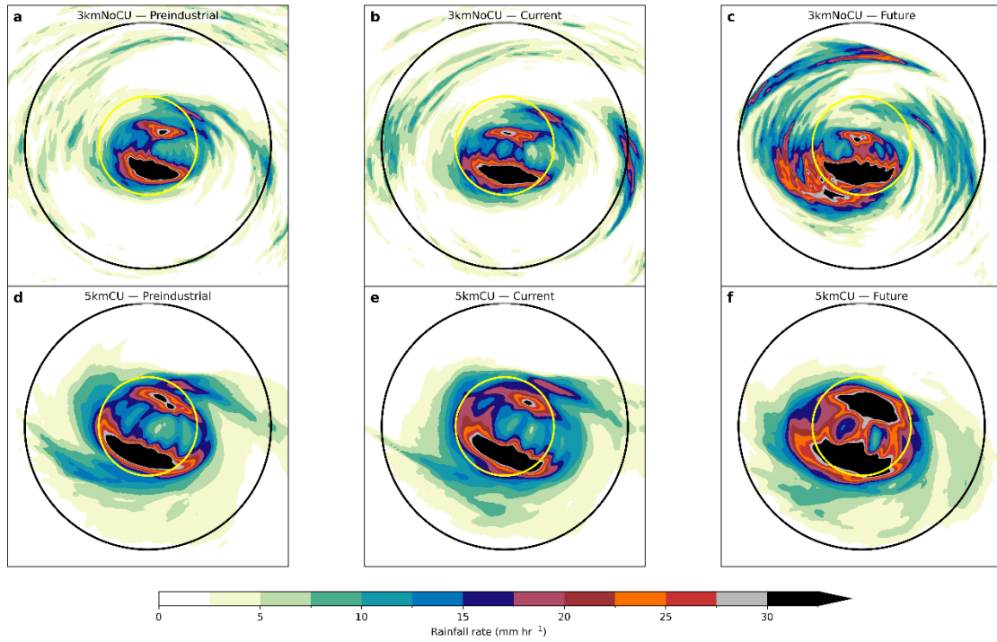
Figure 8. Same as Figure 6, but for Mangkhut
