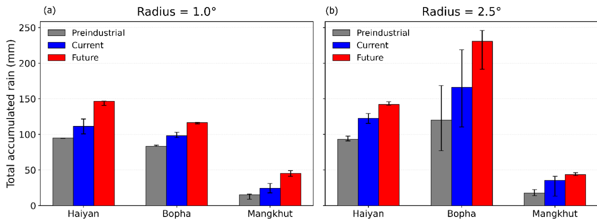
Figure 3. Boxplots for the Total Accumulated Rainfall within 1° and 2.5° radius of the center of the track from the preindustrial, current, and future climate scenarios for Typhoons Haiyan, Bopha, and Mangkhut under the 3kmNoCU simulations using all ensemble members. Error bars represent ensemble interquartile range.
