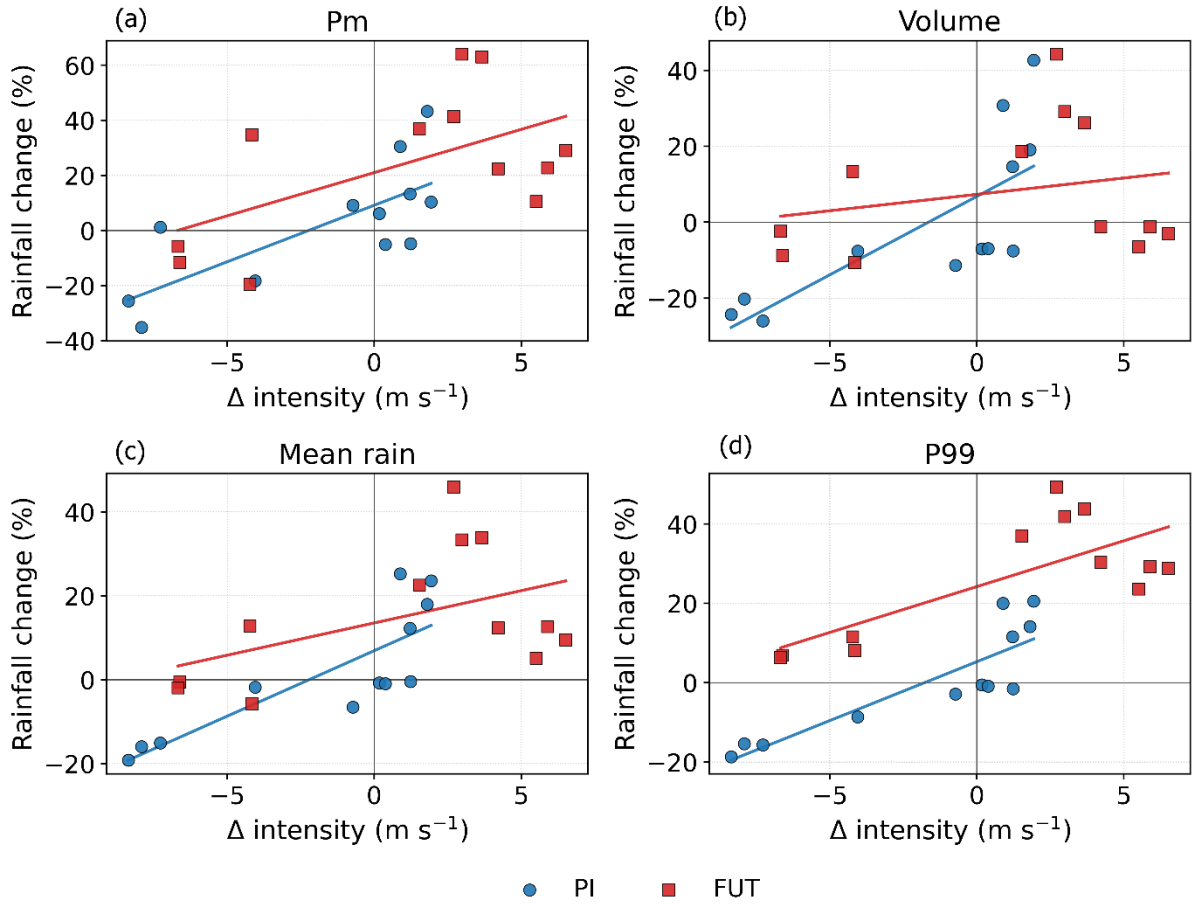
Figure 11. Relationship between changes in tropical cyclone intensity ( \Delta intensity, \text{m s}^{-1} ) and rainfall response for preindustrial (PI; blue) and future (FUT; red) simulations. Panels show percent changes in (a) azimuthally averaged maximum rainfall rate ( P_m ), (b) rainfall volume, (c) mean rainfall rate, and (d) extreme rainfall ( P_{99} ). Solid lines indicate linear fits for each climate state, highlighting a stronger and more consistent positive scaling between intensity and rainfall under future warming compared to preindustrial conditions.
