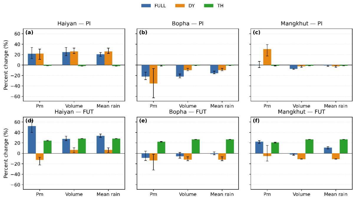
Figure 10. Decomposition of tropical cyclone rainfall changes into full (FULL), thermodynamic (TH), and dynamic (DY) contributions for Haiyan, Bopha, and Mangkhut, shown for preindustrial (PI) and future (FUT) climates relative to present-day conditions. Bars indicate percent changes in azimuthally averaged maximum rainfall rate (Pm), rainfall volume, and mean rainfall rate within 500 km of the storm centre; error bars denote ensemble spread (IQR).
