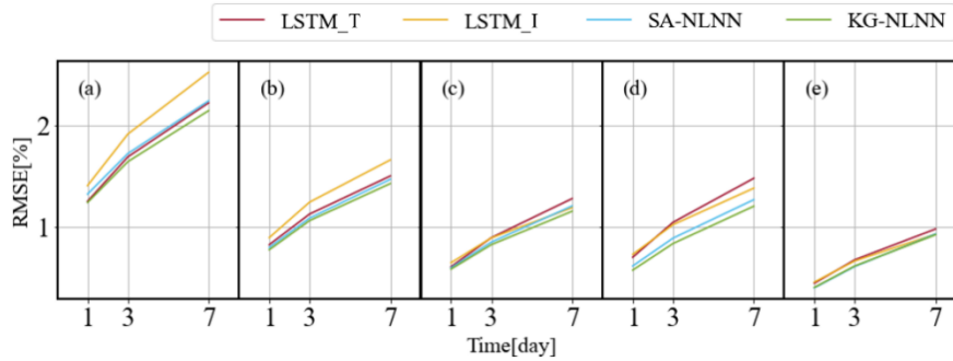
Figure 9. Comparison of mean RMSE for LSTM_T, LSTM_I, SA-NLNN, and KG-NLNN. The values are averaged across twenty research sites and presented separately for each of the five soil depths: 0.05m(a), 0.10m(b), 0.20m(c), 0.50m(d), 1.00m(e).
