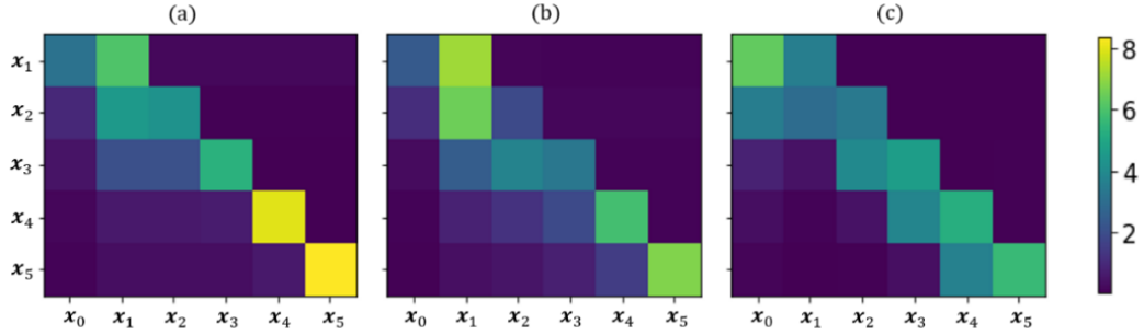
Figure 14. The non-local weight maps of the KG-NLNN model at different time scales at 0.2-day (a), 0.5-day (b), and 1.0-day (c) in the homogenous soil.
