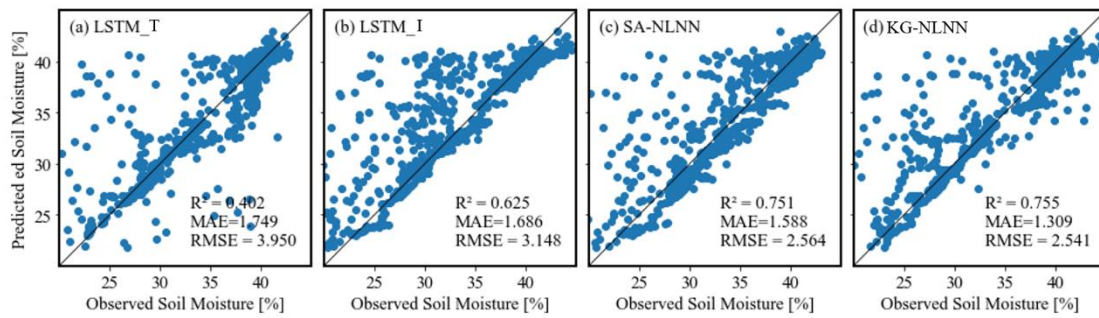
Figure 10. Scatter plots of the soil moisture observations and 7-day predictions generated from (a) LSTM_T, (b) LSTM_I, (c) SA-NLNN, and (d) KG-NLNN at UpperBethlehem.
