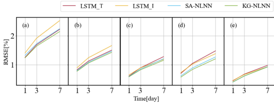
Figure 9. Comparison of mean RMSE for LSTM_T, LSTM_I, SA-NLNN, and KG-NLNN. The values are averaged across twenty research sites and presented separately for each of the five soil depths: 0.05m(a), 0.10m(b), 0.20m(c), 0.50m(d), 1.00m(e).
