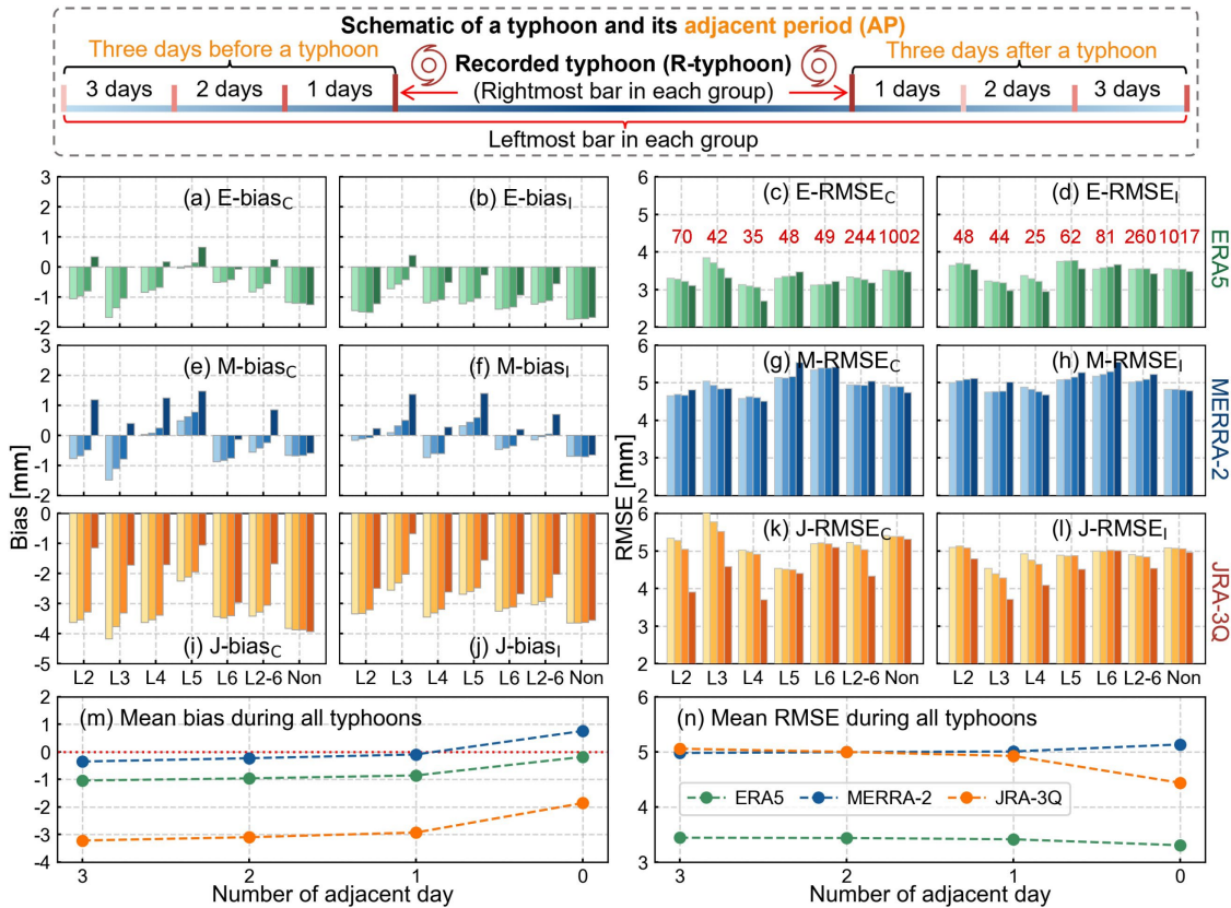
325 Figure 4. The top panel shows the schematic timeline of r-typhoon and the AP. Panels (a–l) present biases and RMSEs under different AP settings across typhoon categories (ERA5: a–d; MERRA-2: e–h; JRA-3Q: i–l). Within each bar cluster, color from light to dark correspond to AP±3, AP±2, AP±1 days, and r-typhoon, respectively. “L2–6” and “Non” denote the results for all typhoons and for non-typhoon periods, respectively. Panels (c) and (d) report the numbers of CMONOC and IGS station–typhoon pairs. Panels (m) and (n) summarize the mean bias and RMSE averaged over all typhoons as a function of AP.
