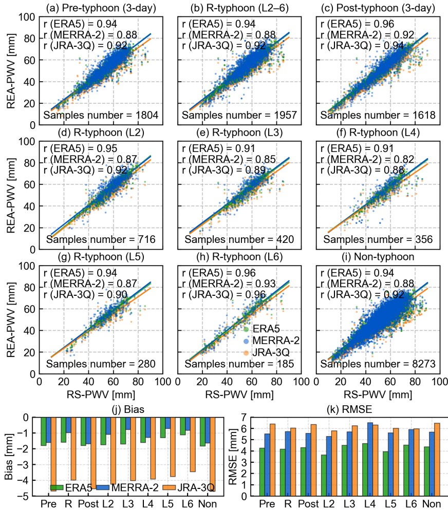
410 Figure 6. Correlation statistics of REA-PWVs and RS-PWVs for (a) pre-typhoon period (3 days before r-typhoon), (b) r-typhoon period, (c) post-typhoon period (3 days after r-typhoon), (d–h) r-typhoon periods for different categories, and (i) non-typhoon periods. Panels (j) and (k) summarize the corresponding REA-biases and REA-RMSEs for panels (a–i). Correlation coefficient ( r ) and the number of samples are shown in each panel (a–i).
