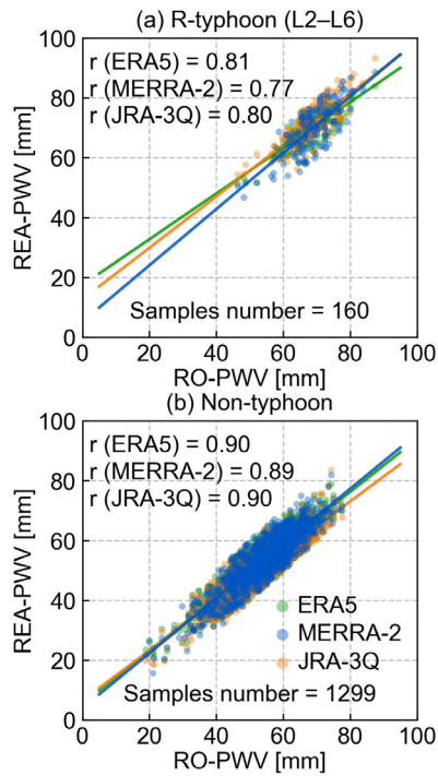
445 Figure 7. Correlation statistics of REA-PWVs and RO-PWVs for (a) r-typhoon and (b) non-typhoon periods. Correlation coefficients ( r ) and the number of samples are shown in each panel.
