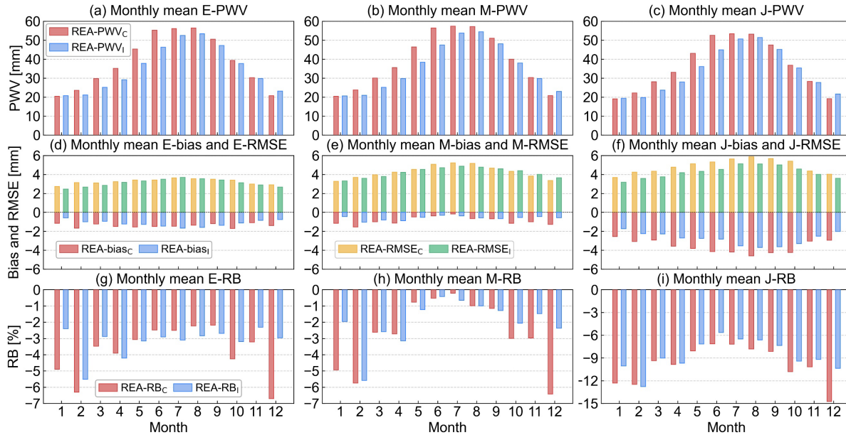
Figure 3. Monthly mean evaluation results. Panels (a-c) show REA-PWV (mm); red and blue bars denote REA-PWV sampled at the locations of CMONOC (REA-PWV C ) and IGS (REA-PWV I ) stations, respectively. Panels (d-f) show REA-bias and REA-RMSE (mm); red and yellow bars denote bias and RMSE at CMONOC stations (REA-bias C and REA-RMSE C ), respectively, and blue and green bars denote bias and RMSE at IGS stations (REA-bias I and REA-RMSE I ), respectively. Panels (g-i) show REA-RB (%); red and blue bars denote RB at CMONOC (REA-RB C ) and IGS (REA-RB I ) stations, respectively. Subscripts C and I indicate that reanalysis PWV is sampled at CMONOC and IGS station locations, respectively, and that the corresponding statistics (bias, RMSE, and RB) are computed against GNSS observations from the same network.
