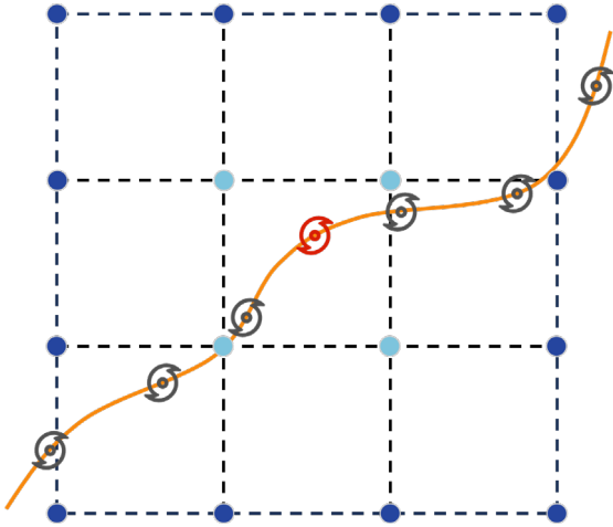
265 Figure 2. Schematic of NSD calculation. The orange line shows the typhoon track; the red marker indicates the typhoon center. The 16 nearest grid points are shown in dark blue and light blue, with the 4 closest points in light blue.
