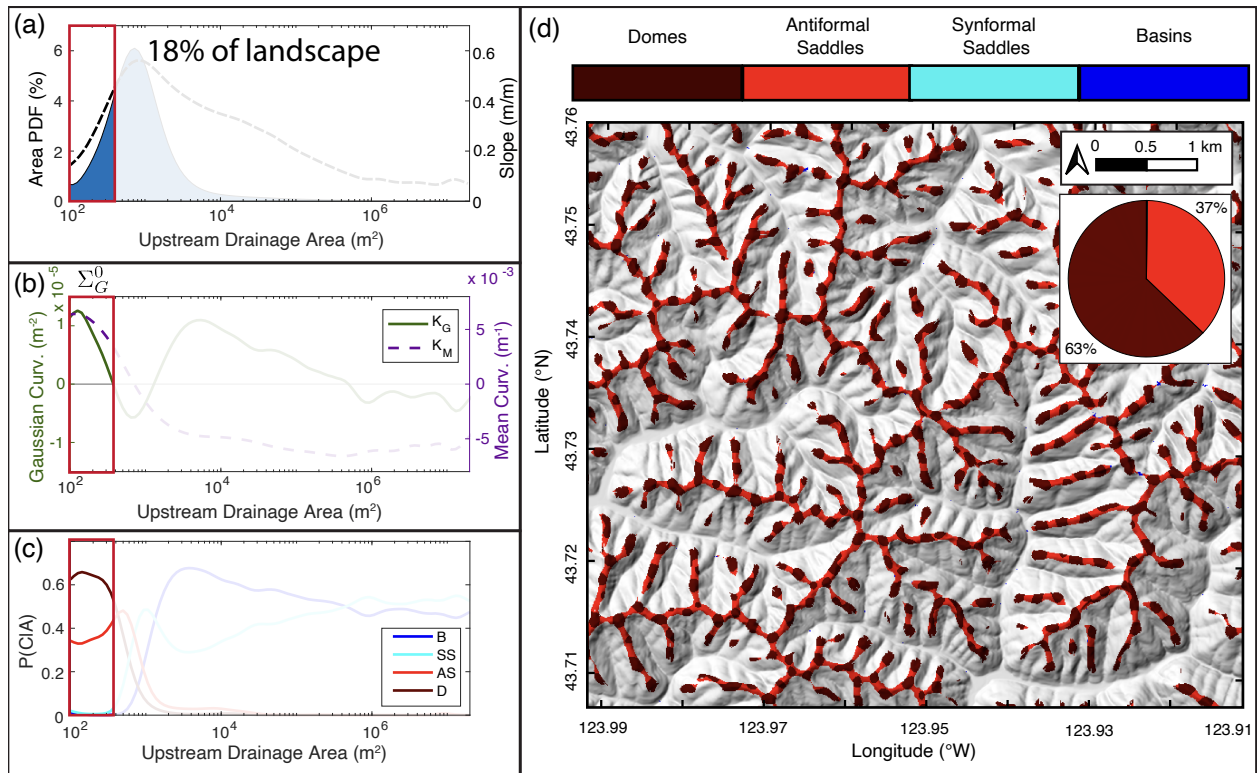
Figure 9. Surface geometry data for region \Sigma_G^0 : points in the landscape with upstream drainage areas less than 3.50 \times 10^2 3.75 \times 10^2 m 2 . The red box in each of the area-binned plots (a-c) highlights the range of included drainage areas. a) PDF of drainage areas. b) Gaussian and mean curvatures binned by area. c) Conditional PDFs of shape classes. d) Map of shape classes projected on a focused subregion of the study area. Pie-chart inset shows shape-class composition of the surface.
