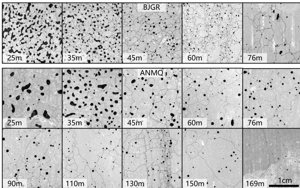
270 Figure A1. Exemplary microstructure images of BJGR and ANMQ ice cores; Microstructure images at different depths are selected, showing significant variations in grain area and bubbles.
