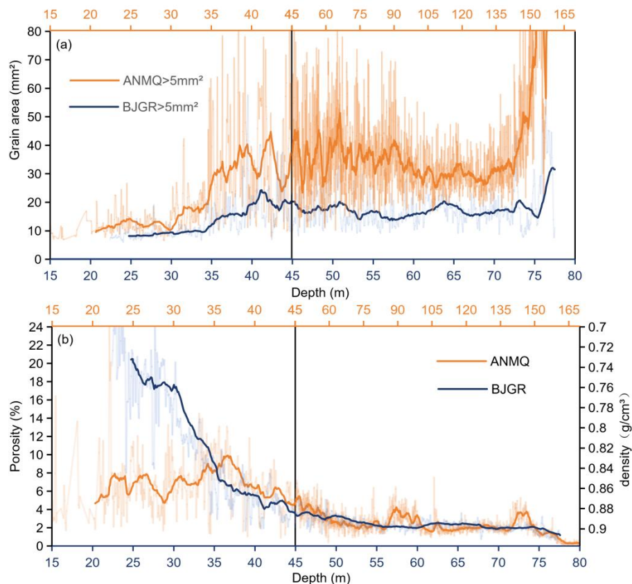
Figure A2. (a) Average area of grains > 5 mm² profiles of ANMQ and BJGR ice cores. The average area of all grains is significantly correlated with the average area of grains > 5 mm² (ANMQ: r_s = 0.847 , p_s < 0.01 ; BJGR: r_s = 0.909 , p_s < 0.01 ); (b) The porosity and slice density profiles of ANMQ and BJGR ice cores; The thin lines represent original data, the bold lines represent the 25 point smooth.
