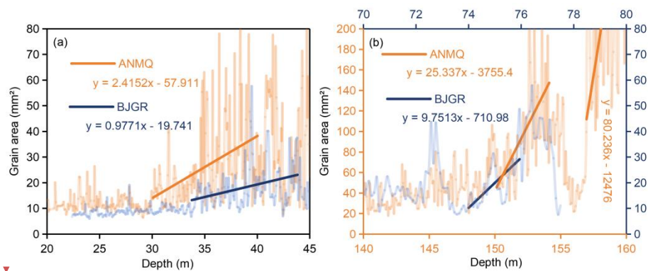
Figure A3. Growth rate of grains > 5 mm 2 : (a) Firn-ice transition layer; (b) SIBM layer; The thin lines represent 2 cm resolution data, the bold lines represent linear fitting results.
