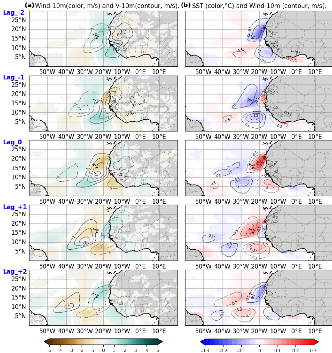
Figure 8: Lagged regression of atmospheric and oceanic variables onto the 2–10-day AEWs index, defined as the 10-m meridional wind anomaly at 23°W-11.5°N (with a positive index corresponding to a northward wind anomaly). Left panels show 10-m wind speed anomalies (color) and 10-m meridional wind anomalies (contours). Right panels show SST anomalies (color) and 10-m wind speed anomalies (contours). Regressions are presented at different time lags (in days) to capture the temporal evolution associated with AEWs passage. The AEWs index time series used here is illustrated in Figure 7.
