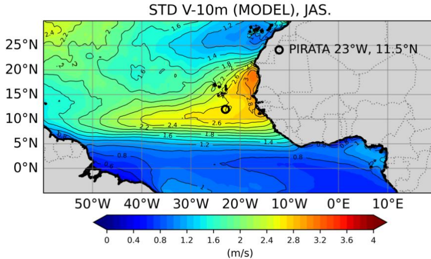
Figure 6: Standard deviation of the 10-m meridional wind anomalies (V-10m), band-pass filtered in the 2–10-day range, during the JAS period from 2001 to 2021 for the coupled model. The location of the PIRATA mooring at 23°W-11.5°N is indicated with a black circle. It lies within the area of maximum variability.
