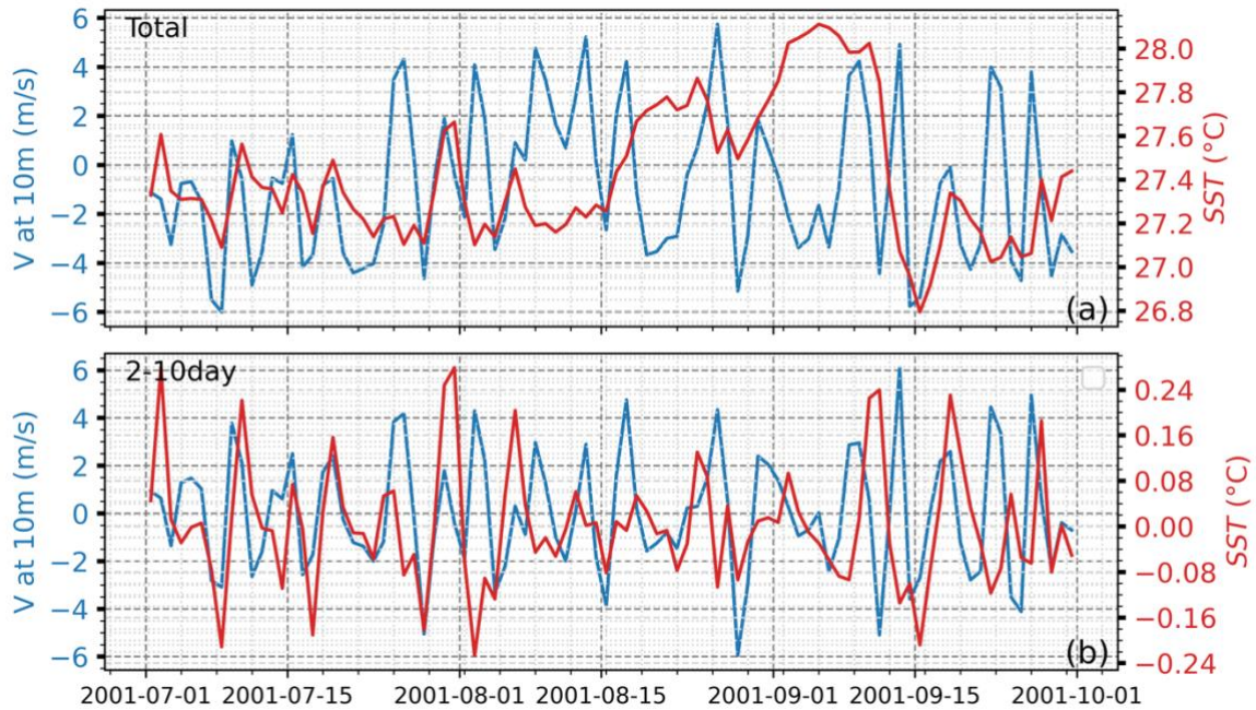
Figure 7: SST (in red) and 10-m meridional wind velocity (in blue) at 23°W-11.5°N during JAS 2001 for the coupled model: (a) non-filtered data, (b) band-pass filtered in the 2–10-day range.
