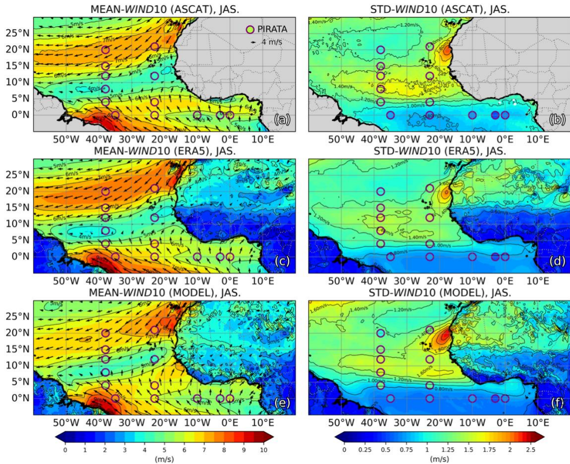
Figure 3: 10-m wind speed for the months of July-August-September (left panels) and corresponding standard deviation (right panels) over the 2007–2021 period for (a), (b) ASCAT, (c), (d) ERA5 and (e), (f) the coupled model. The standard deviation is computed from anomalies filtered in the 2–10-day band. In each panel, PIRATA mooring values are indicated by circles.
