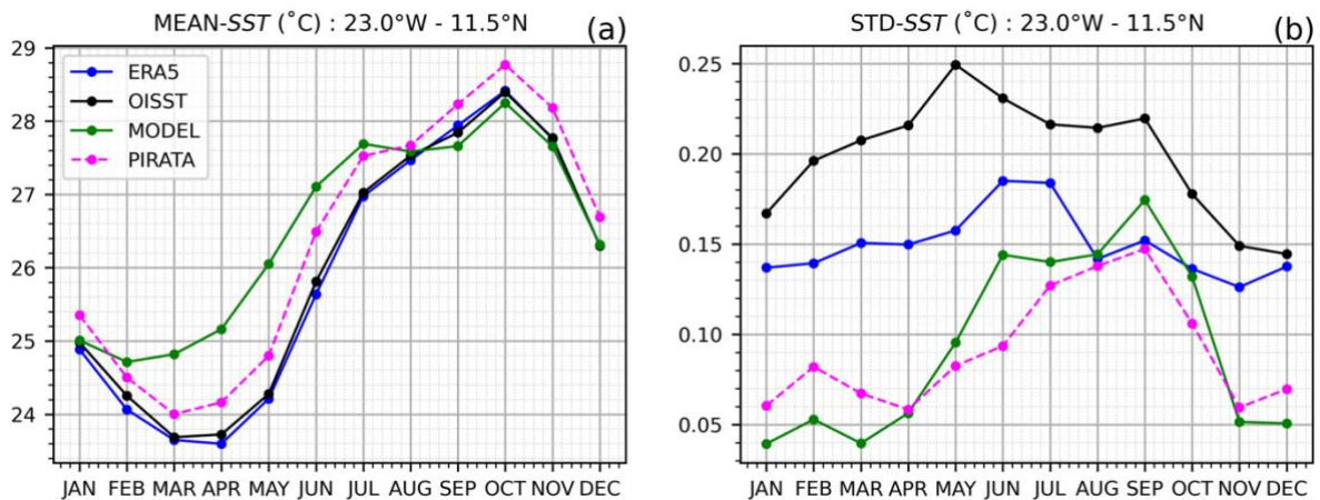
Figure 2: (a) Monthly climatology of SST, and (b) standard deviation of SST anomalies at 23°W–11.5°N over the 2007–2021 period of OISST (black), ERA5 (blue), the coupled model (green), and the 23°W-11.5°N PIRATA mooring (pink). Anomalies are band-pass filtered in the 2–10-day range prior to computing the standard deviation.
