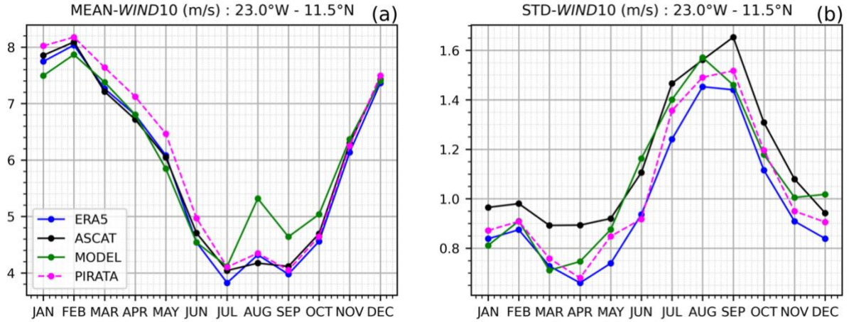
Figure 4: (a) Monthly climatology and (b) monthly standard deviation of the 10-m wind speed at 23°W–11.5°N over the 2007–2021 period for ASCAT (black), ERA5 (blue), the coupled model (green), and the 23°W-11.5°N PIRATA mooring. The standard deviation is computed from anomalies filtered in the 2–10-day band.
