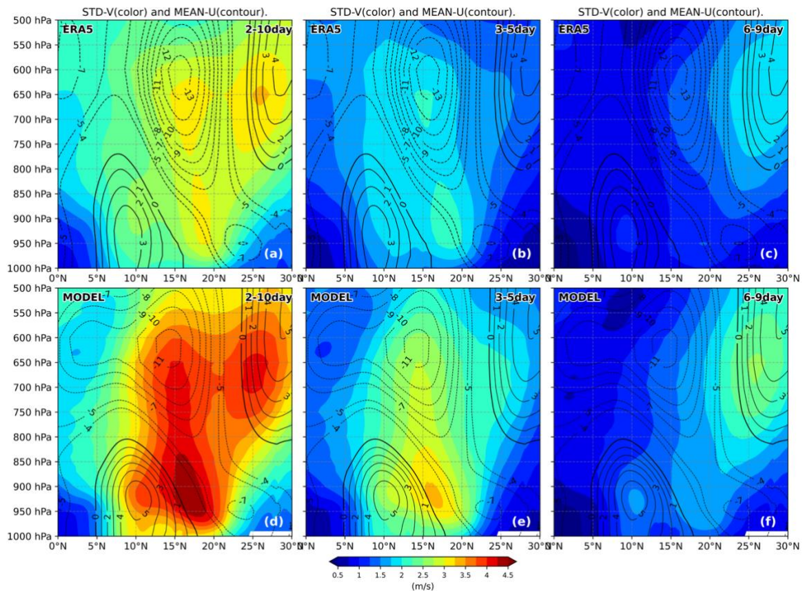
Figure 5: Latitudinal section of the standard deviation of meridional wind anomalies, longitudinally averaged between 25°W and 15°W, during JAS over the 2001–2021 period for (a), (b), (c) ERA5 and (d), (e), (f) the coupled model. Anomalies are band-pass filtered in the 2–10-day (left panels), 3–5-day (middle
