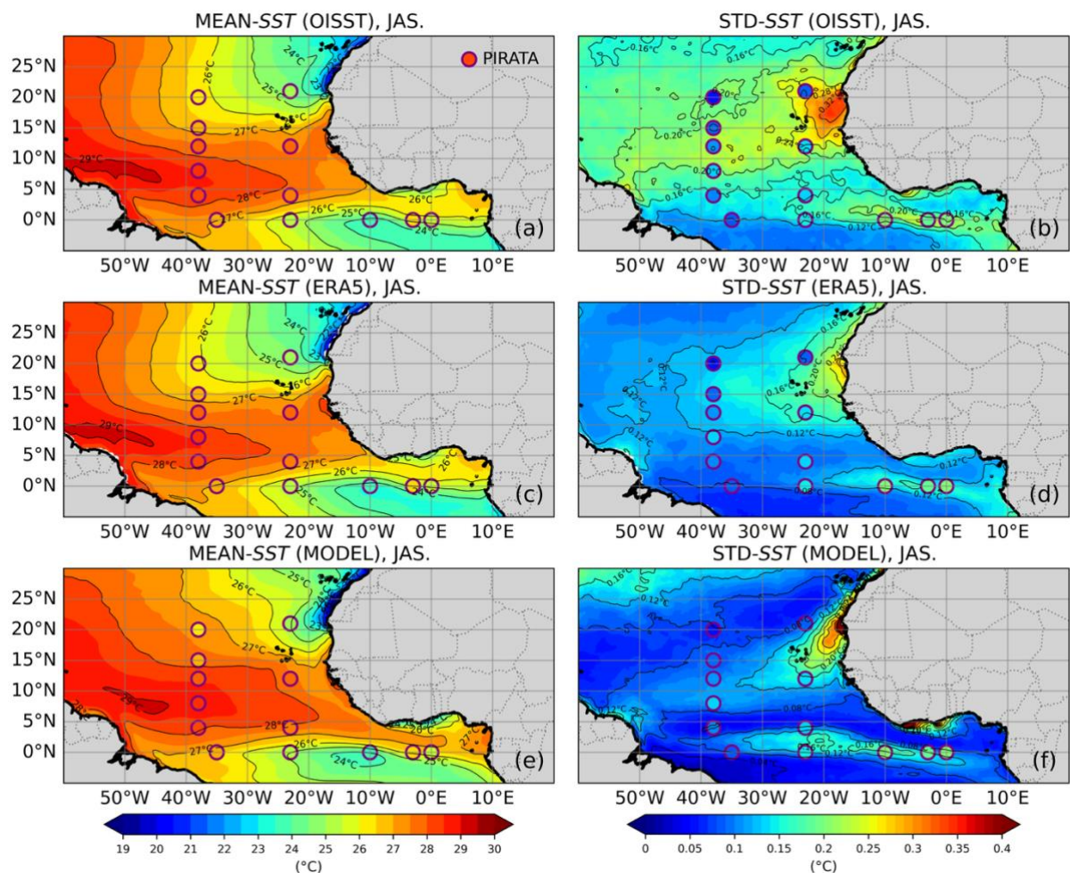
Figure 1: (Left panels) Mean SST, and (right panels) standard deviation of SST anomalies for July–August–September (JAS) over the 2007–2021 period, from (a), (b) OISST, (c), (d) ERA5, and (e), (f) the coupled model. The standard deviation is computed from anomalies band-pass filtered in the 2–10-day range. In each panel, estimates from the PIRATA mooring are indicated by circles.
