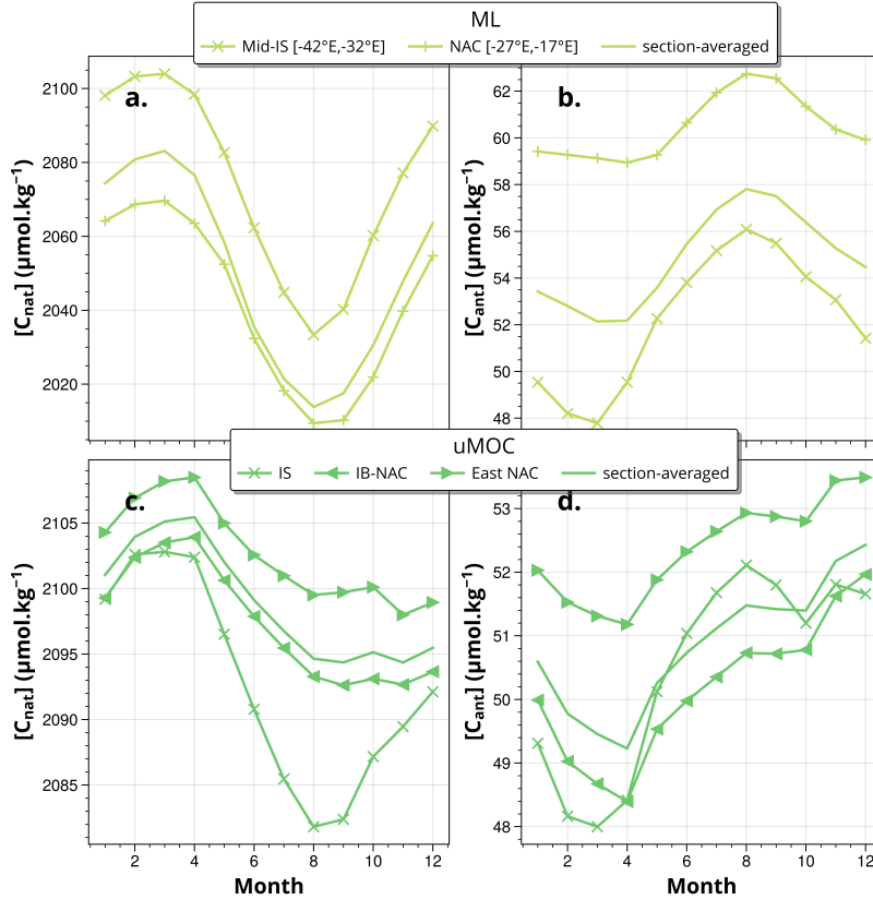
Figure 4. Seasonality of (a) ML [C_{nat}] and (b) ML [C_{ant}] for the full section (continuous color line), the center of Irminger Sea (between -42^{\circ}\text{E} and -32^{\circ}\text{E} , line with x markers) and the NAC (between -27^{\circ}\text{E} and -17^{\circ}\text{E} , line with + markers). Seasonality of (c) uMOC [C_{nat}] and (d) uMOC [C_{ant}] for the full section (continuous color line), the Irminger Sea (line with x markers), the Iceland Basin-NAC region (IB-NAC) (line with ◀ markers) and the East of the NAC (line with ▶ markers). The seasonal cycles are obtained by grouping the time series data by month and averaging over all ocean reanalyses. The time series are subsets of the complete series of Fig. 2, sampled from 2004 to 2017, so that each reanalysis has the same weight in the construction of the seasonality (Table 1).
