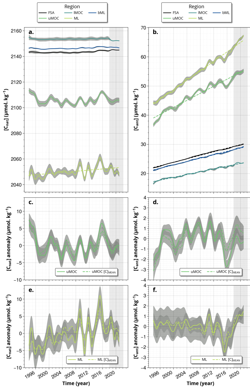
Figure 5. Low pass filtered signal (continuous lines) with their linear trends (dashed lines, plotted when significant at the 90 percent significance level) of (a) [C_{nat}] and (b) [C_{ant}] in the layers of interest uMOC, IMOC, ML and bML based on time series reported in Fig. 2. Full section average (FSA) concentration is in black. For the uMOC (c,d) and (e,f) ML, the signal is plotted in an anomaly along with the corresponding signal for a mean concentration [C]_{MEAN} . For [C_{ant}] , the linear trends have been removed in the anomaly plots. Grey shading indicates when only GLOSEA5 reanalysis is available. STDns ( \pm ) are shown in grey shading. Linear fit ( \pm confidence interval at 90%) on interannual [C_{nat}] : 0.22 \pm 0.04 \mu\text{mol kg}^{-1} \text{yr}^{-1} (ML). Linear fit values on interannual [C_{ant}] : 0.8 \pm 0.008 \mu\text{mol kg}^{-1} \text{yr}^{-1} (ML), 0.3 \pm 0.002 \mu\text{mol kg}^{-1} \text{yr}^{-1} (bML), 0.6 \pm 0.012 \mu\text{mol kg}^{-1} \text{yr}^{-1} (uMOC), 0.3 \pm 0.002 \mu\text{mol kg}^{-1} \text{yr}^{-1} (IMOC) and 0.3 \pm 0.001 \mu\text{mol kg}^{-1} \text{yr}^{-1} (FSA).
