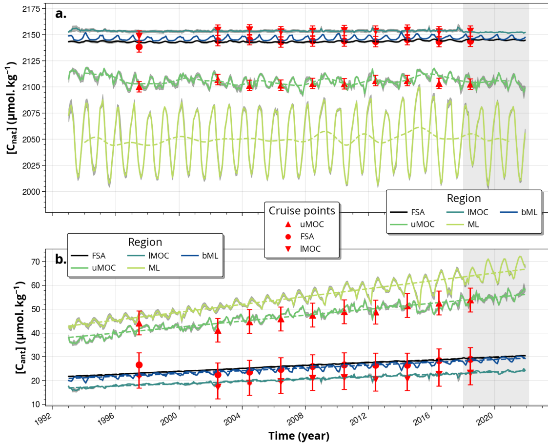
Figure 2. Area mean time series of (a) [C_{nat}] and (b) [C_{ant}] in all the layers of interest: the upper and lower branches of the Atlantic Meridional Overturning Circulation (uMOC in green, and lMOC in dark green, respectively), Mixed Layer (ML) in yellow green, and below the ML (bML) in dark blue. The full section averaged concentration (referred to as FSA) is shown in black. For the uMOC and ML layers, the concentration values were computed as the mean of the estimates from GLOSEA5, ECCO, CORA, EN4 and GOBAI-O 2 (Table 2). For the net, lMOC, and bML layers, the concentration values represent the average of the estimates derived from GLOSEA5, ECCO and EN4. The gray shading along the lines represents the standard deviation of all product estimates used in the monthly averaging, divided by the square root of the number of reanalysis. The dashed lines for C_{nat} (top) represent a low-pass filter time series (cutoff frequency of 24 months). For C_{ant} (bottom), dashed lines indicate the linear trend. The A25 cruise [C_{nat}] and [C_{ant}] estimates for uMOC, lMOC, and net are shown in red, with red vertical lines denoting the error bars (see methods). The grey shading at the end of the time series highlights the period for which only the GLOSEA5 reanalysis is available.
