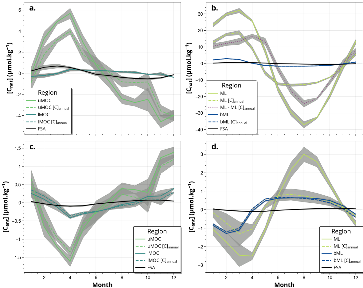
Figure 3. (a,b) Natural carbon [C_{nat}] and (c,d) anthropogenic carbon [C_{ant}] seasonal anomalies. Left (a,c) and right (b,d) panels show respectively uMOC/IMOC and ML/bML (Fig. 1, Table 2). Black lines represent the full section-average (referred to as FSA in the legend), light colors are used for the layers the closest to the sea surface (uMOC or ML), and dark colors account for the deeper layers (IMOC or bML). Each monthly value represents the mean value calculated from the ensemble of ocean reanalyses, and the shaded areas the standard errors. The dashed lines represent the idealized seasonal anomaly computed using annual mean property fields and only taking into account changes in area surfaces of layers (see 2.7 for details). The difference between the seasonal cycle of [C_{nat}] in the ML and its idealized anomaly, attributed to biological activity, is shown in purple (b).
