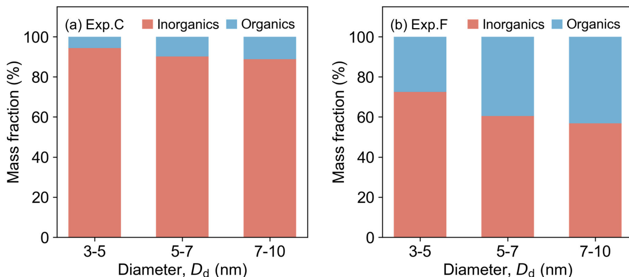
Figure 4. Organic mass fraction of SA-OOMs mixtures as a function of particles diameter range with two precursors mixing ratios: (a) 0.1 for Exp. C, (b) 1 for Exp. F. Red and blue bars represent f_{\text{org}} values of inorganics (SA) and organics (OOMs). Note that the size ranges are defined as semi-open intervals, except for the first bin which includes its lower bound.
