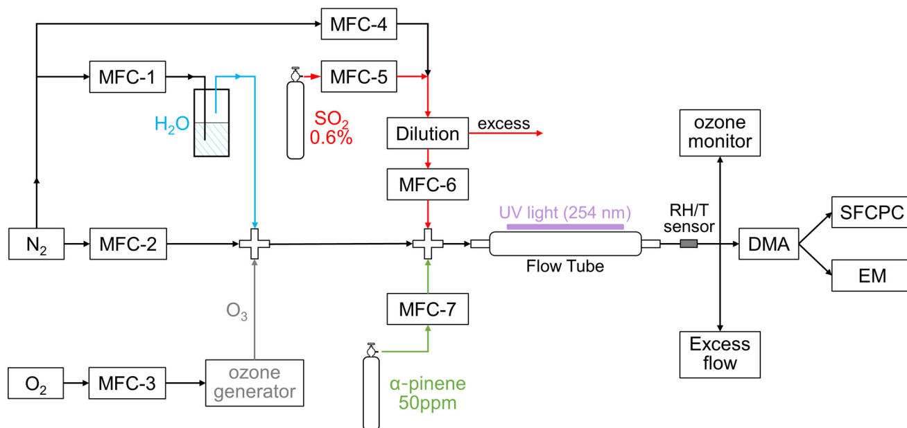
90 Figure 1. Schematic of the flow tube reactor and experimental setup. Precursors (SO 2 , \alpha -pinene, O 3 and H 2 O) were introduced into the flow tube at a total flow rate of \sim 3 L min -1 . SO 2 and \alpha -pinene were subsequently oxidized by O 3 under UV irradiation (254 nm). The resulting oxidation products were classified using a nano-DMA, with particle hygroscopicity and chemical composition-organic content characterized by SFCPC and EM.
