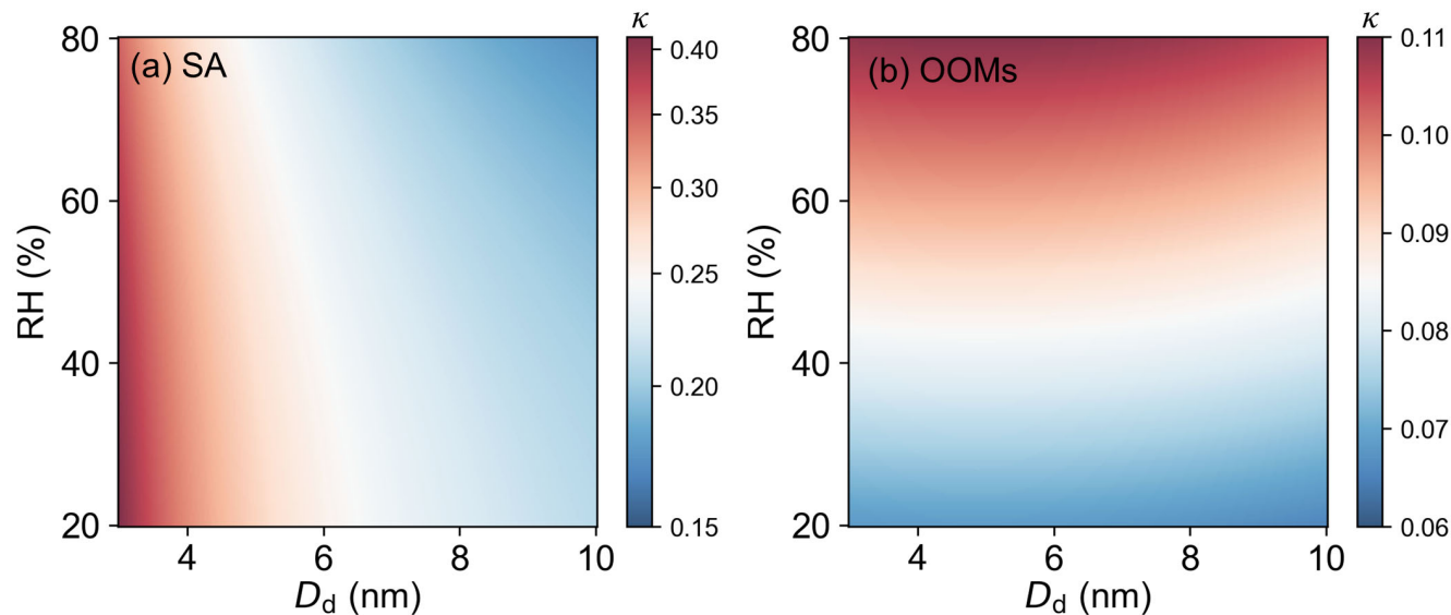
215 Figure 2. Dependence of hygroscopicity on particle size and RH: (a) SA formed from \text{SO}_2 , and (b) OOMs from \alpha -pinene oxidation. Color scale represents the \kappa values derived from f_{\text{org}} measurements using SFCPC and EM, where the values were fitted from measurement data to illustrate \kappa variation trend more clearly.
