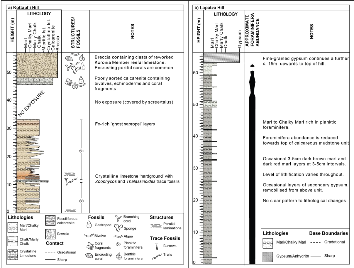
Figure 3 Simplified stratigraphic logs of the Kottaphi Hill succession (a) showing the occurrence of sedimentary structures and fossils up the section and the Lapatza Hill succession (b) showing the approximate abundance of planktic foraminifera and the main lithological changes up the succession.
