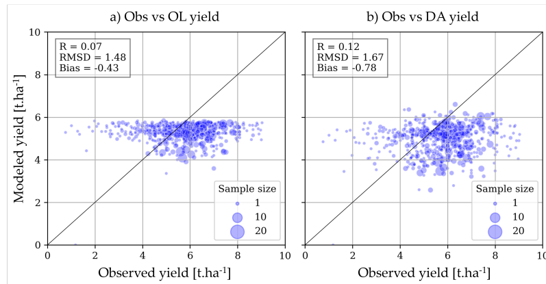
Figure 10. Spatiotemporal performance of the OL and DA simulations for end-of-season yield against in situ data, across all municipalities and years with winter wheat in 2017-2023. The dot size refers to the number of individual fields that contribute to the municipality average, for each observed yearly yield estimate.
