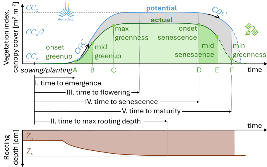
Figure 3. Crop stages assumed in (black I-V) AquaCrop, with an indication of some other (blue) essential AquaCrop crop parameters that define the CC_{pot} and rooting depth evolution. The timing of the crop stages can be inferred from (blue A-F) the time of the various satellite-based phenology stages in the GLSP product. Note the difference in the assumed shape of the curve for (blue) AquaCrop potential vegetation and (dashed green) GLSP actual vegetation during senescence.
