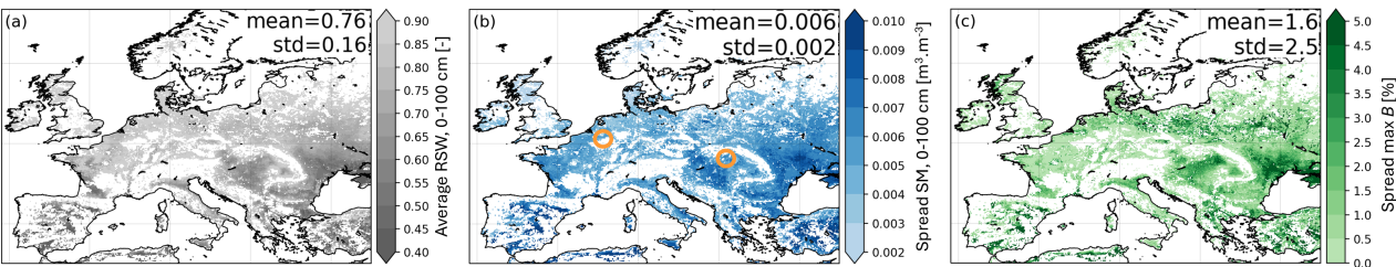
Figure 6. Multi-year averages of (a) relative root-zone soil water content (RSW), (b) ensemble spread in root-zone soil moisture (SM), and (c) ensemble spread in end-of-season (max) B , for 2015-2018. The centers of the circles in panel (b) mark the locations for Figure 7.
