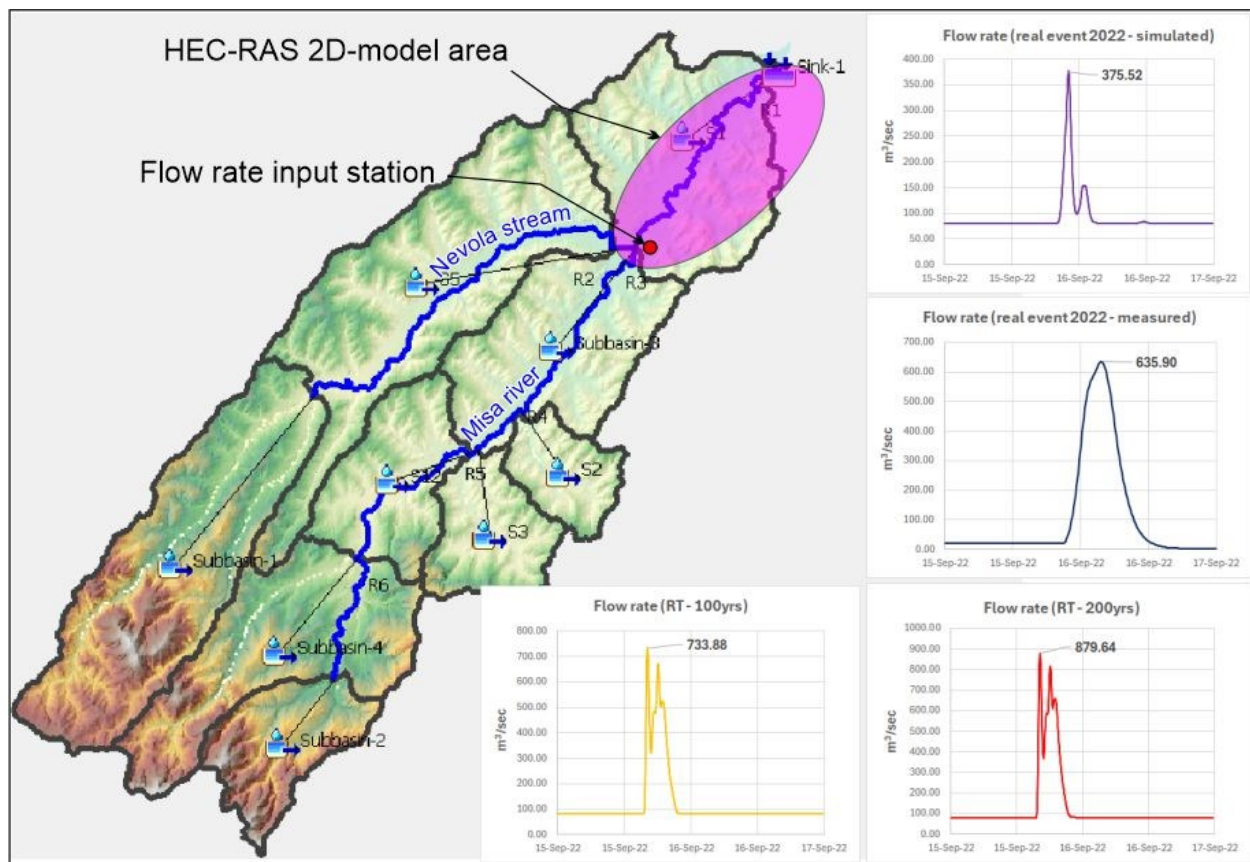
Fig. 12: HEC-HMS model results.
