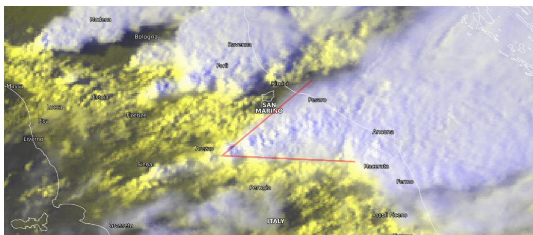
Figure 3: The Central Italy satellite view of the thunderstorm at 3:00 pm UTC on 15th September 2022. MSG-SEVIRI HRV cloud composite with the characteristic and well-recognisable V-shape (drawn in red). Copyright Eumetsat. Image from https://view.eumetsat.int/productviewer?v=61314 (last access 10.18.2024).
