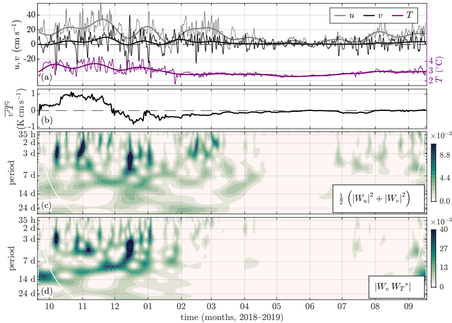
Figure 3. Time series of a) along-slope and across-slope current velocity u , v (left axis), and temperature T (right axis, purple) measured at 250 m depth at the western mooring W2 (a level in the core which consistently has both temperature and velocity measurements), low-passed filtered at 35 hours (thin curves) and 30 days (thick curves). Corresponding b) offshore eddy temperature flux \overline{v'T'} (positive for warm anomalies towards deeper water and cold anomalies towards shallower water), c) wavelet power spectrum, \frac{1}{2} (|W_u|^2 + |W_v|^2) , and d) wavelet cross-spectrum |W_v W_T^*| between v and T . The cone of influence (solid white curve) in (c, d) indicates the areas affected by boundary effects.
