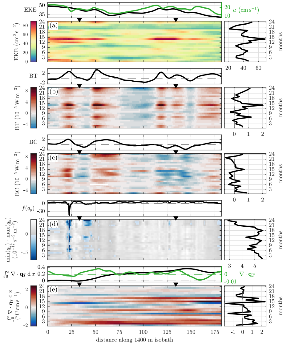
Figure 7. Spatio-temporal evolution along the 1400 m isobath of modelled a) EKE, b) BT, c) BC, and d) f(q_y) \equiv \min(q_y) \cdot \max(q_y) (negative values indicate a measure of cross-isobath sign-change change of sign of the lateral PV gradient -q_y . Temporal averaging is 1 month and the spatial smoothing is 20 km across the isobath) e) cumulative along-isobath integral of eddy temperature flux divergence, \int_0^x \nabla \cdot \mathbf{q}_T dx , where \mathbf{q}_T = (\overline{u'T'}, \overline{v'T'}) . Each group of panels include the spatio-temporal field (colours), its time-average (top), and its along-isobath average (right), except in panel e) where the panel on the right shows the product of along-isobath integral evaluated at the minimum and maximum end of q_y calculated across the isobath, ca. 180 km. In addition, time-averaged \bar{u} (negative values are indicative of a change in sign). Line plots in horizontal panels are time averages and those in vertical panels (e) are shown (green, top panel on the right are along-isobath averages axes). Temporal averaging is 1 month and the spatial smoothing is 20 km. October corresponds to months 1 and 13, April to months 7 and 19. Triangles mark approximate locations of the virtual moorings. Distance-axis tick labels intervals every 25 km correspond to the dots on the 1400 m isobath in Fig. 6. All variables are layer-averaged between 100 m and 2000 m or the seabed, except \nabla \cdot \mathbf{q}_T which is between 100 m and 500 m.
