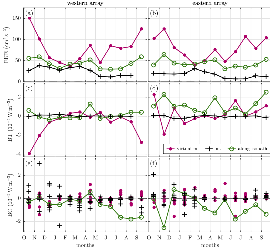
Figure 8. Time series of (a, eb ) EKE, ( bc , ed ) BT, and ( ee , f) BC from in situ moorings (black pluses), from the model using virtual moorings (purple dots), and the average along the 1400 m isobath near moorings (green open circles). The first-two model year-is-shown-in-dark , and the-second-year-in-pale-colours years were averaged together. In ( ee , f), BC are shown for the same levels as the moorings (Fig. 5), and-pale-purple-dots . The in situ mooring time series are offset by five days for clarity as in Figs. 4, 5 but monthly averaged.
