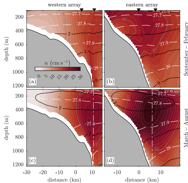
Figure B1. Average simulated along-slope current velocity u (colours) at (a, c) the western and (b, d) eastern mooring arrays during (a, b) autumn and winter (September–February) and (c, d) spring and summer (March–August) averaged over the two-year period. Grey contours show velocity every 10 \text{ cm s}^{-1} , white dashed isopycnals every 0.1 \text{ kg m}^{-3} , and black isotherms every 1^\circ\text{C} . Triangles at the top mark the virtual mooring locations (a, b) and vertical white dash-dotted lines mark the location of the 1400 m isobath used in Section 3.3.2.
