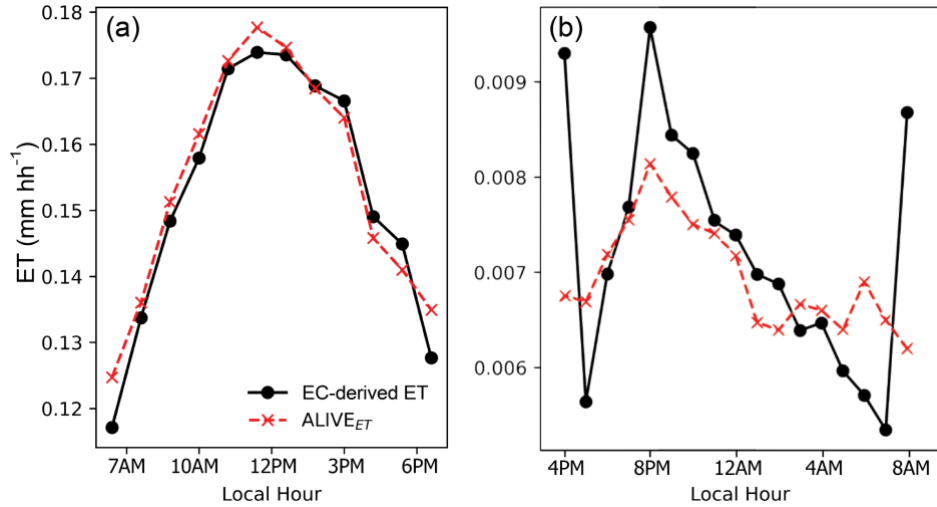
Figure 3. Mean values of EC-derived ET ( \text{mm hh}^{-1} ) (a) vs. daytime \text{ALIVE}_{\text{ET}} estimated from GBR trained on single time observations and (b) nighttime \text{ALIVE}_{\text{ET}} estimated from LSTM trained on time series observations. Values are hourly averages derived from 30-minute data and are averaged across all sites for each local solar hour, with daytime and nighttime defined based on SZA.
