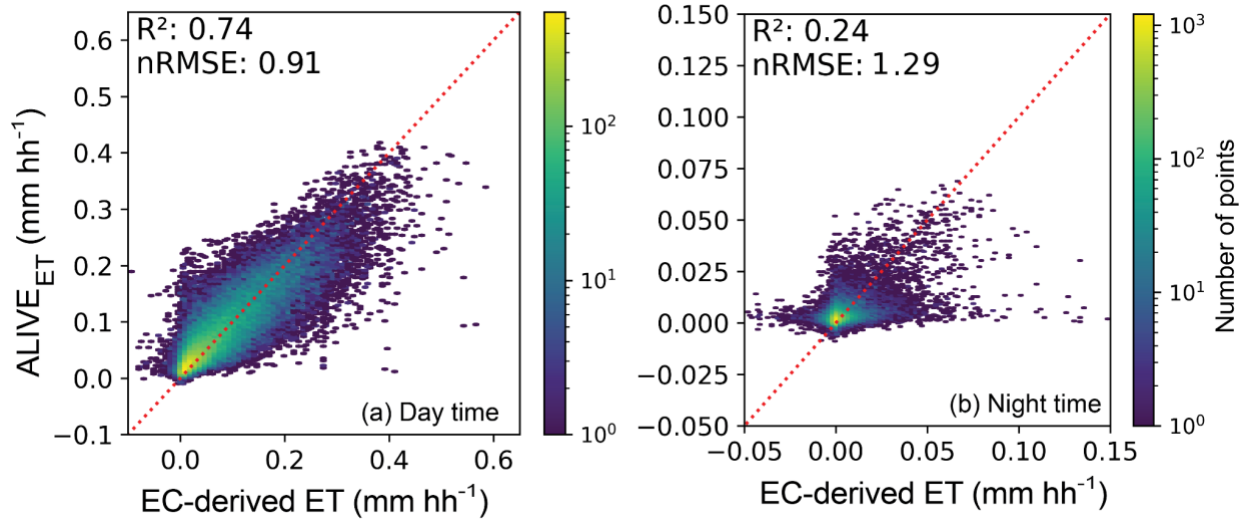
Figure 2. Density scatter plots of EC-derived ET (mm hh -1 ) (a) vs. daytime ALIVE ET estimated from GBR trained on single time observations (n=17480) and (b) nighttime ALIVE ET estimated from LSTM trained on time series observations (n=14304).
