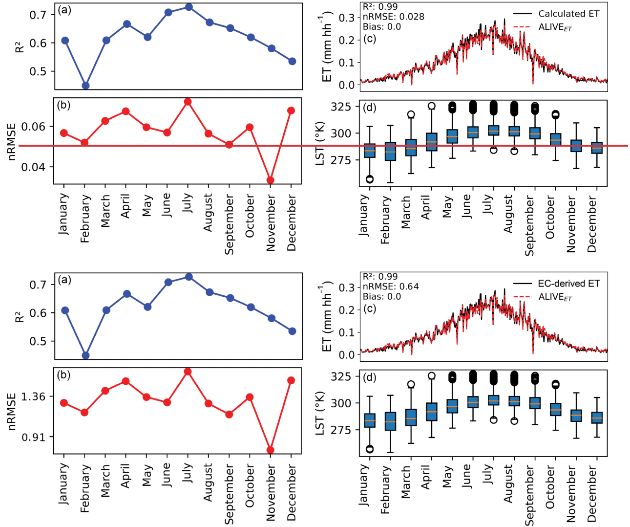
Figure 4. Model performance across different months: (a) R^2 values, (b) nRMSE values, (c) model fit for mean daily ET (mm hh^{-1} ) over the entire year of 2023, and (d) LST distribution showing monthly variability with boxplots.
