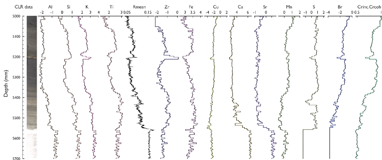
Fig. S5: All CLR XRF data from core AMS22_COMP1. A selection is shown in Fig. 3 of the main text.
