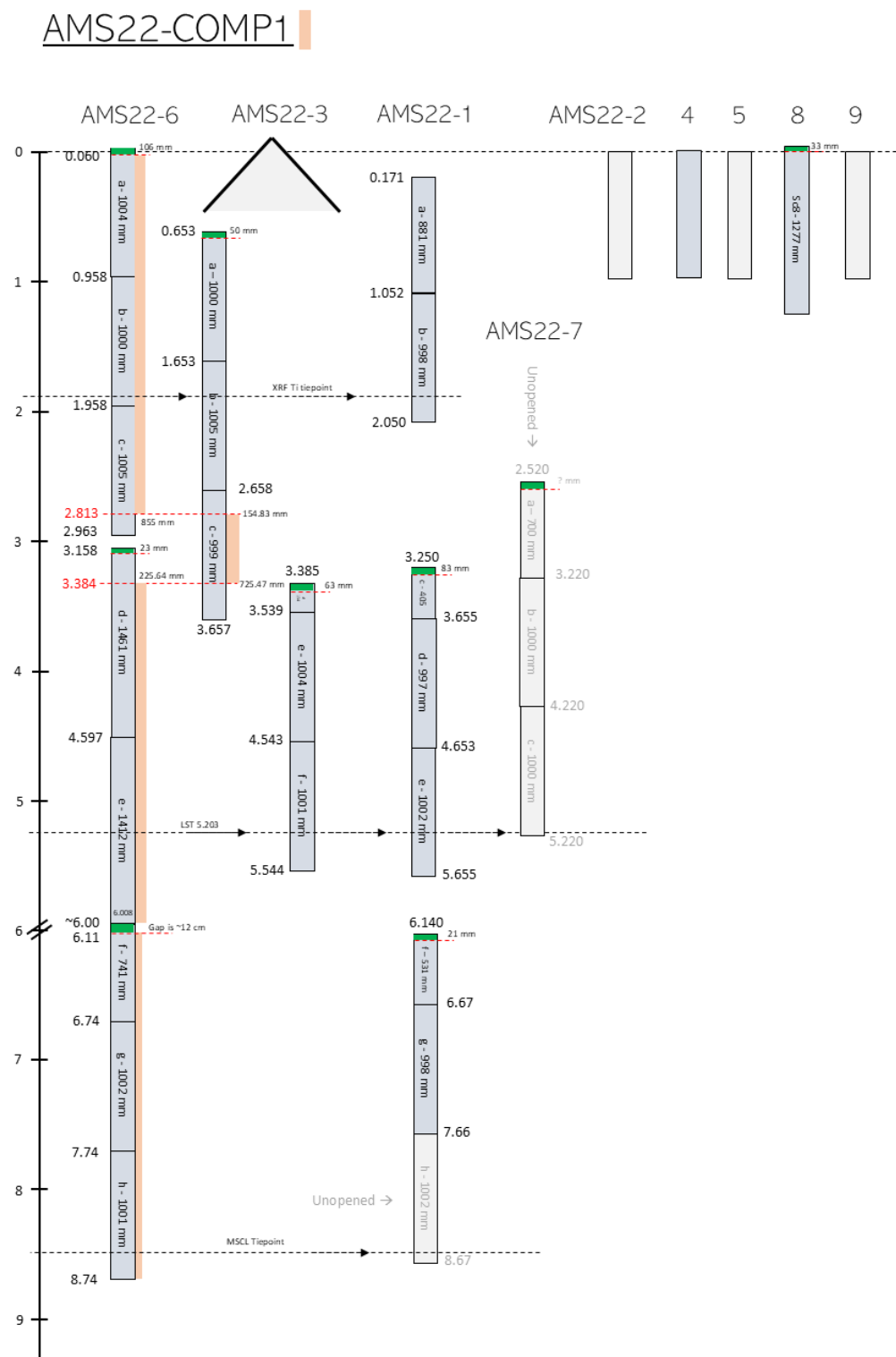
Fig. S1: Core segments, stratigraphic correlation and composite core of Amsoldingensee (coring August 2022)
