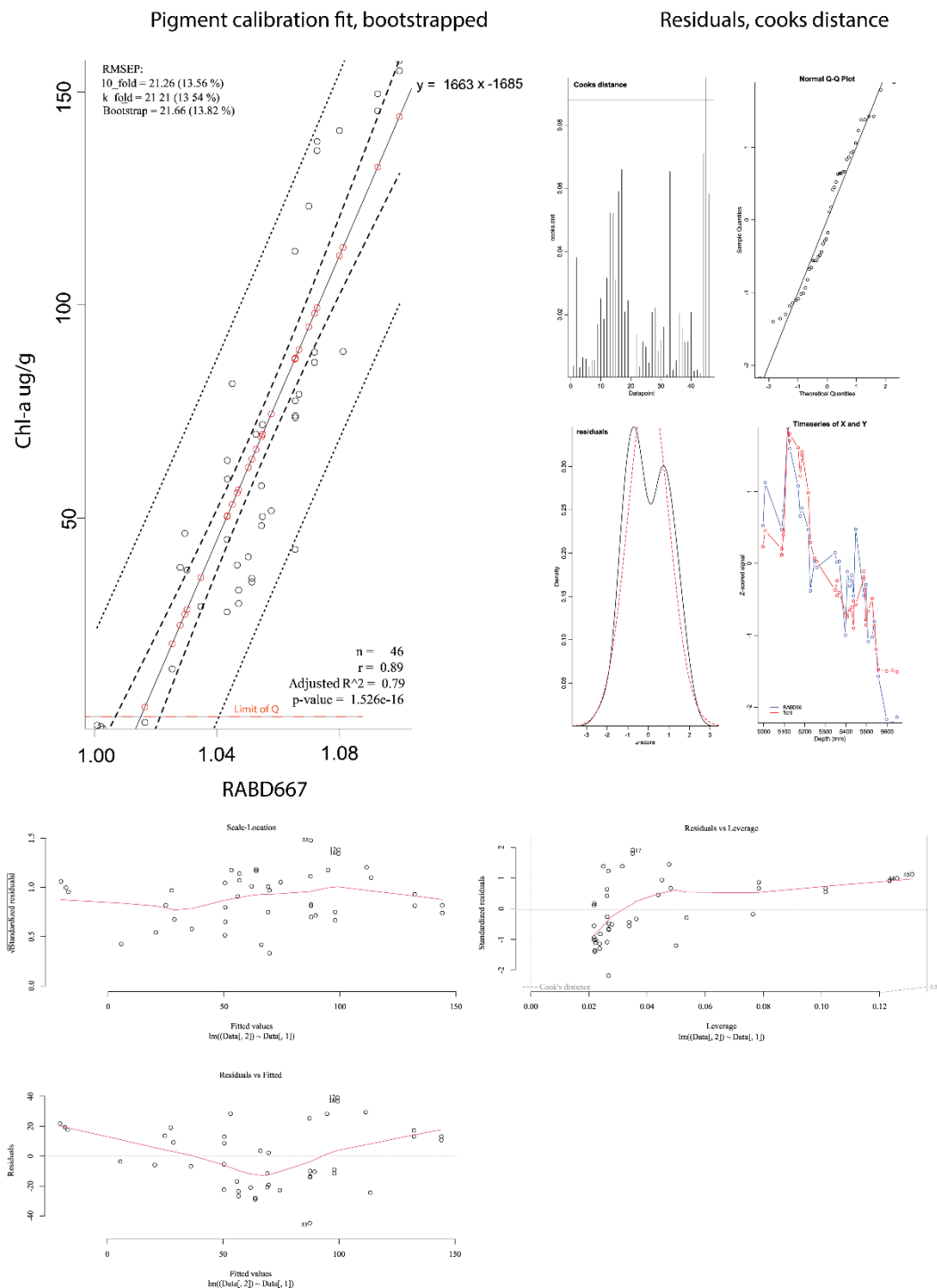
Fig. S3: Calibration of RABD667 (inferred from hyperspectral imaging) to chl a measured with UV-VIS (spectrophotometry) after pigment extraction (proxy-proxy calibration, Butz et al., 2015). Fig. S3 (left) shows the regression with 95% confidence (dashed line) and prediction intervals (dotted line) and the calibration statistics (n, p-values, R^2_{adj} , RMSEP for 10-fold jackknifing, k-fold jackknifing, and bootstrapped); the orange horizontal dashed line represents the Limit of Quantification. The panels in the middle show the Q-Q plot, Cook's Distance, the time series comparison, the residual distribution and (right panels) the scale-location, residual trajectory and leverage plots.
