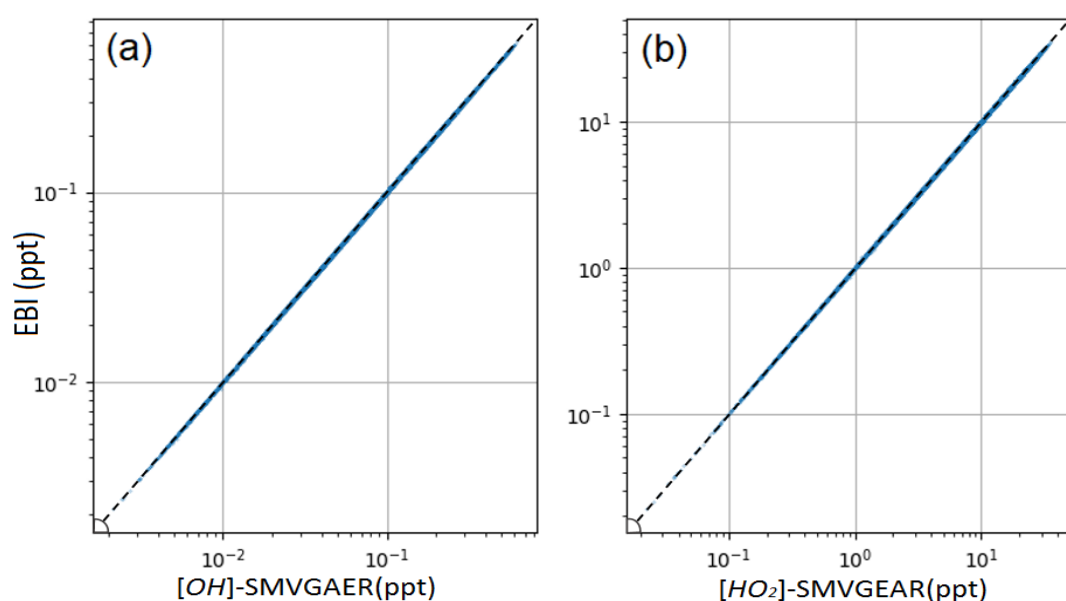
Fig. 3. Comparison of predicted OH (a) and \text{HO}_2 (b) radicals in the surface layer of the 36-km resolution domain using the source-oriented EBI(new) and the SMVGEAR(baseline)
