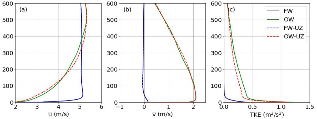
Figure B1. Vertical profiles of time-averaged horizontal velocity components \bar{u} , \bar{v} , and turbulent kinetic energy for wind-following (FW) and wind-opposing (OW) wave cases using vertically stretched grids (solid lines) and uniform vertical grids (dashed lines).
