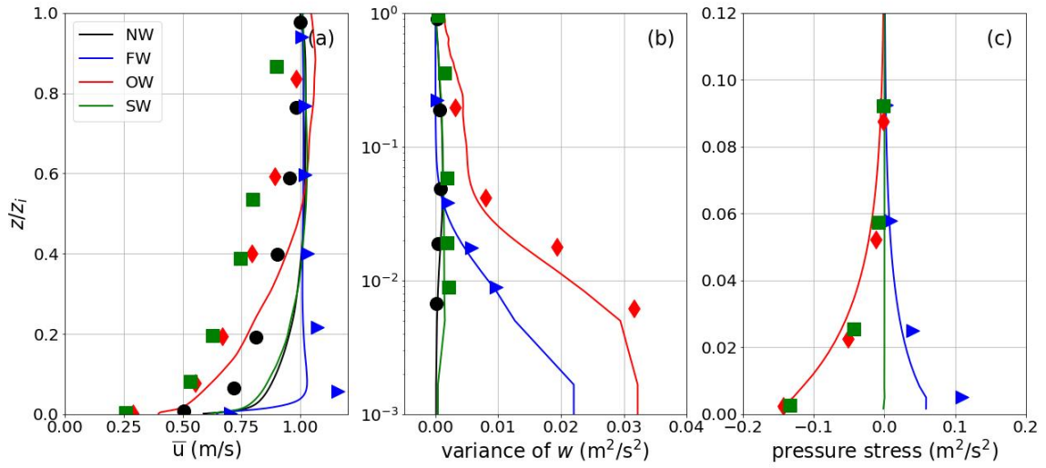
Figure C1. Comparison of vertical profiles of key flow statistics from the present study (solid lines) and Sullivan et al. (2008) (data points represented by markers) for (a) mean streamwise velocity, (b) variance of vertical velocity, and (c) wave-induced pressure stress, for the NW, FW, OW, and SW cases. Profiles are shown as a function of normalized height z/z_i .
