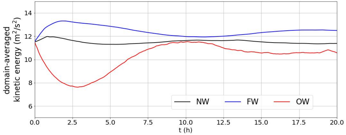
Figure A2. Temporal evolution of domain-averaged kinetic energy during the 20 h simulations for the NW, FW, and OW cases.
