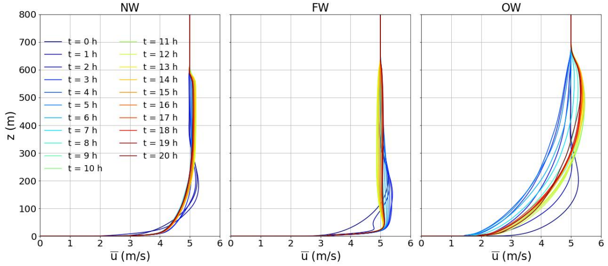
Figure A1. Temporal evolution of profiles of the horizontally averaged streamwise velocity, \bar{u} , over the 20 h simulations for the different wave configurations. Case SW exhibits nearly identical behavior to Case NW and is therefore not shown.
