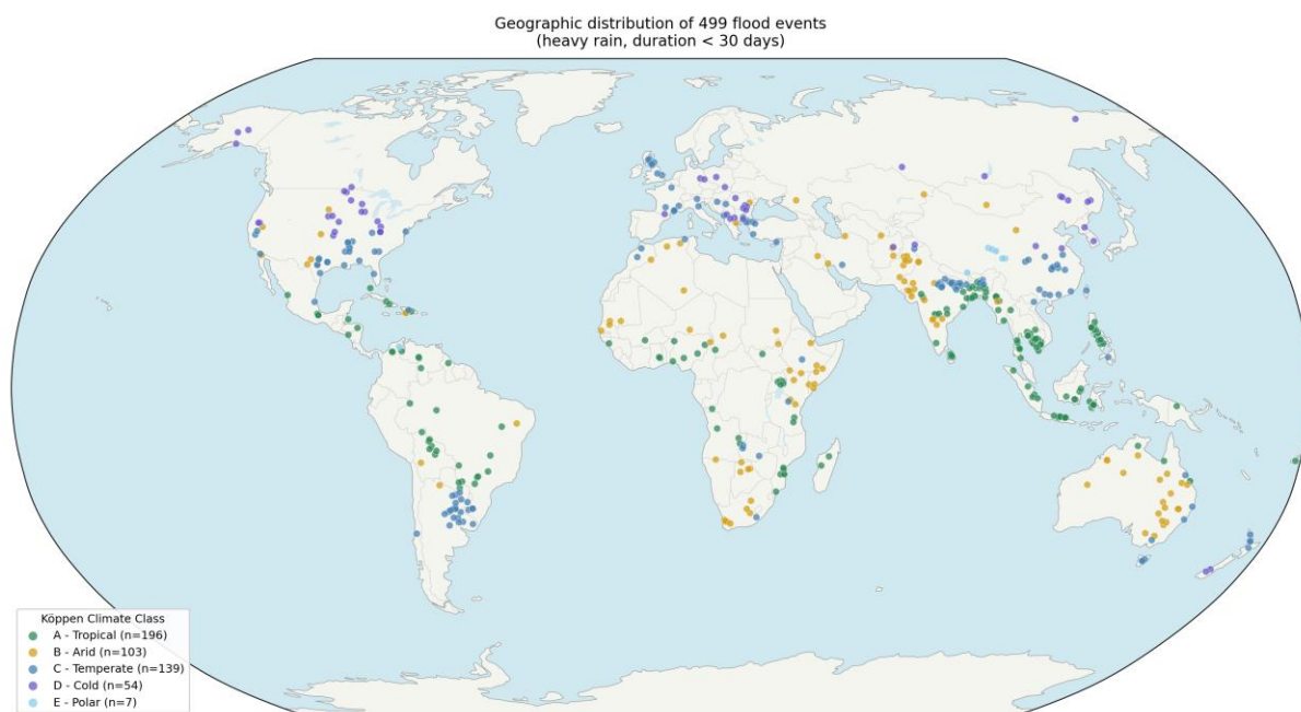
1370 Figure A5: Modelled flood events filtered from the Global Flood Database with respect to their Koeppen Climate Zones
