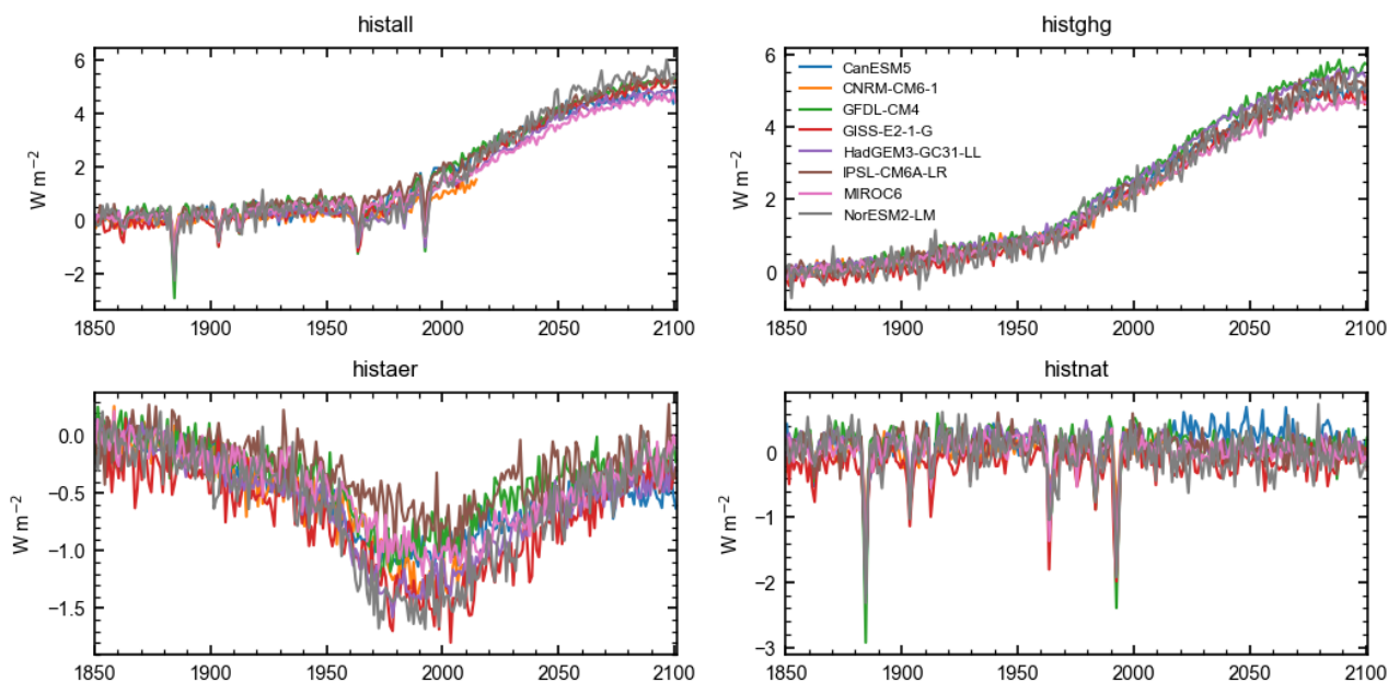
Figure 2. Global-mean timeseries of Effective Radiative Forcing from 1850 to 2100 (extended beyond 2014 using the SSP2-4.5 scenario) for all time-varying anthropogenic and natural forcings ( histall ) and, individually, for well-mixed greenhouse gases ( histghg ), anthropogenic aerosols ( histaer ) and natural forcings ( histnat ). Diagnosed in CMIP6 models using RFMIP experiments analogous to the RFMIP2.0 transient experiments tables described in Table 2.
