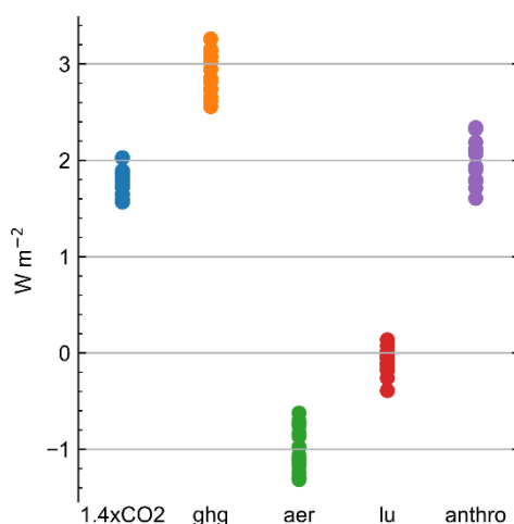
150 Figure 1. Global-mean Effective Radiative Forcing in 2014, relative to pre-industrial, for CO 2 (scaled from a 4xCO 2 simulation to approximately 1.4xCO 2 in 2014), well-mixed greenhouse gases (ghg), anthropogenic aerosols (aer), land use (lu), and all anthropogenic
