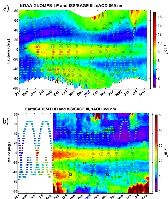
Figure 2. Time-latitude variation of zonal-mean stratospheric aerosol optical depth (SAOD) since April 2024 from OMPS-LP at 869 nm (a) and ATLID at 355 nm (b). Circles in both panels indicate SAGE III 3 day/5° latitude averages of SAOD at the corresponding wavelengths. Black triangle in a) marks the location/timing of Ruang eruption. Black squares in b) indicate the timing and location of suborbital measurements with NDACC lidars and AZOR balloon soundings.
