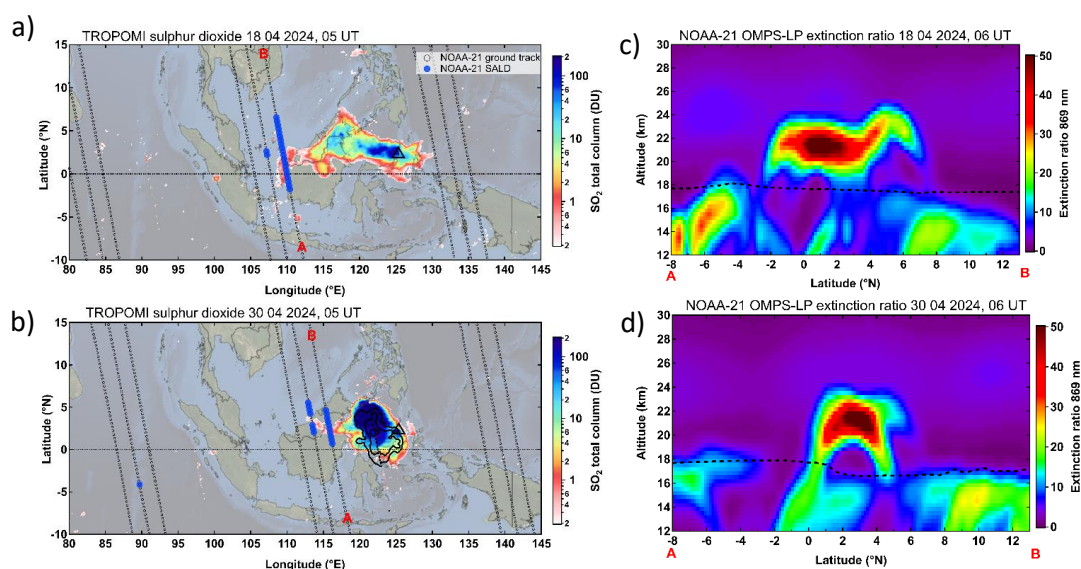
Figure 1. Ruang eruptive sequence in April 2024. a) SO 2 total column map from TROPOMI on 18 April 2024 overlaid by NOAA-21 OMPS-LP ground projections (open circles) and stratospheric aerosol layer detections (SALD, blue circles). The location of Ruang volcano is shown as triangle. b) Same as a) but on 30 April 2024 with black contours indicating TROPOMI absorbing aerosol index above 2 with contour interval of 3. c) Vertical section of OMPS-LP aerosol extinction ratio at 869 nm along the orbital segment A – B (as indicated in the map) on 18 April 2024. Dashed curve marks the tropopause altitude. d) same as c) but on 20 April 2024.
