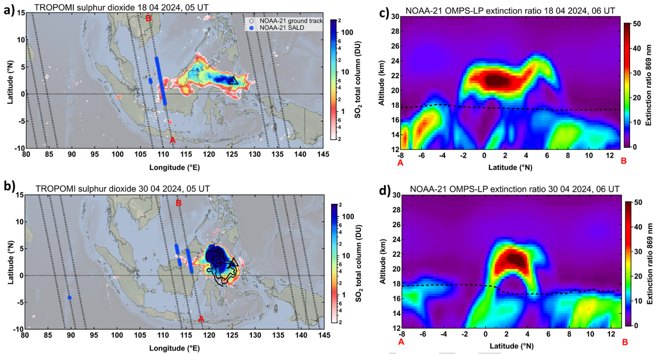
Figure 1. Ruang eruptive sequence in April 2024. (a) SO 2 total column map from TROPOMI on 18 April 2024 overlaid by NOAA-21 OMPS-LP ground projections (open circles) and stratospheric aerosol layer detections (SALD, blue circles). The location of Ruang volcano is shown as triangle. (b) Same as (a) but on 30 April 2024 with black contours indicating TROPOMI absorbing aerosol index above 2 with contour interval of 3. (c) Vertical section of OMPS-LP aerosol extinction ratio at 869 nm along the orbital segment A–B (as indicated in the map) on 30 April 2024. Dashed curve marks the tropopause altitude. (d) same as (c) but on 20 April 2024.
