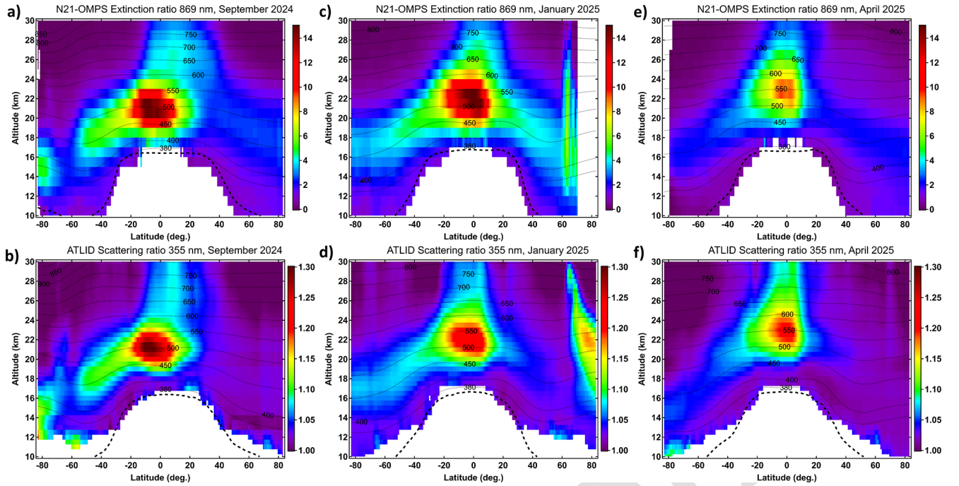
Figure 3. Zonal/monthly-mean latitude-altitude distribution of OMPS-LP extinction ratio at 869 nm (a, c, e) and ATLID scattering ratio at 355 nm (b, d, f) for September 2024 (a, b), January 2025 (c, d) and April 2025 (e, f). Dashed curve indicates the tropopause altitude, solid contours mark potential temperature levels.
