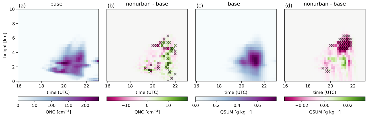
Figure 7. Horizontally averaged vertical profiles of number of activated cloud droplets QNC (a) and total cloud condensate QSUM (c), showing ensemble means for the BASE experiment for case I. (b) and (d) show the corresponding differences between the NONURBAN and BASE experiments for QNC and QSUM, respectively. Black crosses indicate levels where the differences are statistically significant at the 90 % confidence level.
