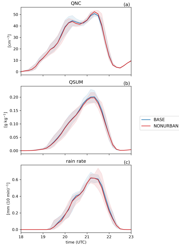
Figure 6. Horizontally averaged and layer-thickness-weighted vertical averages (0 – 13 km) time series of (a) activated cloud droplet number concentration (QNC), (b) total cloud condensate (liquid water, ice, snow, graupel, rain, and hail; QSUM), (c) horizontally averaged rain rate. Lines indicate the ensemble mean, while shading represents the ensemble minimum–maximum range. Blue lines correspond to the BASE experiment, red to the NONURBAN experiment.
