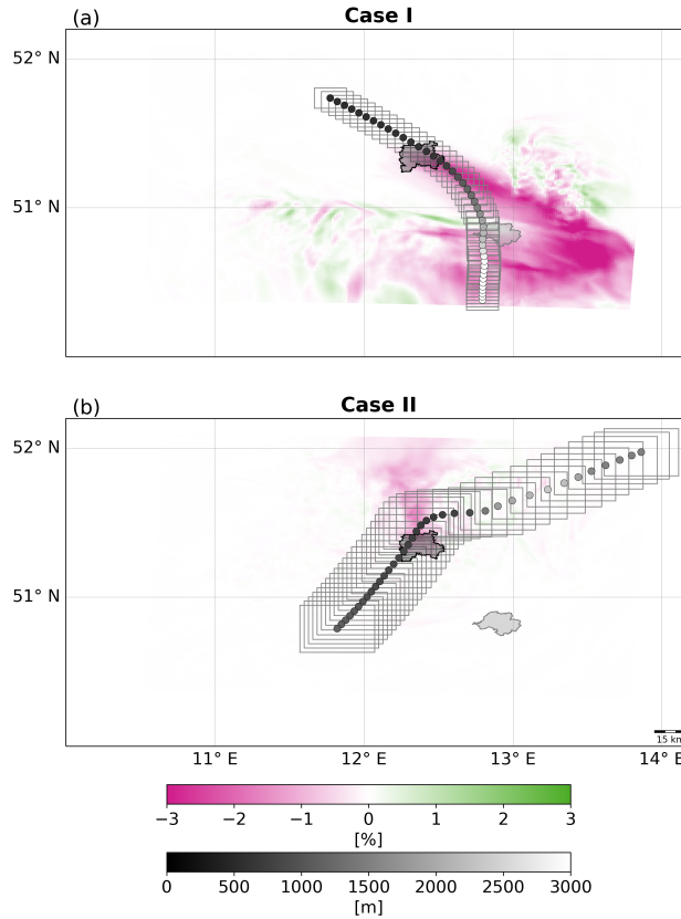
Figure 2. Mean trajectories for case I (a) and case II (b). Pink–green shading shows the percentage difference in aerosol mass concentration (NONURBAN - BASE) averaged across all aerosol species considered in the two-moment microphysics scheme (5 dust classes, ammonium sulfate, ammonium nitrate, sulfate, organic carbon, elemental carbon, 2 sea salt classes), vertically averaged below 1000 m and temporally averaged over the periods when trajectories pass through the urban aerosol plume (case I: 17:50–19:00; case II: 18:20–20:00). Grey shading indicates the average trajectory height and trajectories run in the direction towards higher altitudes. The filled areas mark the urban regions of Leipzig (dark grey) and Chemnitz (light grey). Grey boxes denote the rectangular averaging areas used to extract vertical profiles around each trajectory point.
