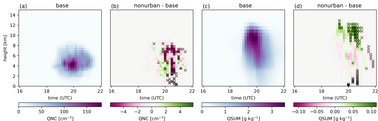
Figure 10. Horizontally averaged vertical profiles of number of activated cloud droplets QNC (a) and total cloud condensate QSUM (c), showing ensemble means for the BASE experiment for case II. (b) and (d) show the corresponding differences between the NONURBAN and BASE experiments for QNC and QSUM, respectively. Black crosses indicate levels where the differences are statistically significant at the 90 % confidence level.
