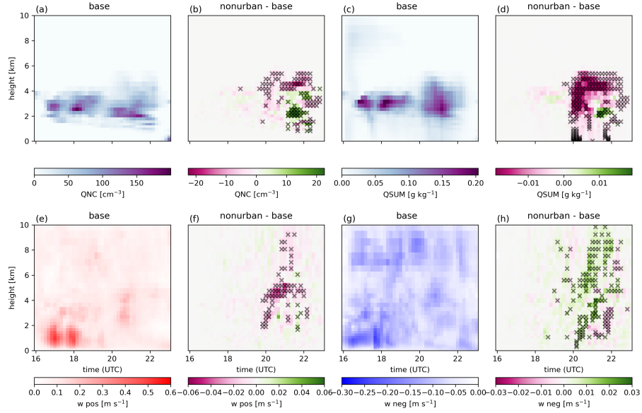
Figure A2. Top row is showing box-spatially-horizontally averaged vertical profiles of number of activated cloud droplets QNC (a) and total cloud condensate QSUM (c) along mean trajectory, showing ensemble means for the BASE experiment for case I. (b) and (d) show the corresponding differences between the NONURBAN and BASE experiments for QNC and QSUM, respectively. Bottom row is showing ensemble mean vertical profiles of positive (w pos) (e) and negative (w neg) (g) vertical velocities from the BASE experiment, spatially horizontally averaged over the analysis box along the mean trajectory for case I. Panels (b) and (d) display the deviations from the BASE case in the NONURBAN experiment. Black crosses indicate levels where the differences are statistically significant at the 90 % confidence level.
