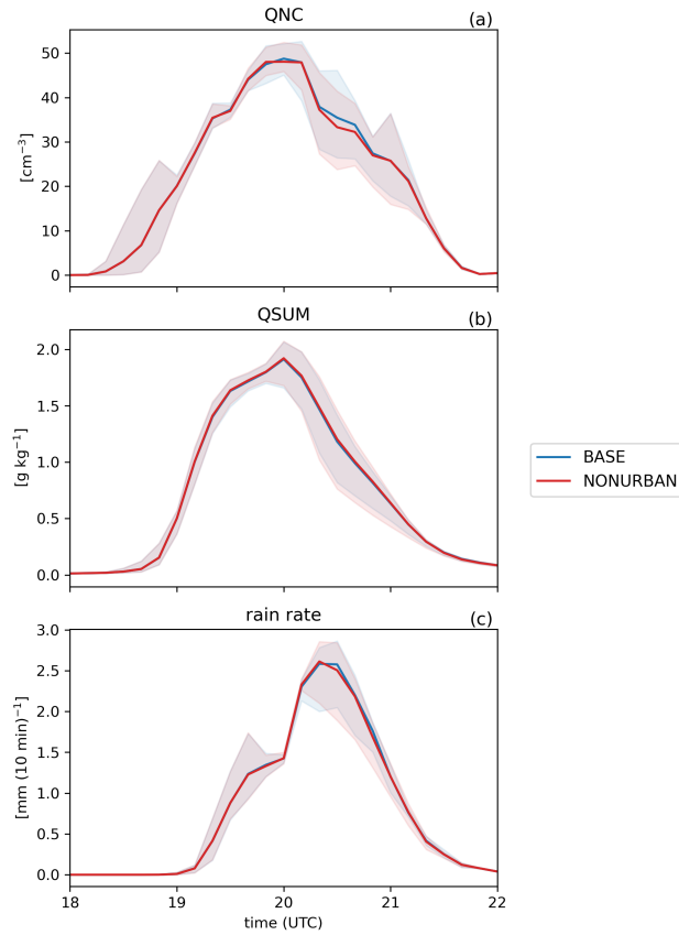
Figure 9. Box-averaged (35 × 35 km 2 ) Horizontally averaged and layer-thickness-weighted vertical averages (0–13 km) time series of (a) activated cloud droplet number concentration (QNC), (b) total cloud condensate (liquid water, ice, snow, graupel, rain, and hail; QSUM), and (c) shows box-averaged horizontally averaged rain rate. Lines indicate the ensemble mean, while shading represents the ensemble minimum–maximum range. Blue lines correspond to the BASE experiment, red to the NONURBAN experiment.
