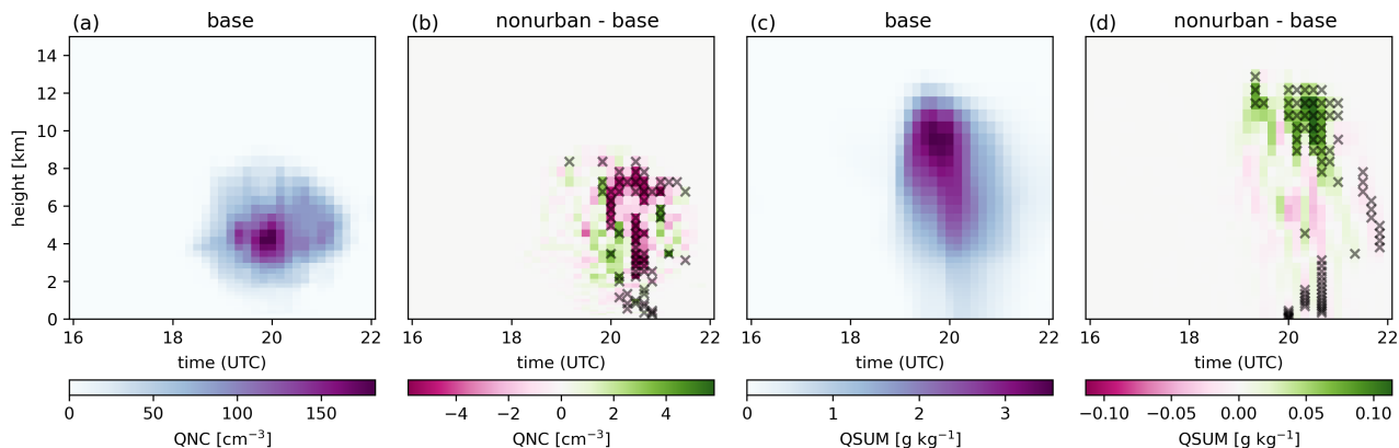
Figure 10. Box-spatially-Horizontally averaged vertical profiles of number of activated cloud droplets QNC (a) and total cloud condensate QSUM (c), showing ensemble means for the BASE experiment for case II. (b) and (d) show the corresponding differences between the NONURBAN and BASE experiments for QNC and QSUM, respectively. Black crosses indicate levels where the differences are statistically significant at the 90 % confidence level.
