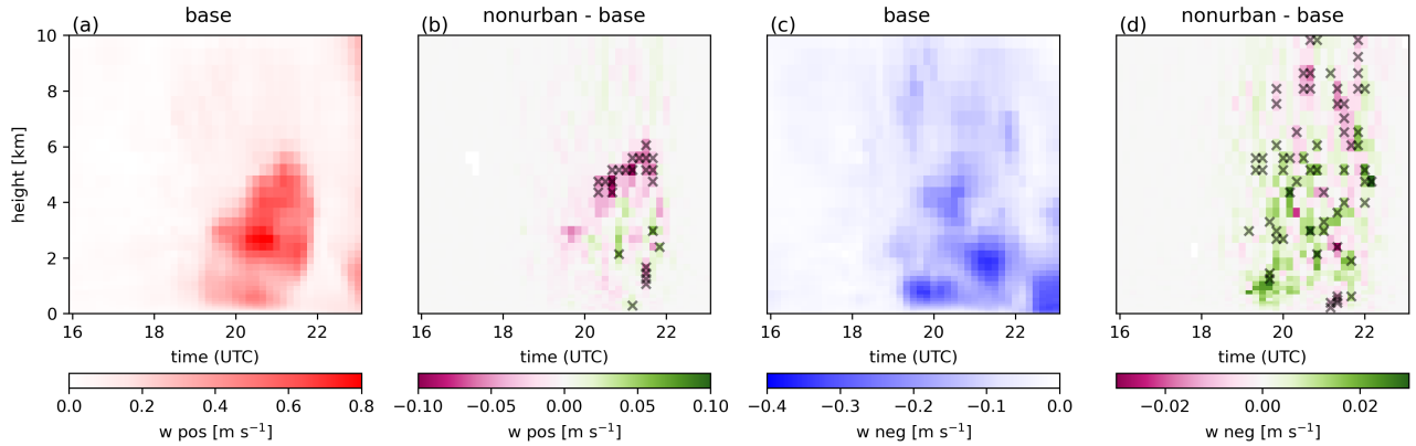
Figure 8. Ensemble mean vertical profiles of positive ( w_{\text{pos}} ) (a) and negative ( w_{\text{neg}} ) (c) vertical velocities from the BASE experiment, spatially horizontally averaged over the analysis box for case I. Panels (b) and (d) display the deviations from the BASE case in the NONURBAN experiment. Statistically significant differences at the 90 % confidence level are marked with black crosses. Note: color pattern reversed for w_{\text{neg}} , as values are negative.
