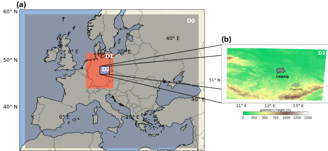
Figure 1. (a) Model domains used in the simulation: Europe-D0 (14 km grid resolution), D1 (2.3 km), and D2 (1 km). (b) Inner model domain D2 showing geometric height of the earth's surface above sea level. The cities Leipzig and Chemnitz are shown as filled areas in grey and light grey to indicate their urban extent.
