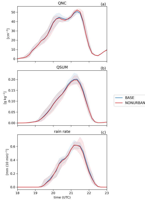
Figure 6. Box-averaged ( 15 \times 15 \text{ km}^2 ) Horizontally averaged and layer-thickness-weighted vertical averages (0 – 13 km) time series of (a) activated cloud droplet number concentration (QNC), (b) total cloud condensate (liquid water, ice, snow, graupel, rain, and hail; QSUM), (c) shows-box-averaged horizontally averaged rain rate. Lines indicate the ensemble mean, while shading represents the ensemble minimum–maximum range. Blue lines correspond to the BASE experiment, red to the NONURBAN experiment.
