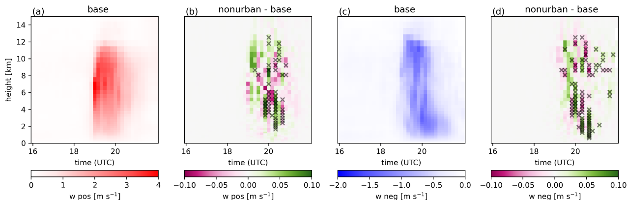
Figure 11. Ensemble mean vertical profiles of positive ( w_{\text{pos}} ) (a) and negative ( w_{\text{neg}} ) (c) vertical velocities from the BASE experiment, spatially horizontally averaged over the analysis box for case II. Panels (b) and (d) display the deviations from the BASE case in the NONURBAN experiment. Statistically significant differences at the 90 % confidence level are marked with black crosses. Note: color pattern reversed for w_{\text{neg}} , as values are negative.
