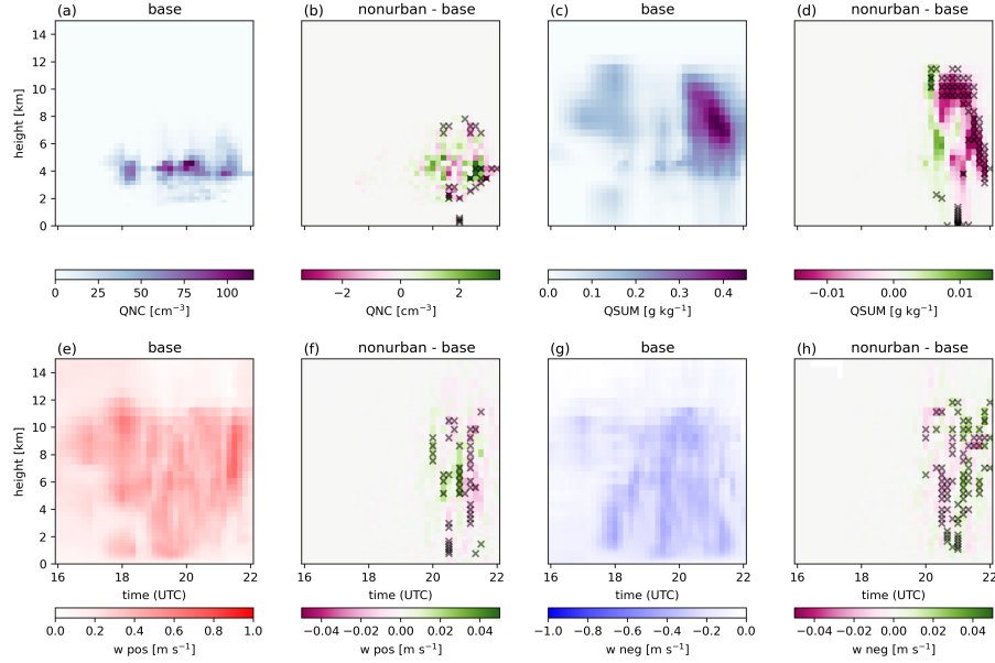
Figure A3. Top row is showing box-spatially-horizontally averaged vertical profiles of number of activated cloud droplets QNC (a) and total cloud condensate QSUM (c) along mean trajectory, showing ensemble means for the BASE experiment for case II. (b) and (d) show the corresponding differences between the NONURBAN and BASE experiments for QNC and QSUM, respectively. Bottom row is showing ensemble mean vertical profiles of positive (w pos) (a) and negative (w neg) (c) vertical velocities from the BASE experiment, spatially horizontally averaged over the analysis box along the mean trajectory for case II. Panels (b) and (d) display the deviations from the BASE case in the NONURBAN experiment. Black crosses indicate levels where the differences are statistically significant at the 90 % confidence level.
