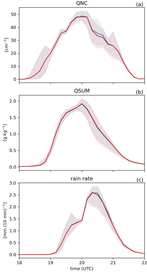
Figure 9. Box-averaged ( 35 \times 35 \text{ km}^2 ) and layer-thickness-weighted vertical averages (0 – 13 km) time series of (a) activated cloud droplet number concentration (QNC), (b) total cloud condensate (liquid water, ice, snow, graupel, rain, and hail; QSUM), (c) shows box-averaged rain rate. Lines indicate the ensemble mean, while shading represents the ensemble minimum–maximum range. Blue lines correspond to the BASE experiment, red to the NONURBAN experiment.
