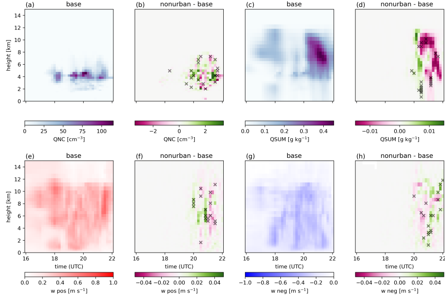
Figure A3. Top row is showing box spatially averaged vertical profiles of number of activated cloud droplets QNC (a) and total cloud condensate QSUM (c) along mean trajectory, showing ensemble means for the BASE experiment for case II. (b) and (d) show the corresponding differences between the NONURBAN and BASE experiments for QNC and QSUM, respectively. Bottom row is showing ensemble mean vertical profiles of positive (w pos) (e) and negative (w neg) (g) vertical velocities from the BASE experiment, spatially averaged over the analysis box along the mean trajectory for case II. Panels (b) and (d) display the deviations from the BASE case in the NONURBAN experiment. Black crosses indicate levels where the differences are statistically significant at the 90 % confidence level.
