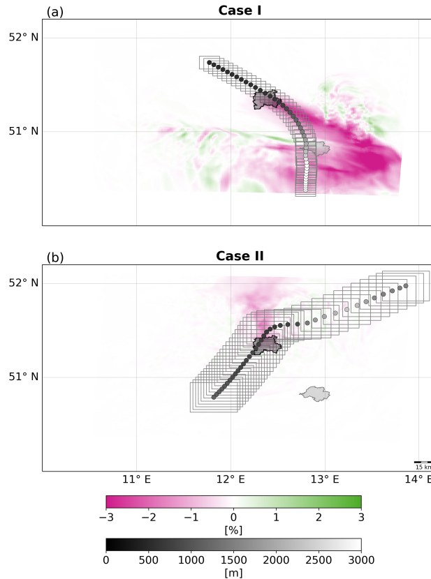
Figure 2. Mean trajectories for Case-case I (a) and Case-case II (b). Pink–green shading shows the percentage difference in the-mean-of aerosol mass concentration (NONURBAN - BASE) averaged across all aerosol species considered in the two-moment microphysics scheme (5 dust classes, ammonium sulfate, ammonium nitrate, sulfate, organic carbon, elemental carbon, 2 sea salt classes), vertically averaged below 1000 m and temporally averaged over the periods when trajectories pass through the urban aerosol plume ( Case-case I: 17:50–19:00; Case-case II: 18:20–20:00) between the NONURBAN and BASE experiments, covering the period from entering the urban area until ascent above 1000 m. Grey shading indicates the average trajectory height and the trajectories run in the direction towards higher altitudes. The filled areas mark the urban regions of Leipzig (dark grey) and Chemnitz (light grey). Grey boxes denote the rectangular averaging areas used to extract vertical profiles around each trajectory point.
