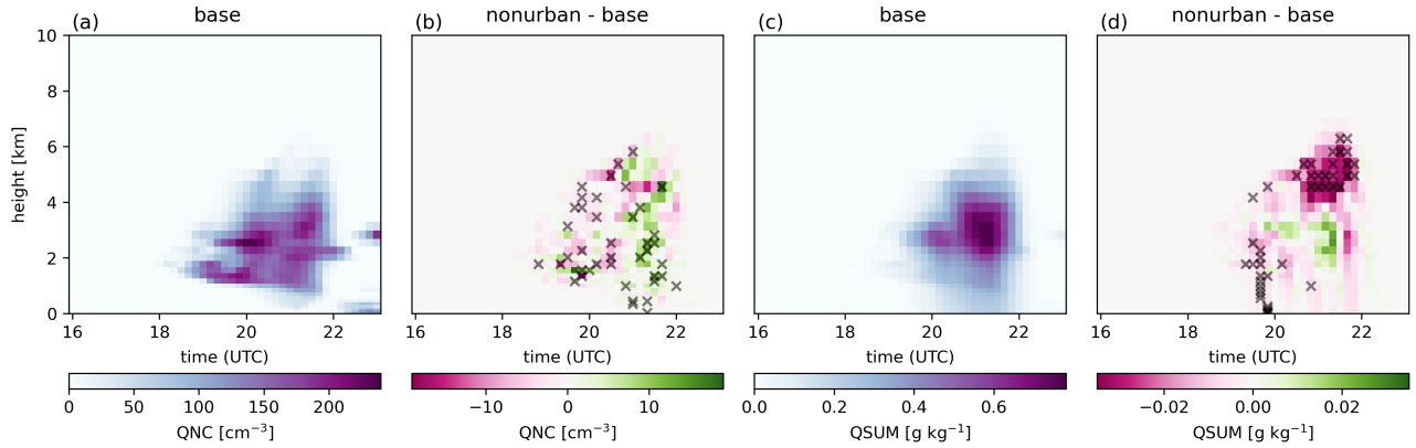
Figure 7. Box spatially averaged vertical profiles of number of activated cloud droplets QNC (a) and total cloud condensate QSUM (c), showing ensemble means for the BASE experiment for case I. (b) and (d) show the corresponding differences between the NONURBAN and BASE experiments for QNC and QSUM, respectively. Black crosses indicate levels where the differences are statistically significant at the 90 % confidence level.
