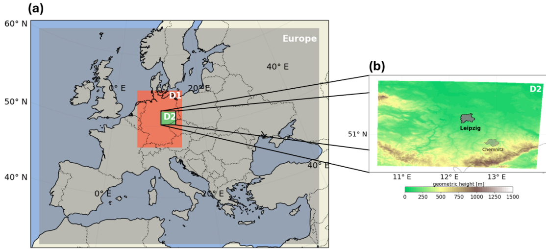
Figure 1. (a) Model domains used in the simulation: Europe (14 km grid resolution), D1 (2.3 km), and D2 (1 km). (b) Inner model domain D2 showing geometric height of the earth's surface above sea level. The cities Leipzig and Chemnitz are shown as filled areas in grey and light grey to indicate their urban extent.
