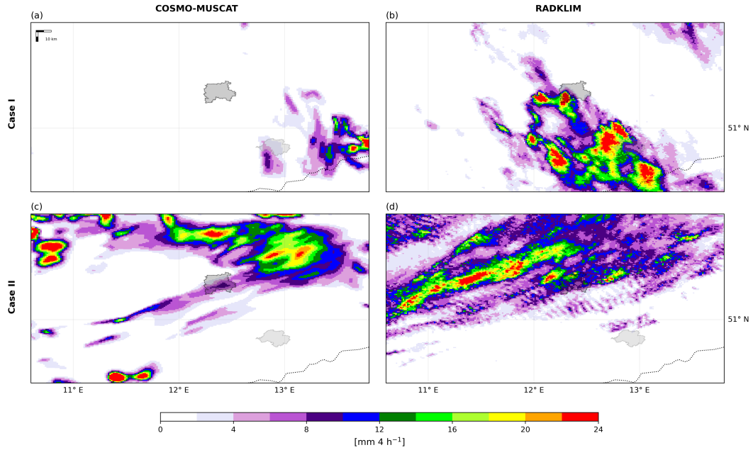
Figure 3. Accumulated precipitation over a 4-hour period for both cases. Simulated precipitation ensemble mean from COSMO-MUSCAT (a, c) and radar-derived precipitation from RADKLIM (b, d) for Case-case Case I (top row) and Case-case Case II (bottom row).
