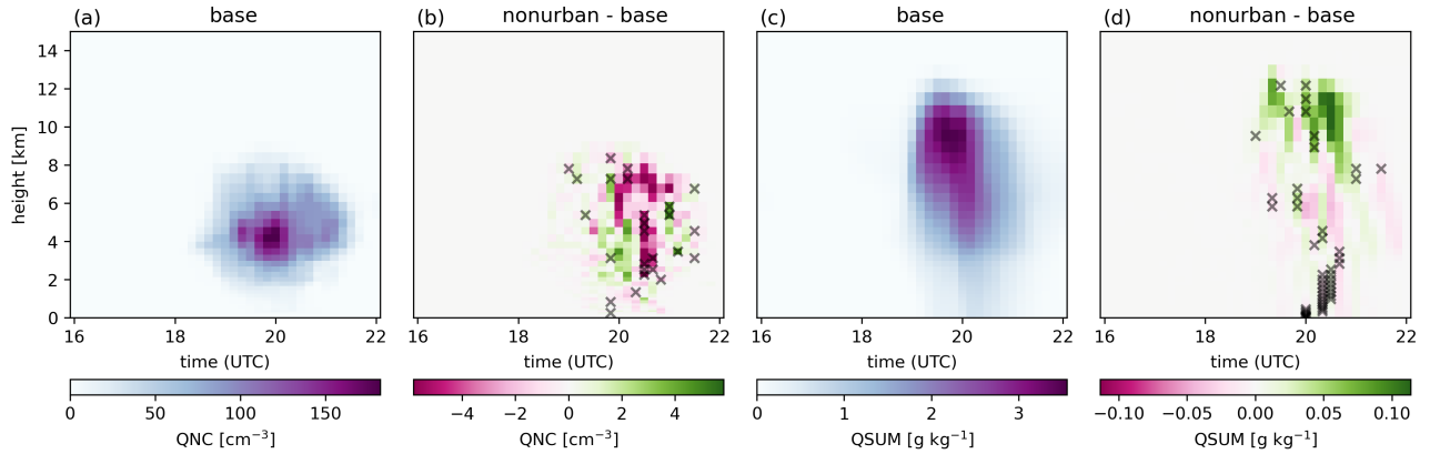
Figure 10. Box spatially averaged vertical profiles of number of activated cloud droplets QNC (a) and total cloud condensate QSUM (c), showing ensemble means for the BASE experiment for case II. (b) and (d) show the corresponding differences between the NONURBAN and BASE experiments for QNC and QSUM, respectively. Black crosses indicate levels where the differences are statistically significant at the 90 % confidence level.
