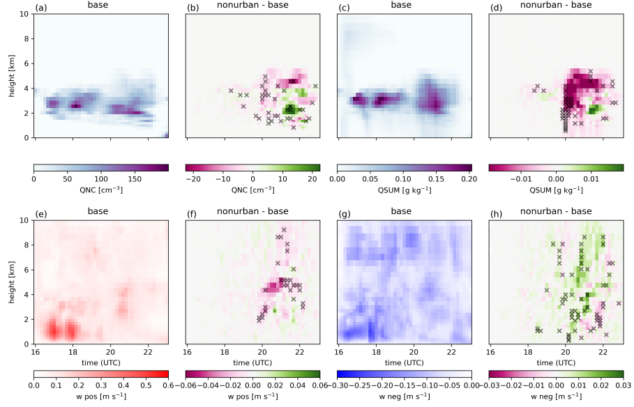
Figure A2. Top row is showing box spatially averaged vertical profiles of number of activated cloud droplets QNC (a) and total cloud condensate QSUM (c) along mean trajectory, showing ensemble means for the BASE experiment for case I. (b) and (d) show the corresponding differences between the NONURBAN and BASE experiments for QNC and QSUM, respectively. Bottom row is showing ensemble mean vertical profiles of positive ( w_{\text{pos}} ) (e) and negative ( w_{\text{neg}} ) (g) vertical velocities from the BASE experiment, spatially averaged over the analysis box along the mean trajectory for case I. Panels (b) and (d) display the deviations from the BASE case in the NONURBAN experiment. Black crosses indicate levels where the differences are statistically significant at the 90 % confidence level.
