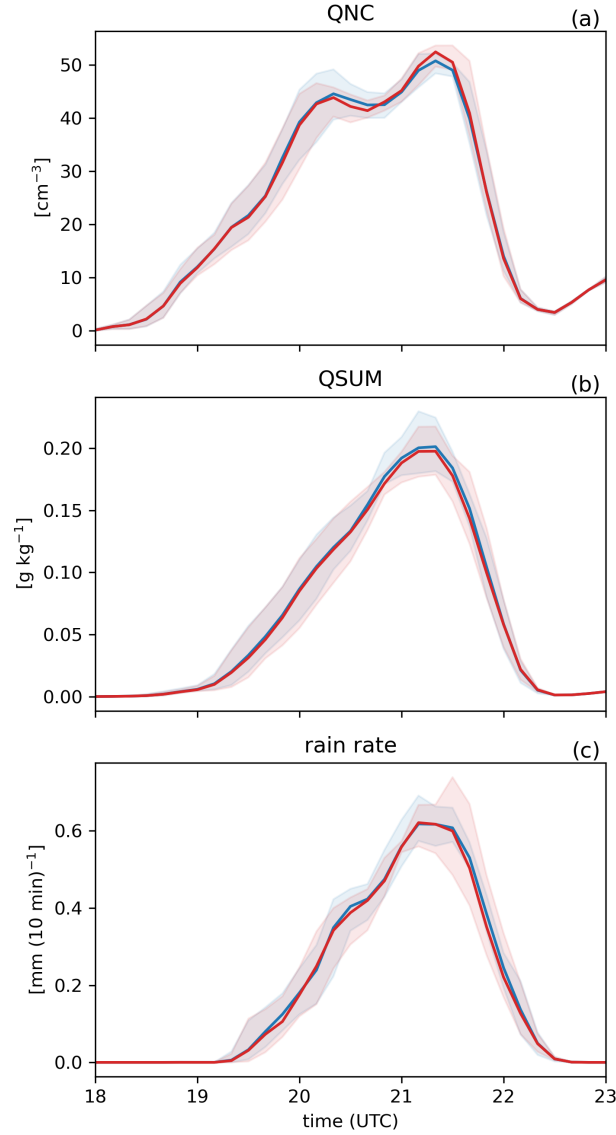
Figure 6. Box-averaged ( 15 \times 15 \text{ km}^2 ) and layer-thickness-weighted vertical averages (0 – 13 km) time series of (a) activated cloud droplet number concentration (QNC), (b) total cloud condensate (liquid water, ice, snow, graupel, rain, and hail; QSUM), (c) shows box-averaged rain rate. Lines indicate the ensemble mean, while shading represents the ensemble minimum–maximum range. Blue lines correspond to the BASE experiment, red to the NONURBAN experiment.
