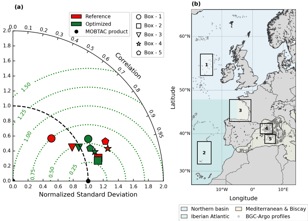
Figure 10. Surface chlorophyll-a validation against the MOBTAC multi-observation reprocessed product over the period 2017–2019. (a) Taylor diagram computed on monthly mean time series in log 10 space. The radial distance from the origin represents the normalised standard deviation ( \sigma_{\text{model}}/\sigma_{\text{obs}} ), the angular position the Pearson correlation coefficient, and the green dotted contours the centred root-mean-square difference. Red markers denote the REF simulation and green markers the OPTI simulation; marker shapes identify the five validation boxes (circle: Box 1; square: Box 2; inverted triangle: Box 3; star: Box 4; pentagon: Box 5). The black filled circle indicates the MOBTAC reference point at unit normalised standard deviation, and the black dashed semicircle marks the locus where model and observed variability are equal ( \sigma_{\text{model}}/\sigma_{\text{obs}} = 1 ). (b) Location of the five validation boxes within the IBI domain: Box 1 (Celtic Sea / Rockall Trough), Box 2 (Canary / Madeira), Box 3 (Bay of Biscay), Box 4 (Gulf of Lion), and Box 5 (Balearic Sea). The three broader sub-regions for subsurface BGC-Argo validation are delineated by colored polygons: Northern basin (20°W–17°E, 48–65°N), Iberian Atlantic (20–5°W, 26–48°N), and Mediterranean & Bay of Biscay (5°W–17°E, 26–48°N). Individual profile locations from the approximately 1,430 BGC-Argo profiles matched to the IBI model over 2017–2019 are shown as grey dots.
