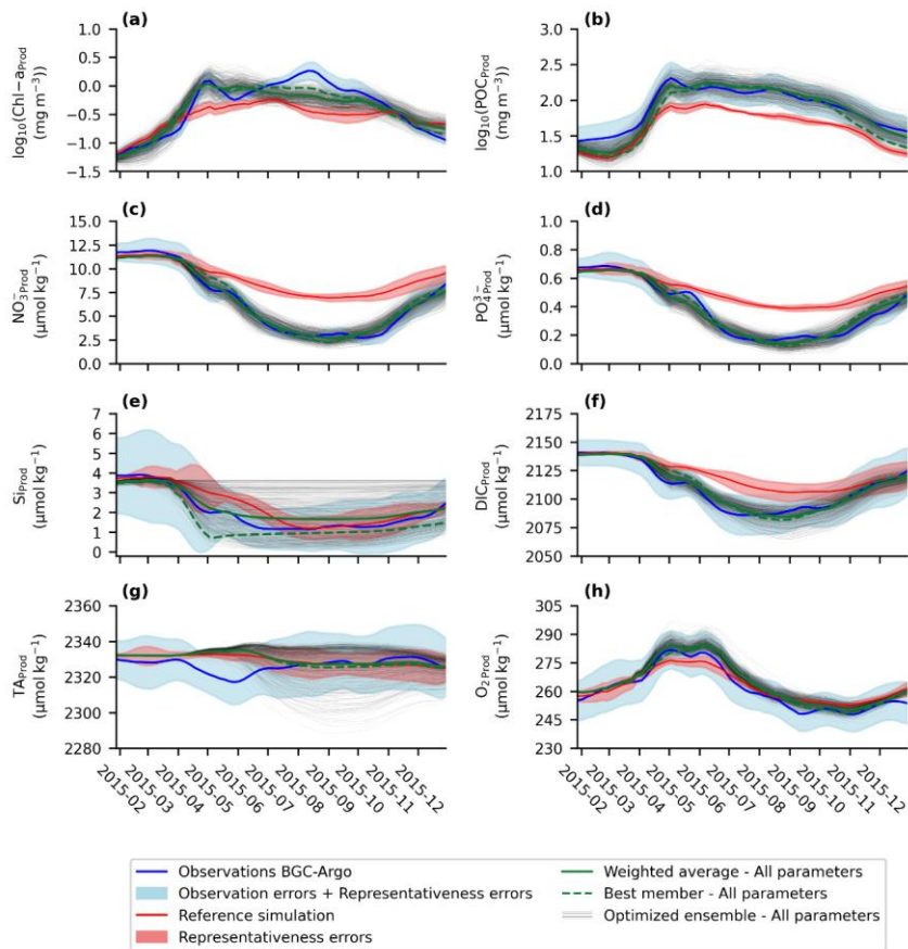
Figure 5. Seasonal cycle of assimilated metrics in the productive layer. Panels show: (a) \log_{10}(\text{Chl} - a_{\text{Prod}}) , (b) \log_{10}(\text{POC}_{\text{Prod}}) , (c) \text{NO}_3^-_{\text{Prod}} , (d) \text{PO}_4^{3-}_{\text{Prod}} , (e) \text{Si}_{\text{Prod}} , (f) \text{DIC}_{\text{Prod}} , (g) \text{TA}_{\text{Prod}} , and (h) \text{O}_{2\text{Prod}} . The blue curve represents observations from BGC-Argo float #5904479, with the blue shading indicating the combined observations and representativity errors. The red curve corresponds REF from PISCES-1D, with the red shading representing representativity errors. Green line indicate the weighted means of the ensemble optimized using All parameters of the PISCES model. The black curves represent the ensemble of selected members obtained by optimizing all parameters of the PISCES model. A six-point moving average was applied to all time series to smooth short-term fluctuations.
