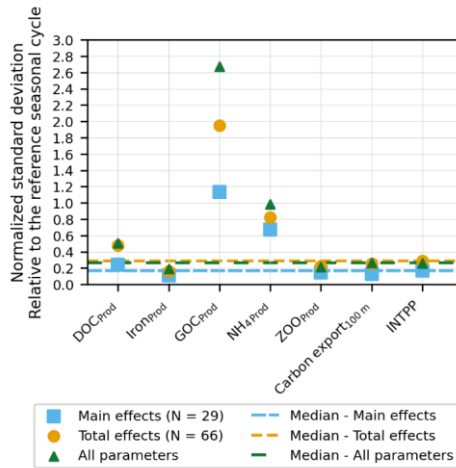
Figure 8. Standard deviation (unitless) of the ensemble optimized using different parameter selection strategies, normalized by the variability of the seasonal cycle in REF. The X-axis indicates non-assimilated state variables as well as two derived outputs : carbon export at 100 m depth and integrated net primary production (INTPP). Results are shown for the three parameter selection strategies : 'Main effects (N=29)', 'Total effects (N=66)' and 'All parameters'. Each point corresponds to a specific metric, with dashed lines indicating the median value.
