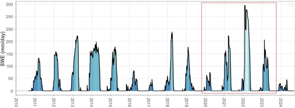
515 Figure 8: SWE values during the 2010-2024 period for the MDU catchment. The red rectangle represents the period used to compute the water budget.
