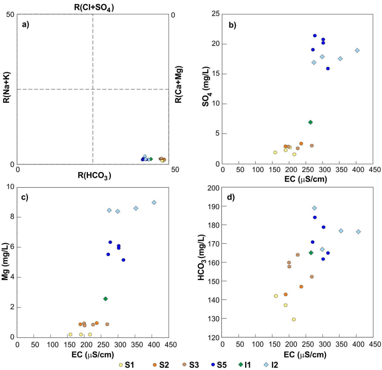
Figure 6: a) Langelier-Ludwig diagram for the Ussita stream; b) sulphate concentrations vs EC values; c) Magnesium concentrations vs EC values; d) Alkalinity vs EC values. For the location of sampling points, see Fig. 1.
