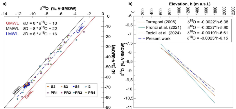
Figure 7: a) \delta\text{D} vs \delta^{18}\text{O} values of precipitation samples with the resulting linear regression (Local Meteoric Water Line, LMWL), compared with the Global Meteoric Water Line (GMWL) and the Mediterranean Meteoric Water Line (MMWL); b) Linear regression between \delta^{18}\text{O} and elevation determined by four water collectors (PR) with those proposed by Tarragoni (2006), Fronzi et al. (2021), and Tazioli et al. (2024). For the location of sampling points, see Fig. 1.
