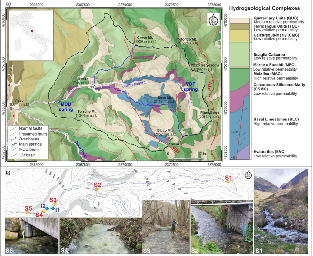
Figure 1: a) Map of hydrogeological complexes of the Ussita Stream catchment based on the geological map of Pierantoni et al. (2013). MDU = Ussita catchment at Madonna Dell’Uccelletto (MDU); UV = Ussita catchment at Ussita Village (UV); VDP = Val Di Panico spring; VBF = Mt. Vettore-Mt. Bove Fault system; PTV = Pizzo Tre Vescovi thrust. b) The location of stream gauges with reliable rating curves (S2 and S5), stream sections monitored by spot measurements with the OTT MF Pro flow meter (S1, S3, and S4), and GW inflow (I1 and I2). The grey shadow zone represents the outcropping of the low-permeability Marne a Fucoidi Complex (MFC).
