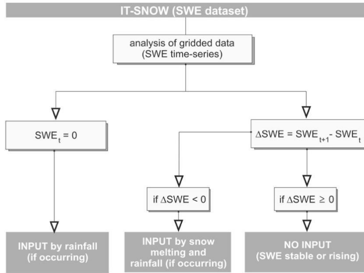
Figure 2: Workflow for analyzing water availability contribution from IT-SNOW's SWE data.
