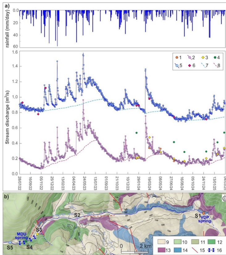
430 Figure 4: a) Daily stream discharge data at stream gauges S2 and S5 with rainfalls recorded at Ussita gauge and base flow curves and the discrete monitoring carried out along the stream (1 – S1 section; 2 – S2 section; 3 – S3 section; 4 – S4 section; 5 – S5 section; 6 – discrete monitoring in S5 section; 7 – Base Flow at S5 section; 8 – Base Flow at S2 section). b) location of stream sections on the geological map of Fig. 1a (9 – QUC; 10 – SCC; 11 – MFC; 12 – MAC; 13 – CSMC; 14 – BLC; 15 – Normal faults; 16 – Main GW inflows to the stream).
