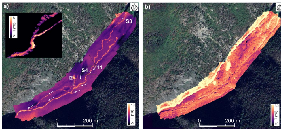
435 Figure 5: a) thermal drone investigations carried out in January 2024 and b) in July 2025. Base map: map data © 2025 Google.
