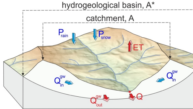
300 Figure 3: Schematic representation of a hydrogeological system with groundwater inflow coming outside the catchment area (A). A^* = recharge area.
