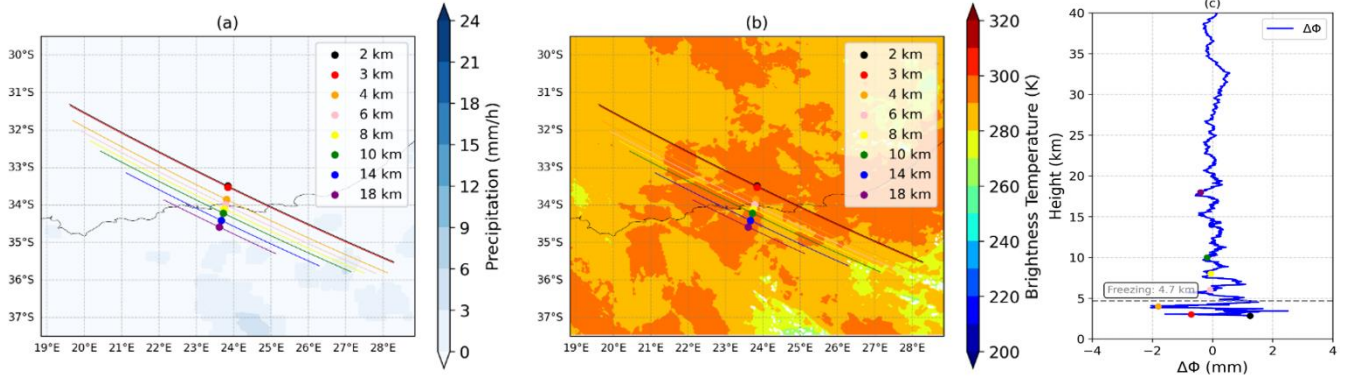
Figure 11. \Delta\Phi not induced by precipitation. (a) The IMERG precipitation product collocated with the Yunyao PRO profile on the southern coastline of Africa. (b) The brightness temperature data collocated with the Yunyao PRO profile. (c) The corresponding \Delta\Phi values for each PRO tangent point. Each line represents the \Delta\Phi along a single occultation ray path, with color denoting the altitude of its tangent point. The gray dashed line represents the freezing level.
