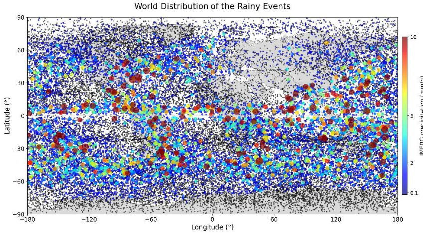
145 Figure 4. Geographic distribution of Yunyao polarimetric radio occultation events from 21 March to 21 June 2025. Events are collocated with the IMERG precipitation product. Black dots denote non-precipitating events. Colored markers (blue to dark red) indicate events where IMERG precipitation > 0 mm h -1 ; warmer colors and larger sizes indicate heavier rain.
