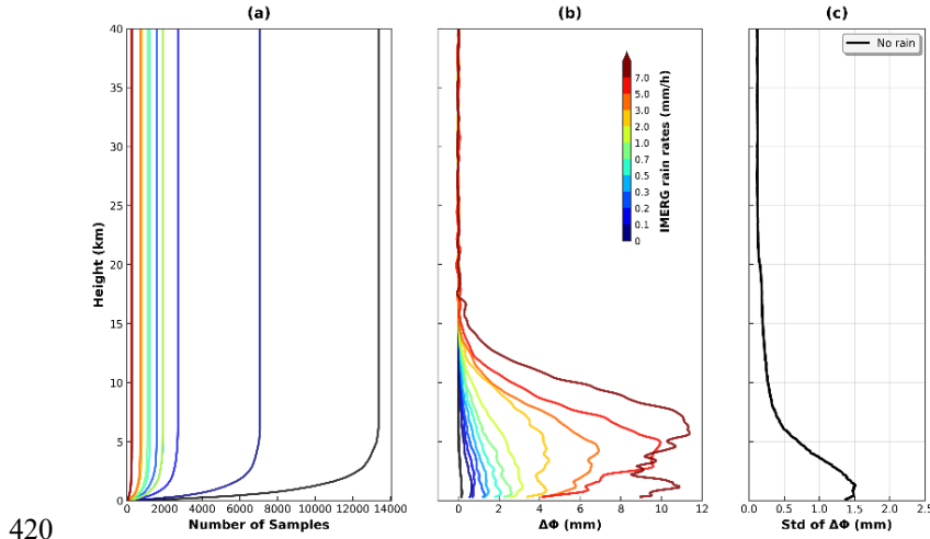
Figure 13. Statistical analysis of results over 0–40 km. (a) Sample size for each precipitation group; (b) Mean \Delta\Phi per precipitation group, with the black curve indicating the bias under non-precipitating conditions; (c) Standard deviation of the \Delta\Phi for the non-precipitation (0 mm h -1 ) group.
