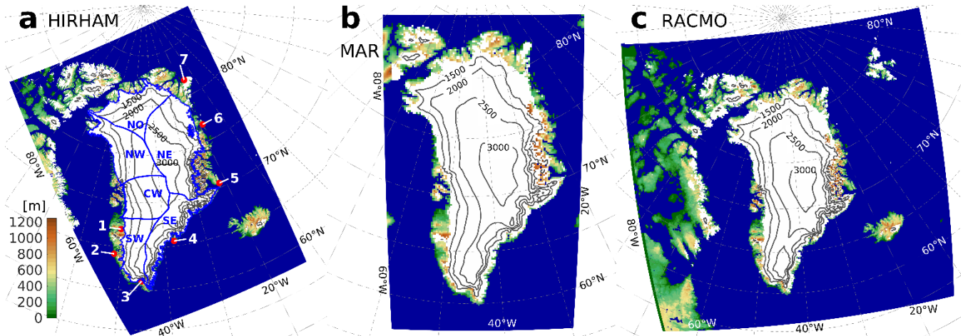
55 Figure 1: Model domain and orography for the HIRHAM (a), MAR (b) and RACMO (c) RCM simulations. Sea points are given in blue, glacier free land points in green/brown and glacier points in white with added surface elevation contour lines in black. The location of seven observational stations (red dots) and six drainage basins (blue contour lines; Rignot and Mouginot, 2012) are shown in panel a. The stations in order 1–7 are Kangerlussuaq, Nuuk, Narsarsuaq, Tasiilaq, Ittoqqortoormiit, Danmarkshavn and Station Nord.
