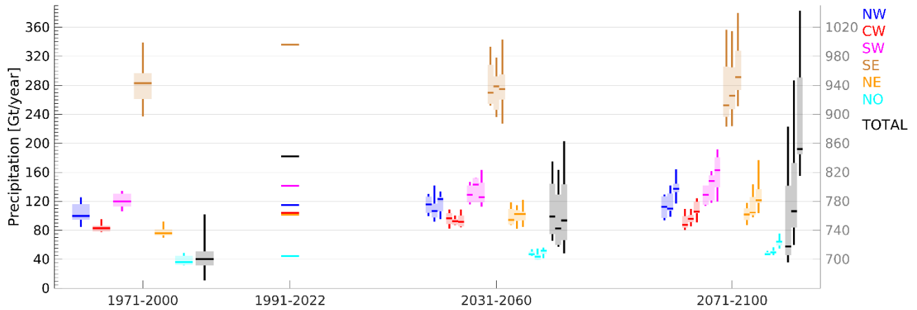
235 Figure 7: Mean precipitation (in Gt per year) for the RCM simulations over the six drainage basins and the full ice sheet for the historical period 1971–2000, for CARRA (1991–2022) and the scenario periods 2031–2060 and 2071–2100. The horizontal lines denote the ensemble median, the boxes represent the 25 th to 75 th percentiles while the vertical bars show the full model spread. For the two scenario periods the boxes are split into three segments: the left for SSP1-2.6, the middle for SSP2-4.5 and the right for SSP5-8.5. The y axis to the right is used for the full ice sheet (black) while the values for the six individual drainage basins are given by the y axis to the left.
