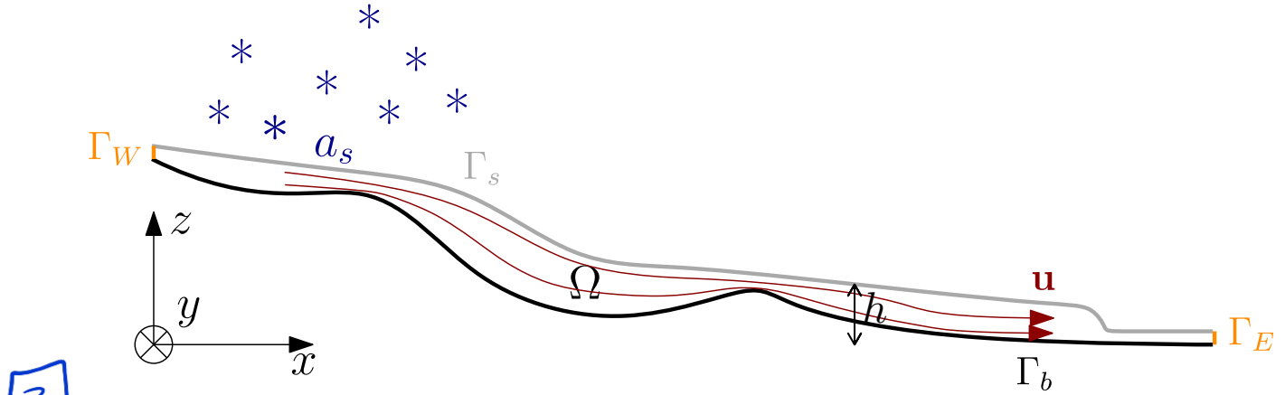
Figure 1. Illustration of a viscous free surface problem in the form of a mountain glacier. The ice is formed by accumulated snow and flows down the mountain due to the force of gravity. The surface height h indicates the distance from z = 0 to the surface \Gamma_s . Adapted from Löfgren et al. (2024), published in The Cryosphere , licensed under CC BY 4.0.
