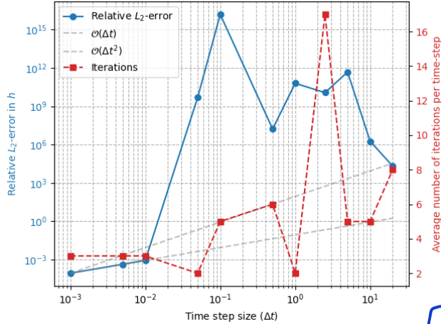
(c) Fully implicit solver, no FSSA. A maximum of 400 implicit iterations is permitted per time step. Error tolerance 1e-9 .
