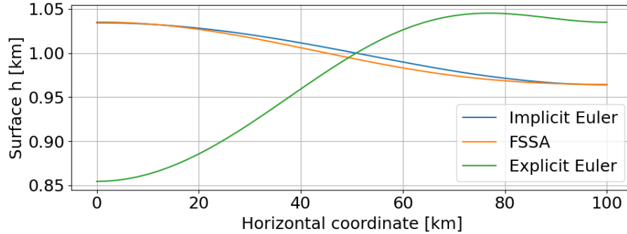
(b) \Delta t = 20 years
