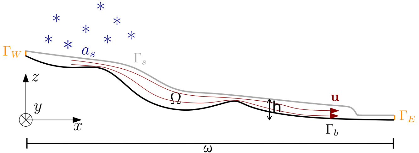
Figure 1. Illustration of a viscous free surface problem in the form of a mountain glacier. The ice is formed by accumulated snow and flows down the mountain due to the force of gravity. The surface height h indicates the distance from z = 0 to the surface \Gamma_s . The domain \omega is the projection of the full domain \Omega from \mathbb{R}^d to \mathbb{R}^{d-1} . The vertical position of the line |\text{---}| used to denote \omega is arbitrary chosen.. Adapted from Löfgren et al. (2024), published in The Cryosphere , licensed under CC BY 4.0.
