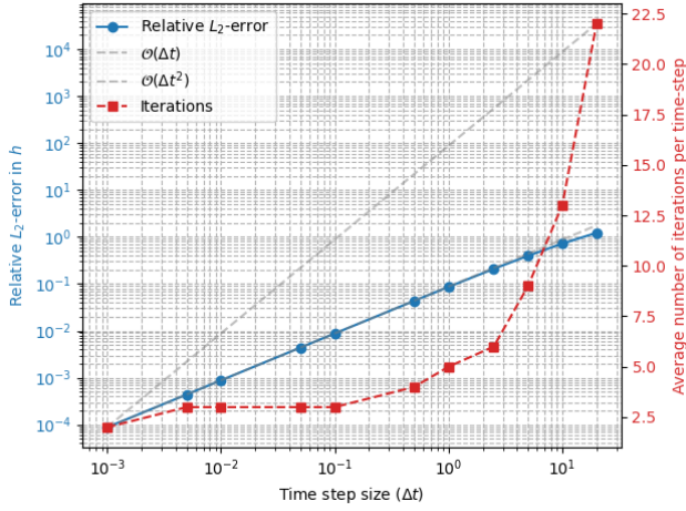
(a) Fully implicit BDF1 solver using the simplified stabilization of (23). A maximum of 100 implicit iterations is permitted per time step. Convergence tolerance 1e-9 .
