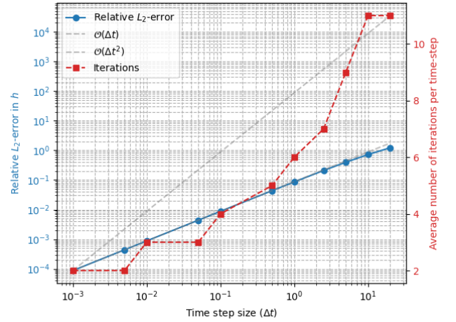
(d) Fully implicit solver. A maximum of 100 implicit iterations is permitted per time step. Convergence tolerance 1e-9 .
