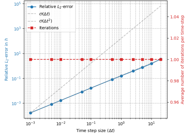
(b) Forward Euler for free surface, with FSSA ( \theta_1 = 1, \theta_2 = 1 ).
