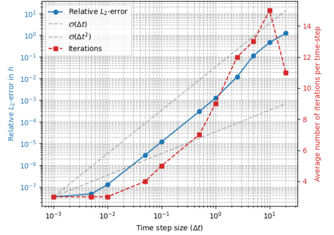
(b) Fully implicit BDF2-solver. A maximum of 100 implicit iterations is permitted per time step. Convergence tolerance 1e-9 .
