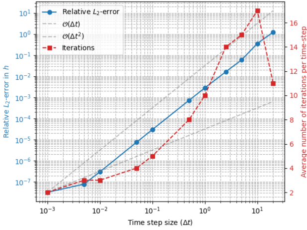
(a) Fully implicit Crank-Nicolson solver. A maximum of 100 implicit iterations is permitted per time step. Convergence tolerance 1e-9 .
