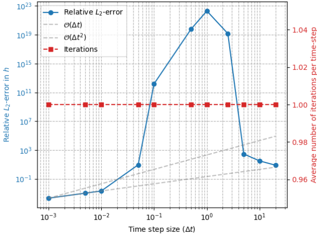
(a) Forward Euler for free surface, no FSSA. The very large errors for intermediate time-step sizes are due to high frequency oscillations. For the three largest time steps, the solution is smooth but erroneous.
