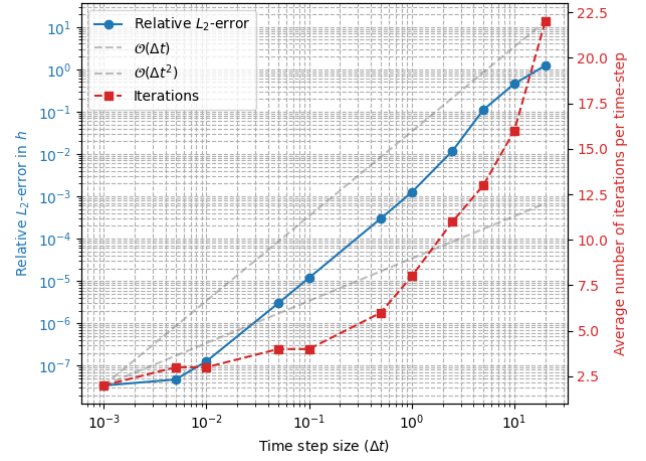
(b) Fully implicit BDF2-solver using the simplified stabilization of (23). A maximum of 100 implicit iterations is permitted per time step. Convergence tolerance 1e-9 .
