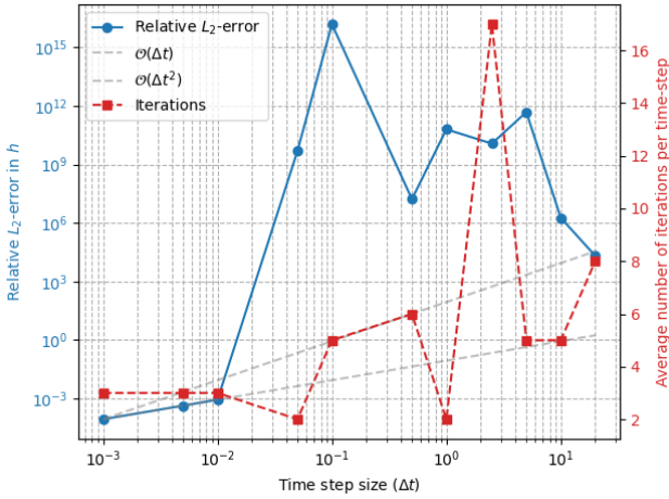
(c) Fully implicit solver, no FSSA. A maximum of 100 implicit iterations is permitted per time step. Convergence tolerance 1e-9 .
