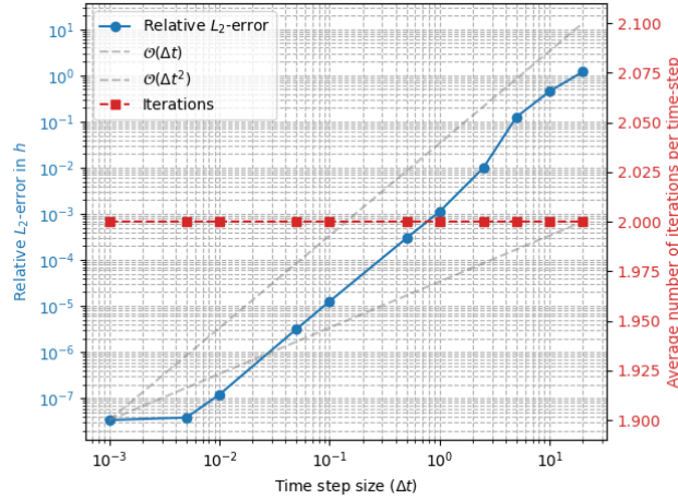
(c) Fully implicit BDF2-solver using the simplified stabilization of (23). A maximum of 100 implicit iterations is permitted per time step. Convergence tolerance 1e-9 .
