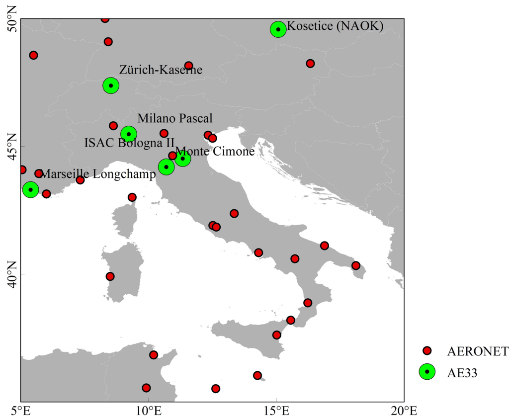
Figure 1. Location distribution of AERONET and AE33 ground observation stations. The small red dots, large green dots, 105 and text in the figure represent AERONET sites, AE33 sites, and AE33 site names, respectively.
