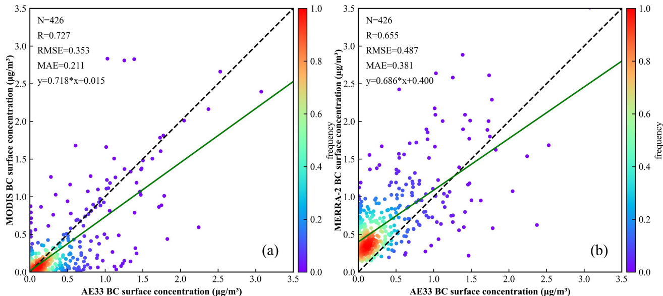
Figure 8. Scatter plot of MODIS BC and AE33 versus MERRA-2 BC and AE33. (a) and (b) represent MODIS BC and MERRA-2 BC, respectively. The black dashed line and the green solid line represent the 1:1 line and the linear regression function respectively.
