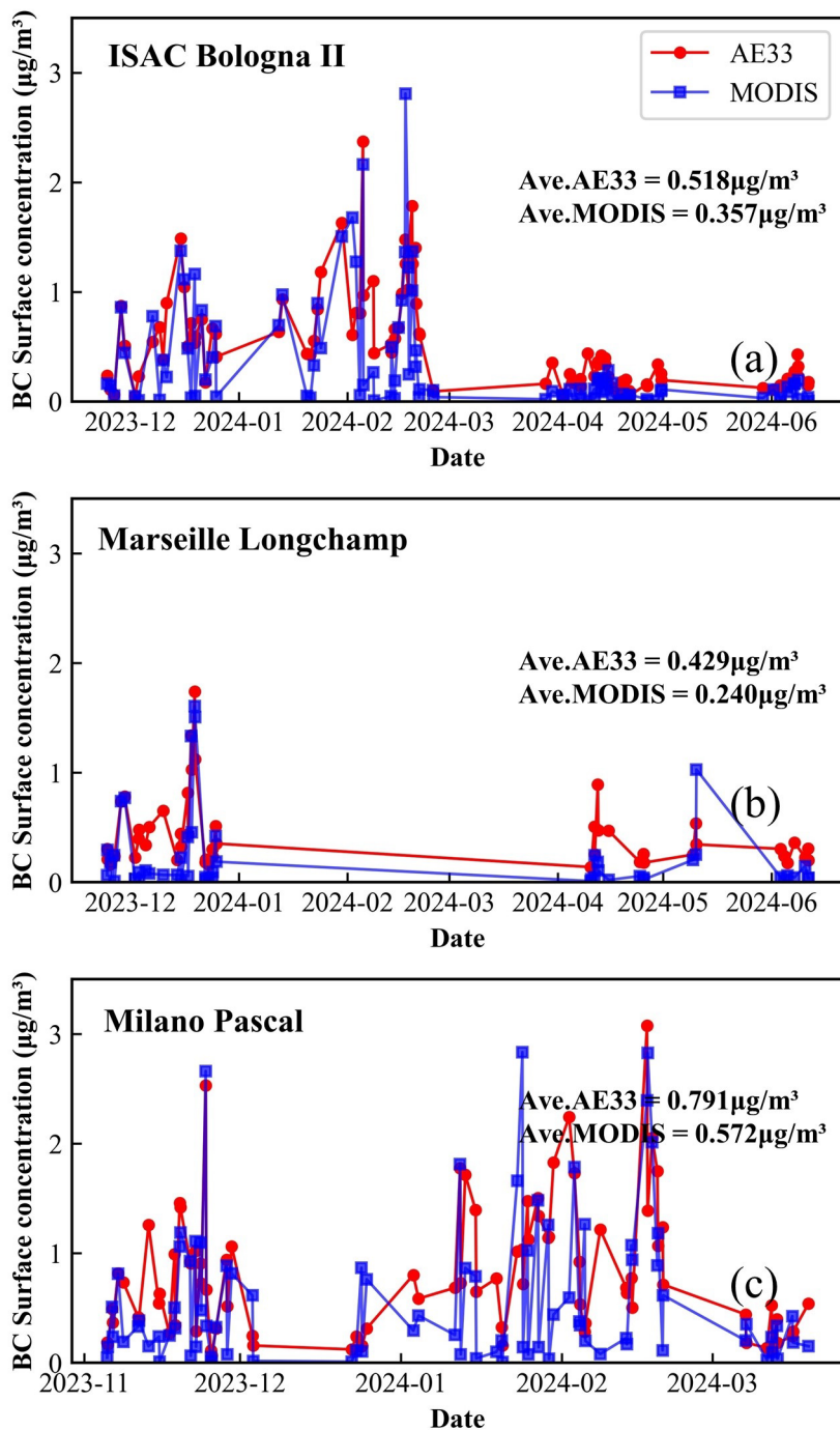
Figure 7. Comparison of consistency changes between MODIS BC and AE33 BC. (a), (b), and (c) represent ISAC Bologna II, Marseille Longchamp, and Milano Pascal, respectively.
