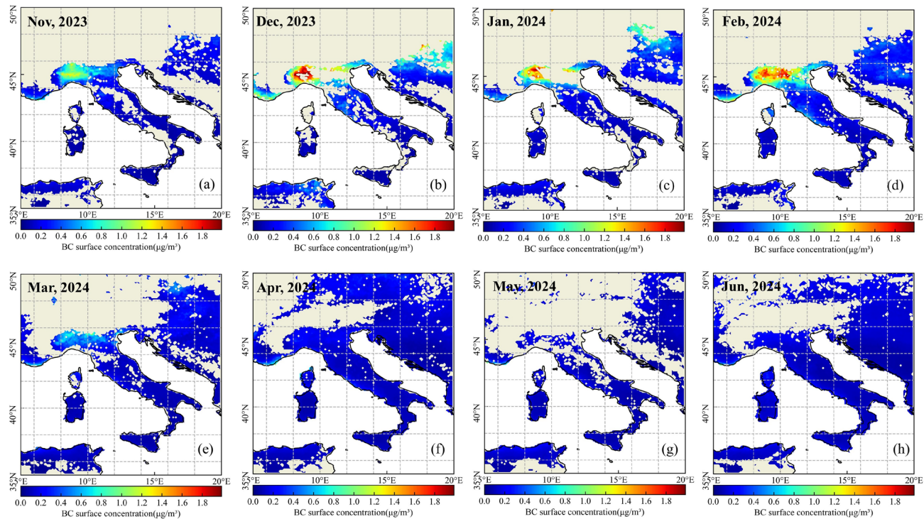
Figure 6. Maps of monthly BC surface concentration distribution. (a)-(h) respectively represent from November 2023 to June 2024.
