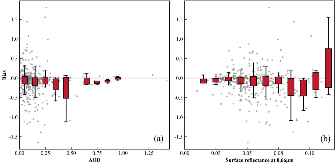
Figure 9. The box plot of BC surface concentration Bias (MODIS - AE33) independence analysis on the (a) AOD and (b) surface reflectance. The red box represents the interquartile range (IQR, 25th–75th percentiles), and the black whiskers extend to the most extreme data points within 1.5 \times \text{IQR} from the quartiles.
