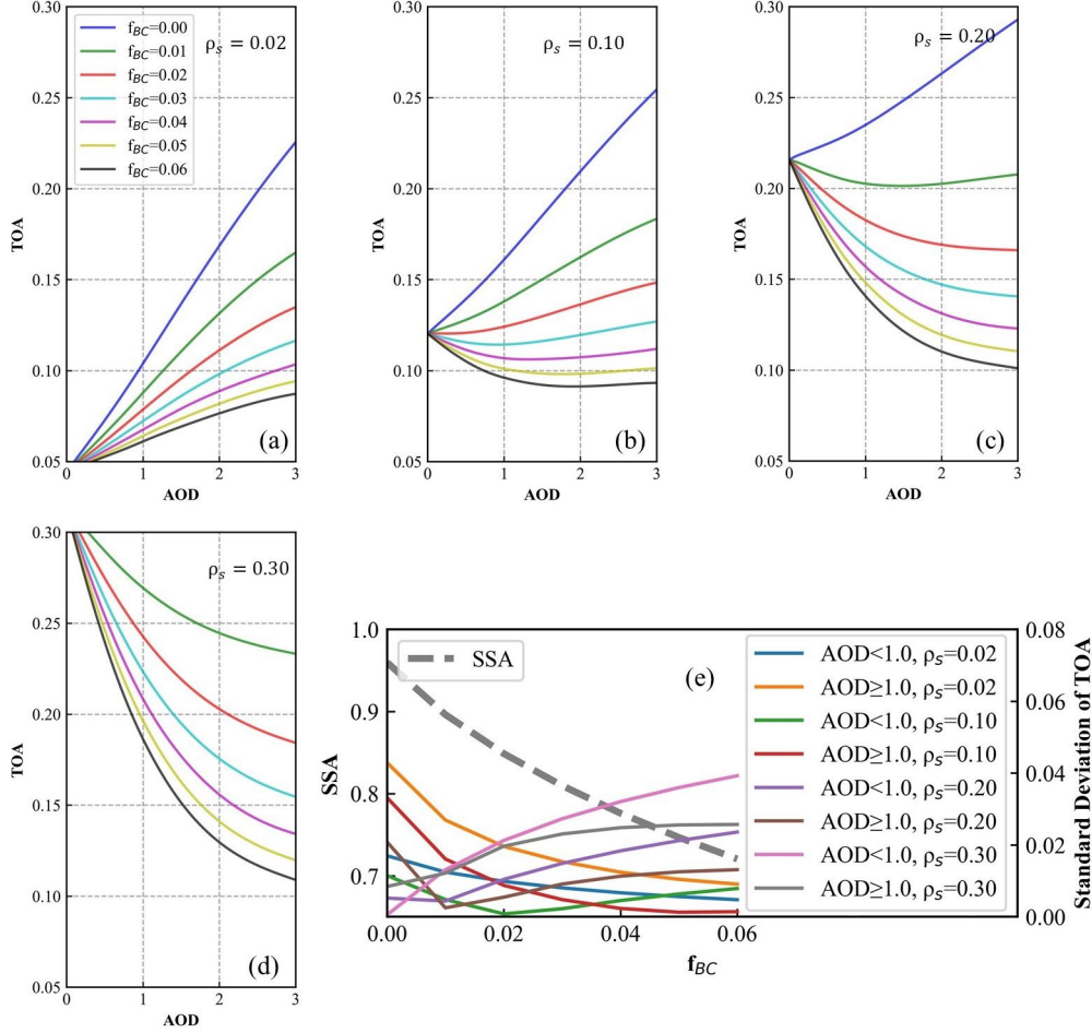
Figure 5. Sensitivity analysis of BC inversion based on 6SV2.1 model. The (a)-(d) represents the \rho_s at 0.66\mu\text{m} variation step sizes, which are 0.02, 0.10, 0.20, and 0.30, respectively. The (e) represents SSA and Standard deviation of TOA changes in different f_{BC} .
