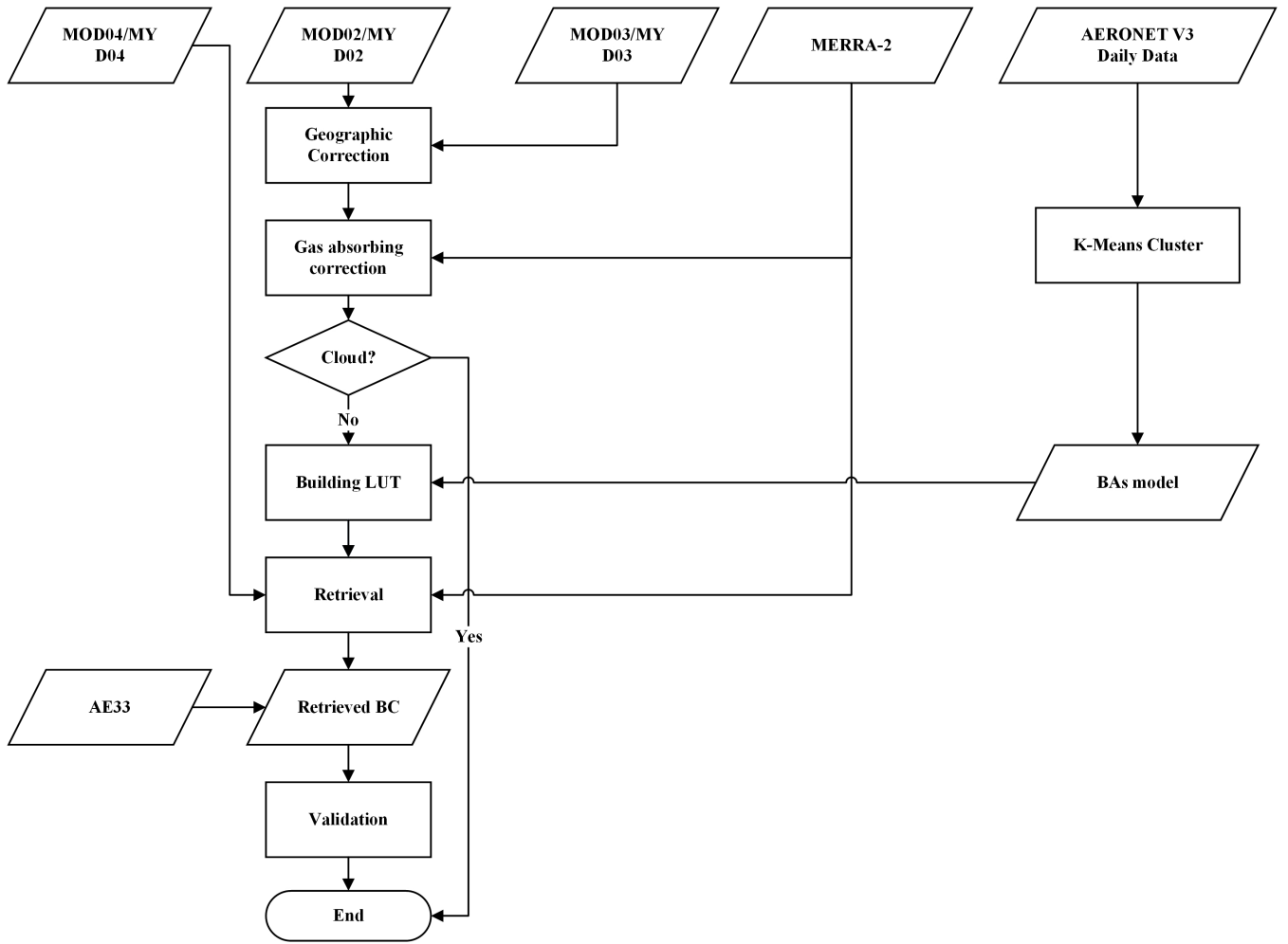
190 Figure 4. BC surface concentration retrieval algorithm workflow chart.
