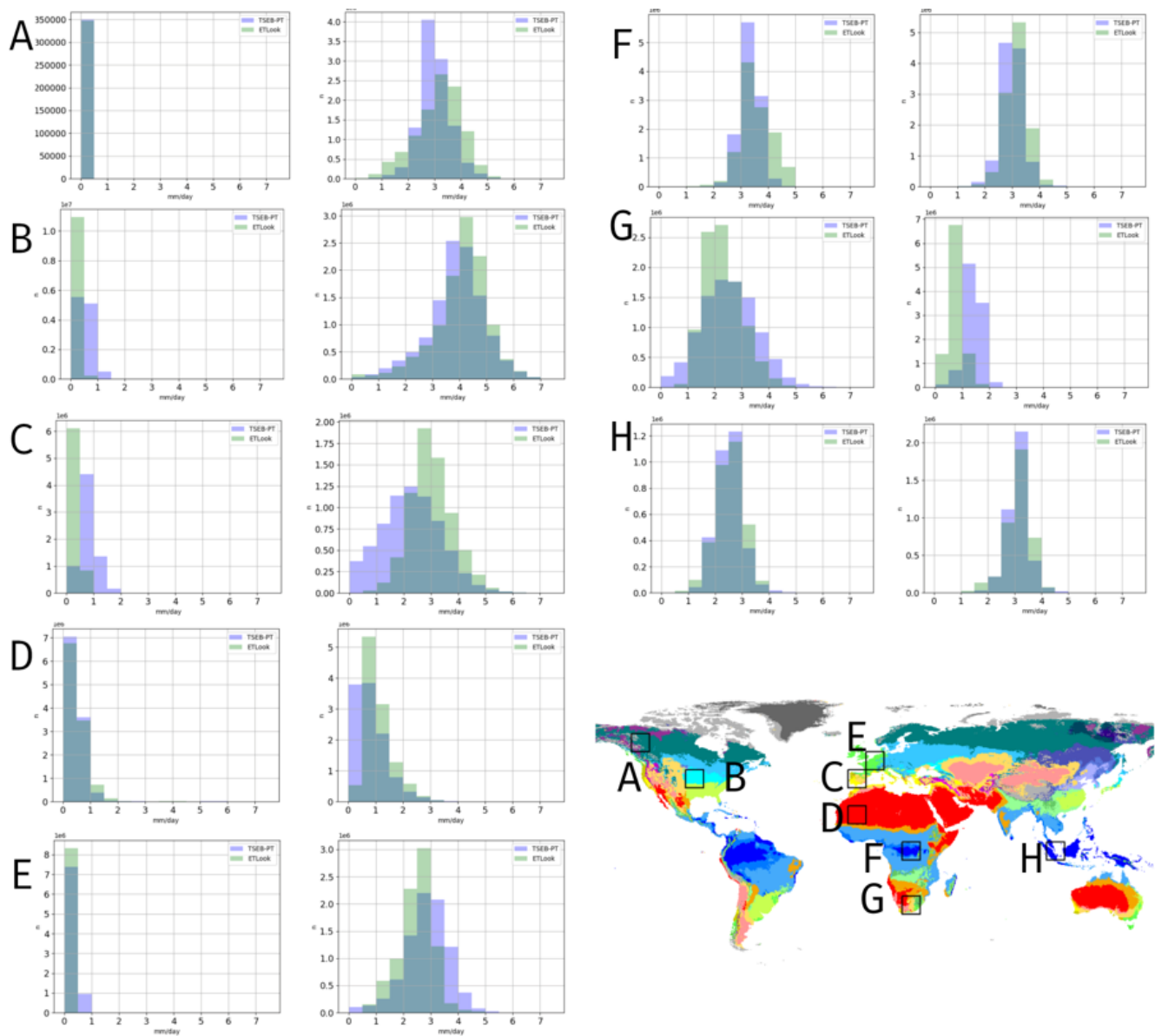
Figure C6. Histograms of TSEB-PT (blue) and ETLook (green) dekadal ET in first dekads of January (left panels) and of July (right panels) 2021 across 10° lat/lon tiles located in different climate regions according to the Köppen classification system. Climate types per region: A: Dfc; B: Dfa; C: mosaic of Csa, BSk, Csb, Cfb; D: BWh; E: Cfb; F: Af; G: mosaic of BWh, BSk, Cwb, Cfb; H: Af.
