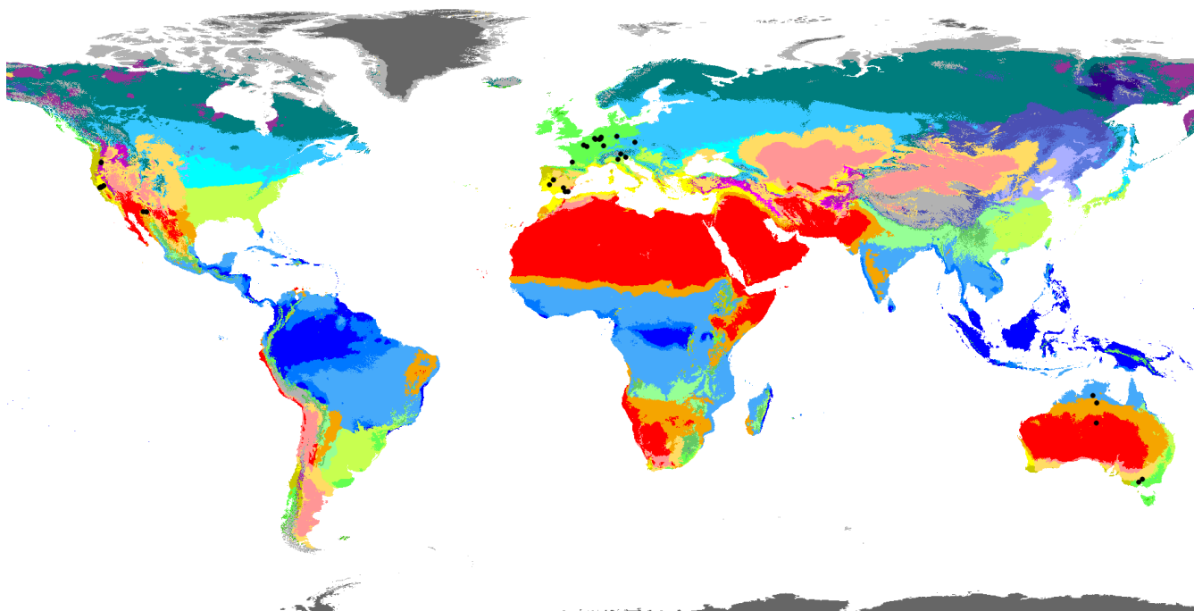
Figure C9. Location of sites used to evaluate CAMS meteorological data (Section 4.3.3). Background map shows Köppen climate classification
