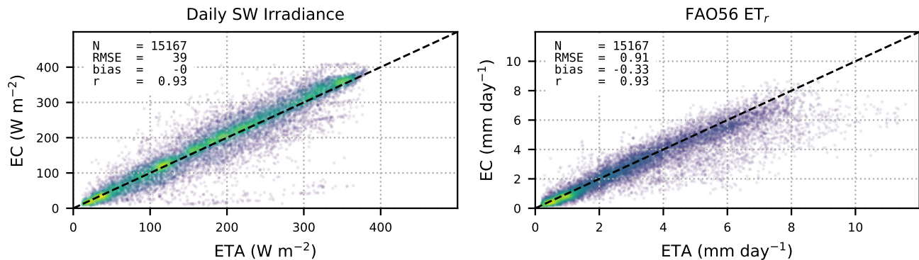
Figure 17. Comparison between daily solar irradiance (Daily SW Irradiance in \text{Wm}^{-2} ) and reference ET (FAO56 \text{ET}_r , panel in \text{mm day}^{-1} ) modelled with topographically corrected CAMS forecast data (x-axis) and measured (y-axis) in 43 representative Eddy Covariance stations located in western Europe, United States and Australia.
