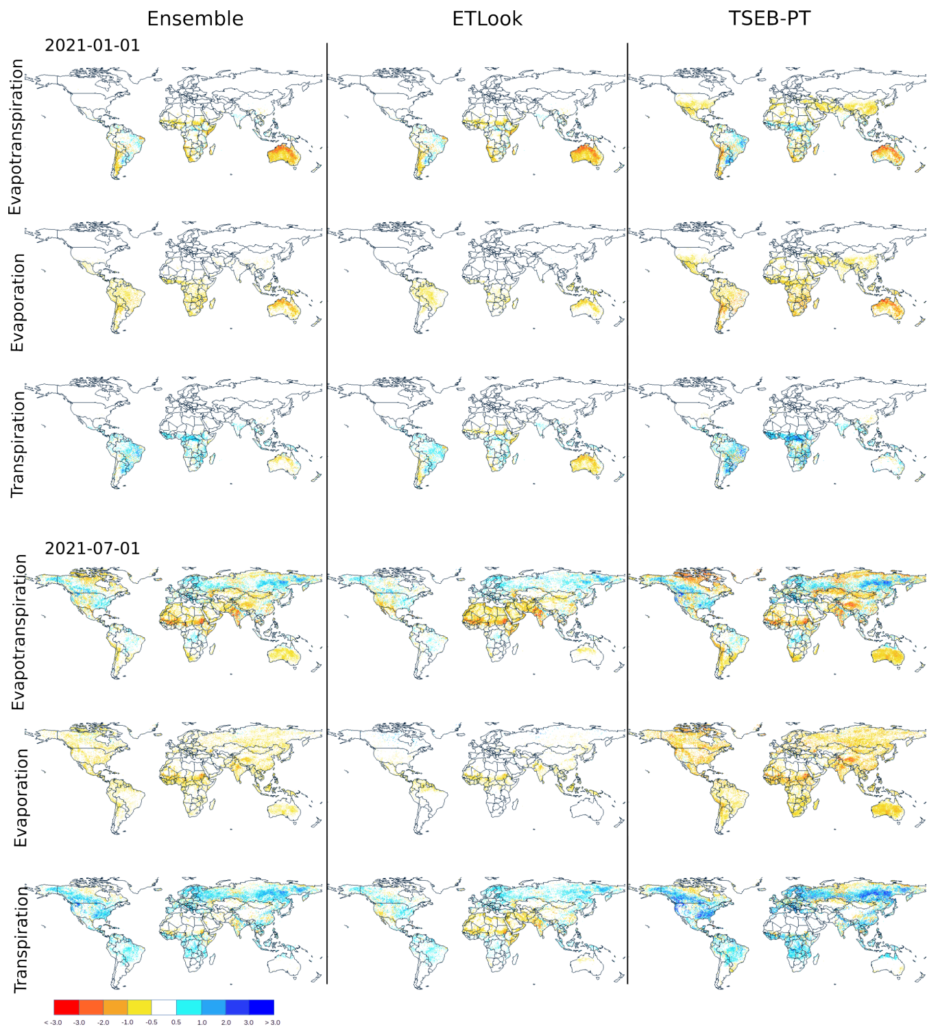
Figure C7. Differences (WapOR - CLMS: mm/day) between estimates of ET, E and T of the two products on the first dekad of January and July 2021.
