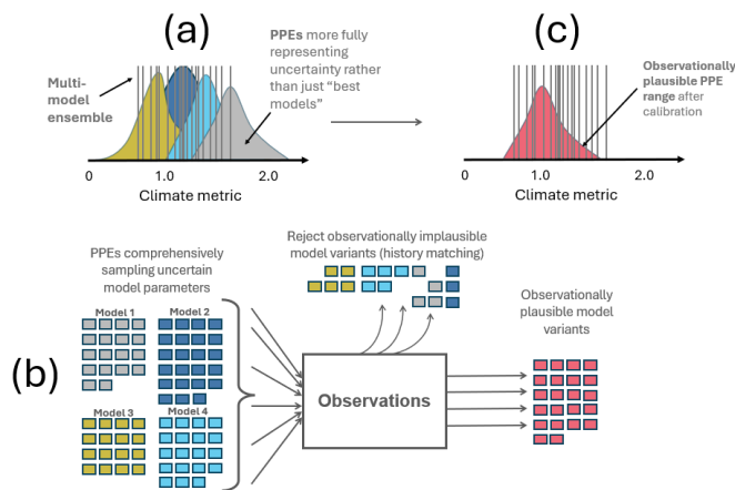
300 Figure 4. Schematic illustrating two aspects of PPEs. (a) PPEs more fully represent uncertainties than a multi-model ensemble (MME) of well-configured best estimates from several modelling centres. The MME (grey vertical lines) represents an unquantified mixture of structural differences, parametric uncertainties and internal variability, making it difficult to understand and ultimately reduce the spread in predictions or projections. PPEs (shown by pdfs) provide a way of cleanly separating structural and parametric uncertainty. (b) Statistically rigorous model calibration can be used to constrain the multi-model PPE range –shown in (c) – by defining a set of observationally plausible model
