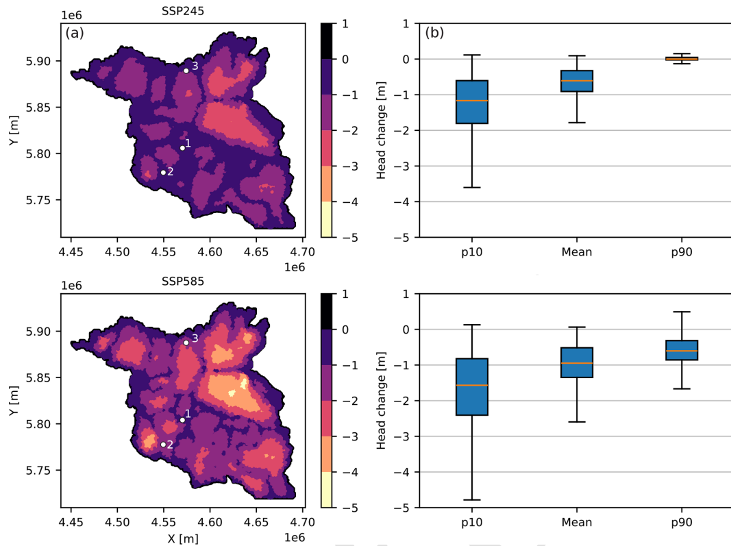
Figure 7. Projected changes in hydraulic heads between the present and late-century periods: (a) spatial distribution of head changes for the SSP ensemble mean; coordinates are shown in DHDN/3° Gauss-Krüger zone 4; labels refer to wells, shown in Fig. 6; (b) comparison of P10, mean, and P90 ranges.
