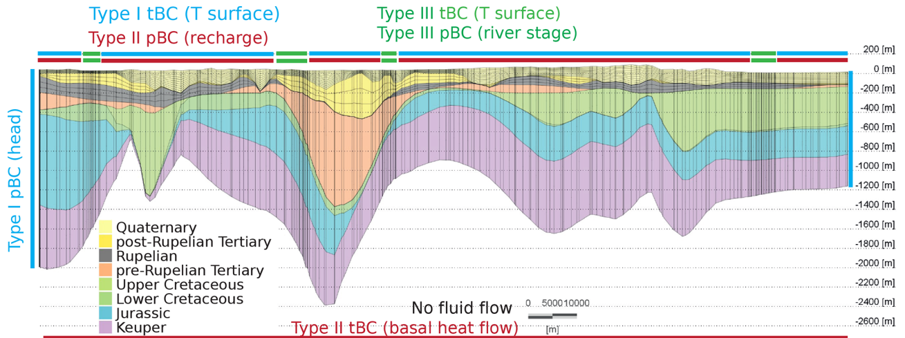
Figure 2. Layering and the setup of the hydraulic (pBC) and thermal (tBC) boundary conditions of the groundwater model. The location of the cross-section is shown in Fig. 1b.
