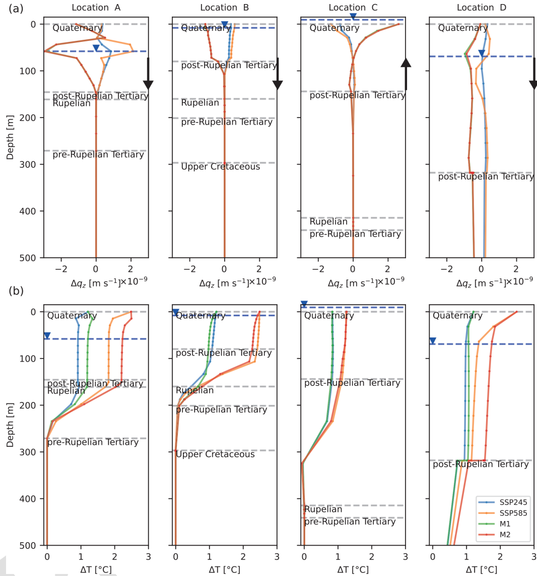
Figure 9. Changes in (a) vertical groundwater flux and (b) temperature vs. depth between the present and late-century periods. The scenario pairs SSP245/M1 and SSP585/M2 assume the same degrees of surface warming but decreasing/increasing groundwater recharge, respectively. The blue line indicates water table depth. The arrow shows the direction of vertical groundwater flow ( q_z vector is always oriented upward).
