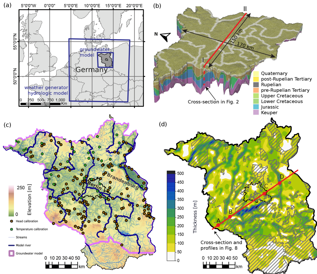
Figure 1. Overview of the study area: (a) geographical location and models' extent; (b) 3-D view of the groundwater model mesh; (c) topography of Berlin-Brandenburg and locations of the groundwater model calibration points; (d) thickness of the Quaternary unit. Dashed polygons indicate absence of the Rupelian aquitard.
