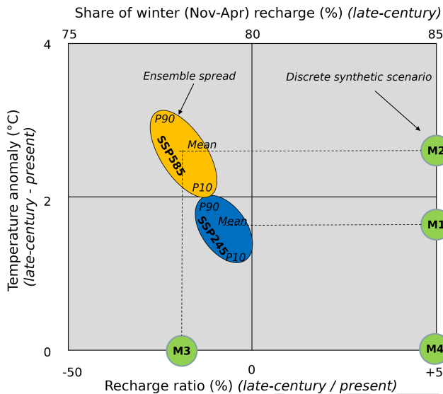
Figure 4. Schematic representation of the groundwater modeling scenarios. See Table 1 for the detailed description.
