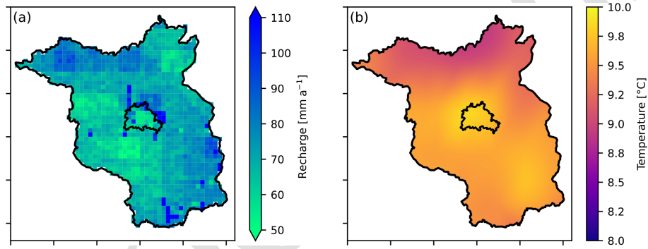
Figure A1. Variability of groundwater recharge and near-surface air temperature across the study area for the present period.
