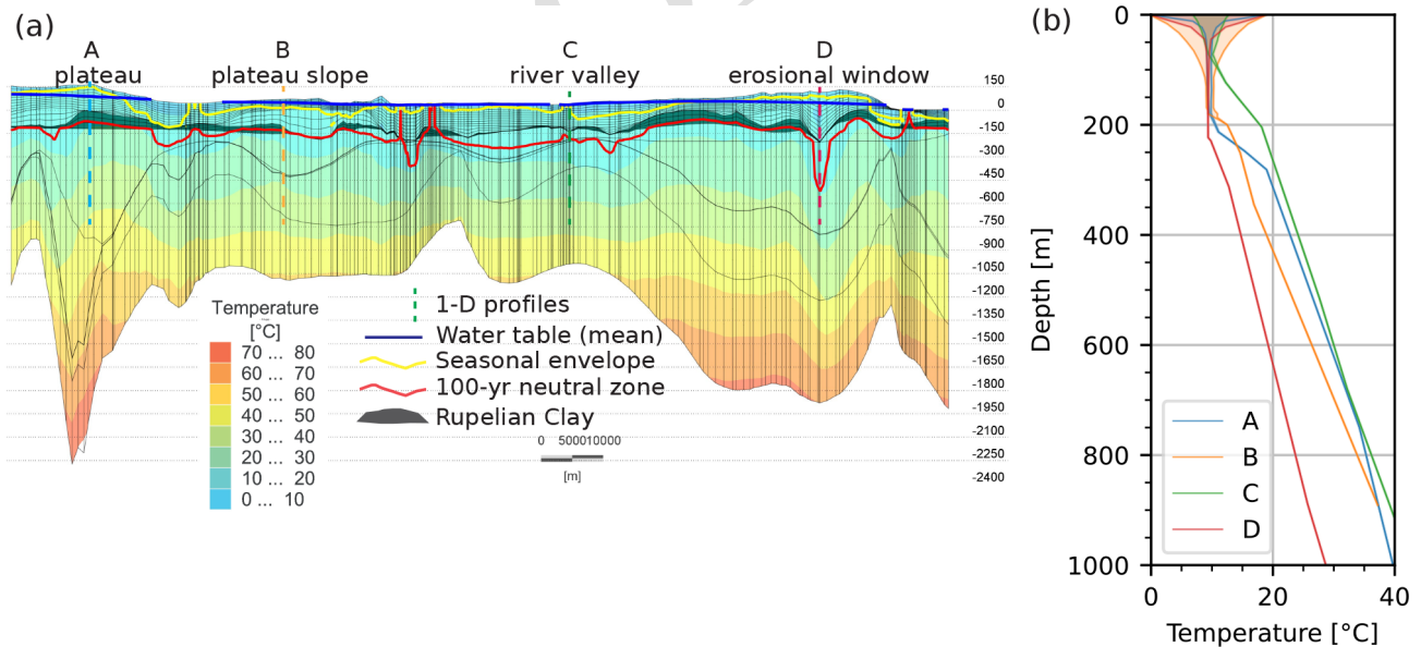
Figure 8. (a) cross-section of the initial subsurface thermal field, showing variability in the maximum depth of thermal disturbance (100 years neutral zone) and a seasonal envelope; (b) initial temperature profiles (lines) and seasonal envelopes (shaded areas). The location of the cross-section is shown in Fig. 1d.
