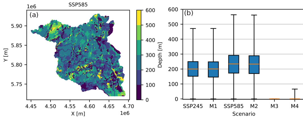
Figure 10. Depth to long-term steady groundwater temperatures: (a) spatial variability under SSP585; (b) comparison of the depth variability between scenarios. Scenarios M3 and M4 assume changes in recharge and constant surface temperatures.
