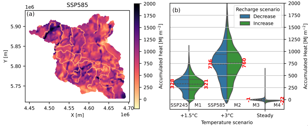
Figure 11. Accumulated heat-in-place: (a) map for scenario SSP585, (b) violin plots (equal-width-normalized) comparing probability distributions of accumulated heat-in-place per m 2 between the scenarios. Red labels indicate P50 values; black labels refer to model scenarios.
