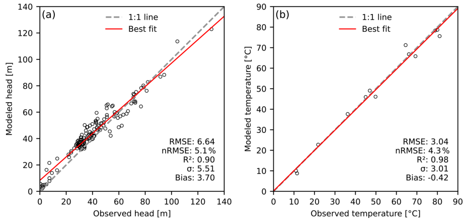
Figure 5. Steady-state groundwater model calibration results: simulated versus observed hydraulic head and temperature at monitoring points (locations shown in Fig. 1c). RMSE – Root Mean Square Error, nRMSE: normalized to value range; R^2 : coefficient of determination; \sigma : standard deviation.
