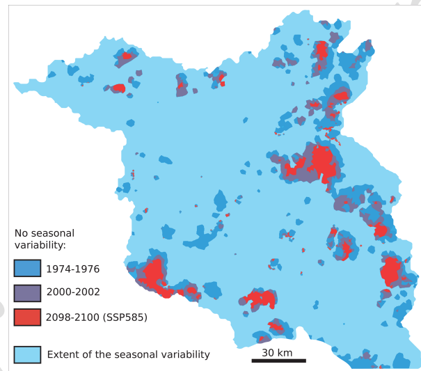
Figure A4. Extent of seasonal temperature damping at the water table during three periods. As a threshold for damping, we used a magnitude of temperature fluctuations < 1^{\circ}\text{C} .
