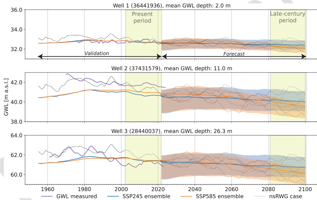
Figure 6. GWL time series for (a) shallow, (b) intermediate, and (c) deep monitoring wells (locations shown in Fig. 7a). Colored lines indicate ensemble mean, shaded areas represent P10–P90 range of the ensemble distribution, black lines are examples of individual nsRWG realizations. Numbers in brackets denote well ID from the state monitoring network (LfU, 2023).
