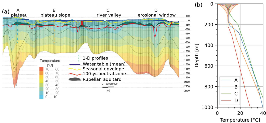
Figure 8: (a) cross-section of the initial subsurface thermal field, showing variability in the maximum depth of thermal disturbance (100-yr neutral zone) and a seasonal envelope; (b) initial temperature profiles (lines) and seasonal envelopes (shaded areas). The location of the cross-section is shown in Figure 1d.
