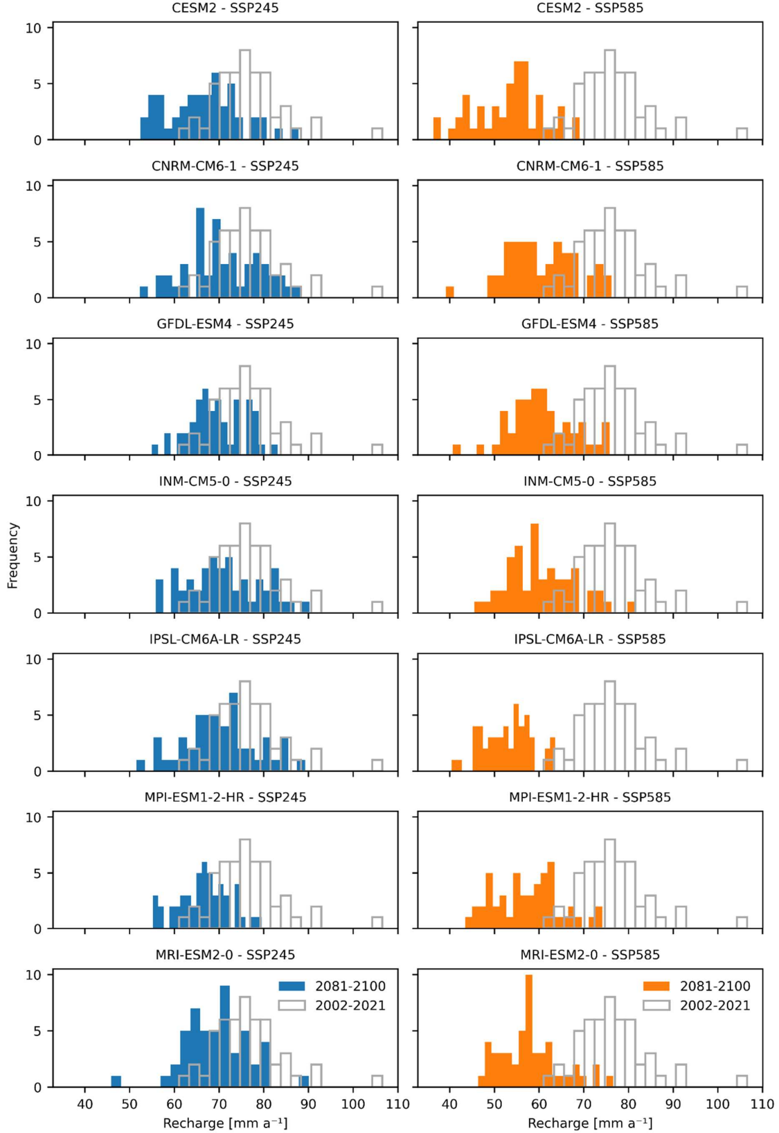
Figure A2: Histograms of mean annual recharge for Brandenburg, showing the distribution of 50 nsRWG realizations between the present and late-century periods for each GCM. Left: SSP245; right: SSP585.
