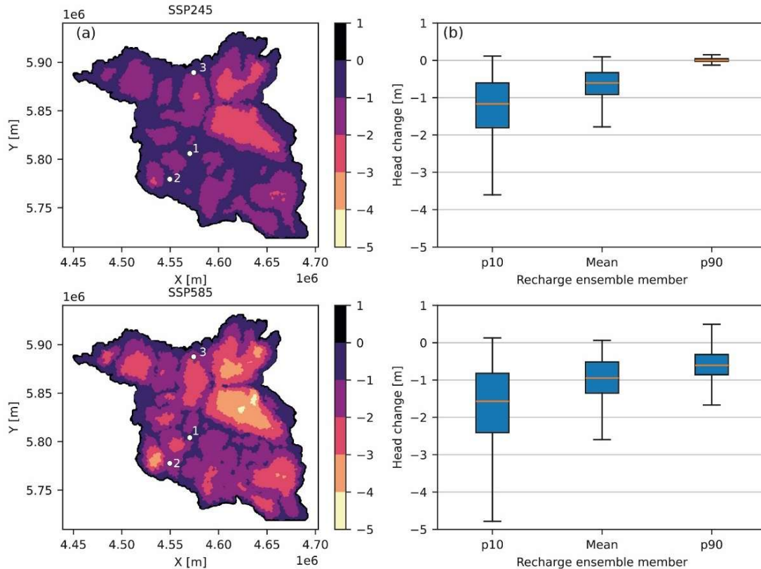
Figure 7: Projected changes in hydraulic heads between the present and late-century periods: (a) spatial distribution of head changes for the SSP ensemble mean; coordinates are shown in DHDN / 3-degree Gauss-Krüger zone 4 (EPSG:31468); labels refer to wells, shown in Figure 6; (b) comparison of P10, mean, and P90 ranges.
