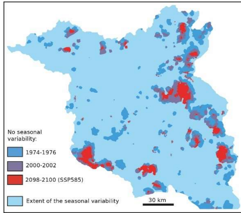
Figure A4: Extent of seasonal temperature damping at the water table during three periods. As a threshold for damping, we used a magnitude of temperature fluctuations <1^\circ\text{C} .
