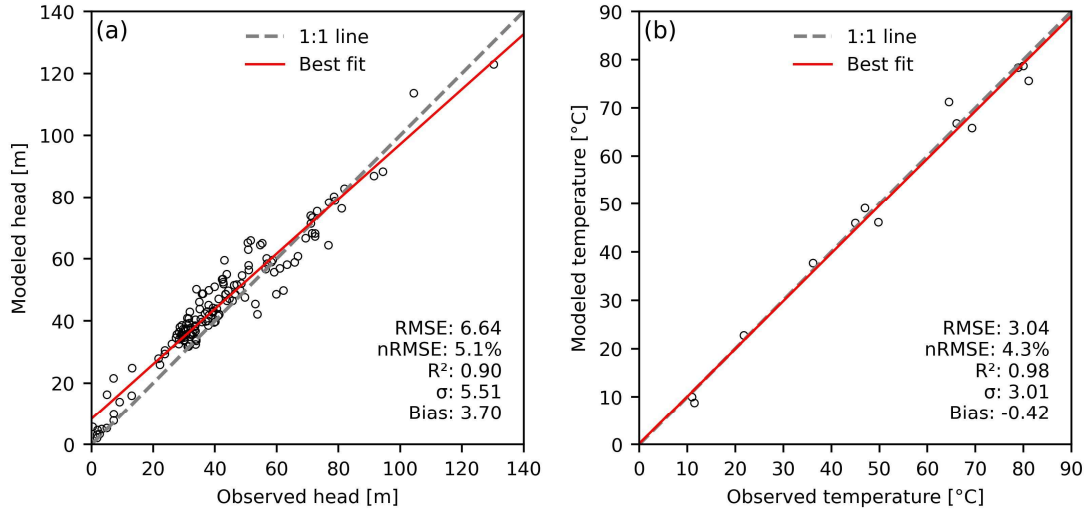
370 Figure 5: Steady-state groundwater model calibration results: simulated versus observed hydraulic head and temperature at monitoring points (locations shown in Figure 1c. RMSE – Root Mean Square Error, nRMSE – normalized to value range; R^2 – coefficient of determination; \sigma – standard deviation.
