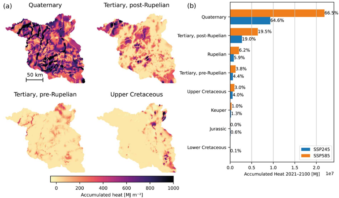
475 Figure 12: Accumulated heat by geological unit between the present and late-century periods: (a) maps for scenario SSP585, (b) comparison between SSP585 and SSP245 with percent labels indicating unit's contribution to the total accumulated heat.
