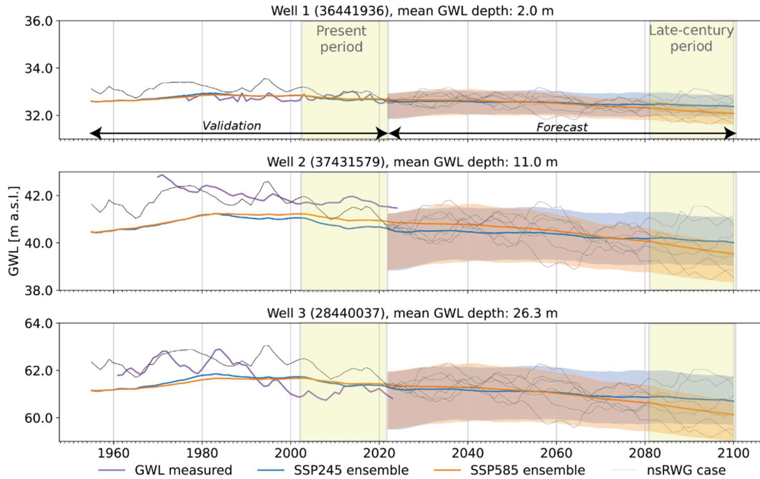
375 Figure 6: GWL time series for (a) shallow, (b) intermediate, and (c) deep monitoring wells (locations shown in Figure 7a). Colored lines indicate ensemble mean, shaded areas represent P10-P90 range of the ensemble distribution, black lines are examples of individual nsRWG realizations. Numbers in brackets denote well ID from the state groundwater monitoring network (LfU, 2023).
