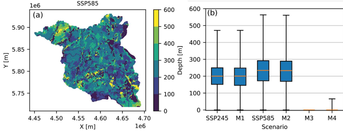
450 Figure 10: Depth to long-term steady groundwater temperatures: (a) spatial variability under SSP585; (b) comparison of the depth variability between scenarios. Scenarios M3 and M4 assume changes in recharge and constant surface temperatures.
