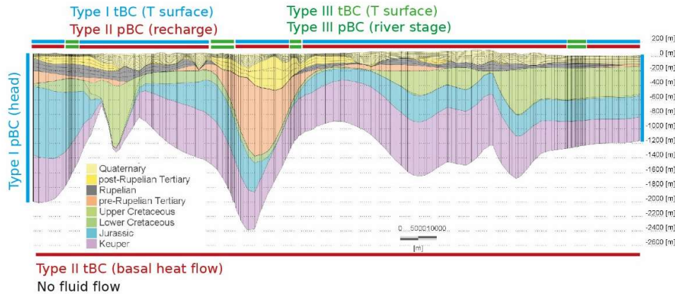
Figure 2: Layering and the setup of the hydraulic (pBC) and thermal (tBC) boundary conditions of the groundwater model. The location of the cross-section is shown in Figure 1b.
