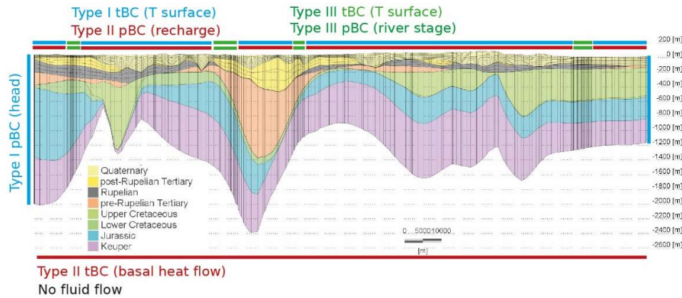
Figure 2: Layering and the setup of the hydraulic (pBC) and thermal (tBC) boundary conditions of the groundwater model. The location of the cross-section is shown in Figure 1b.
