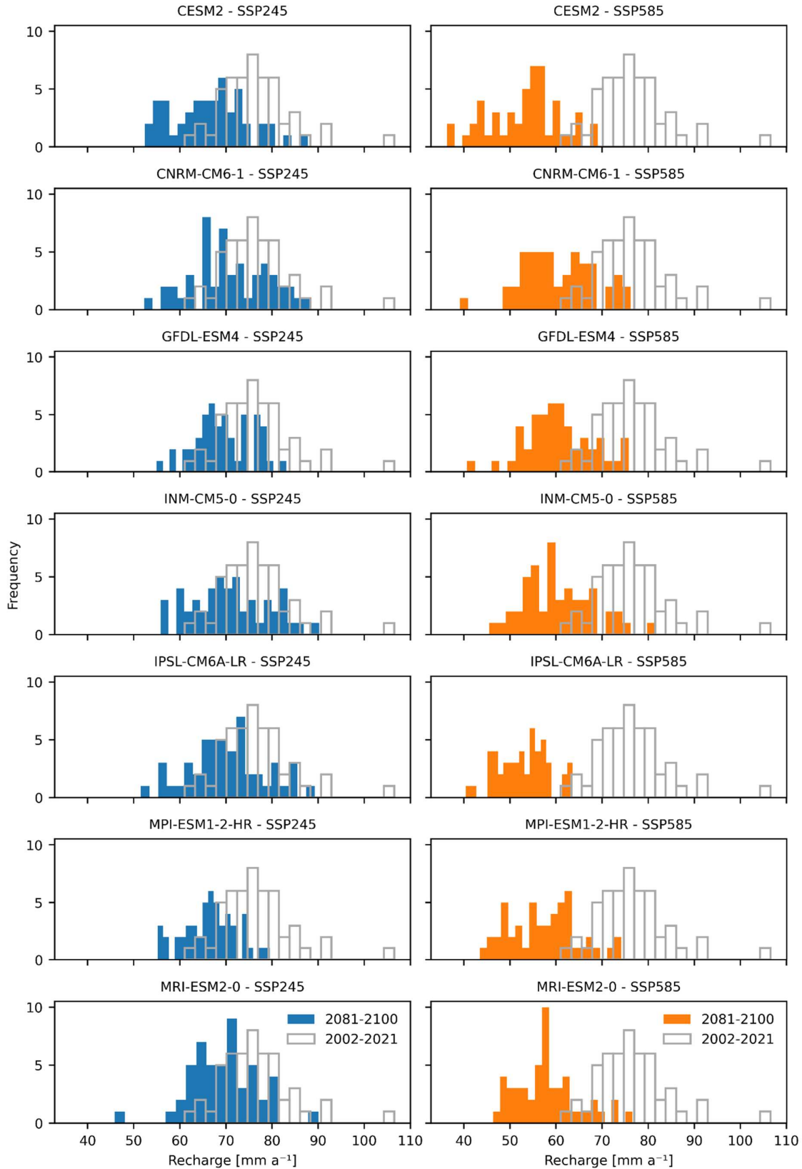
725 Figure A2: Histograms of mean annual recharge for Brandenburg, showing the distribution of 50 nsRWG realizations between the present and late-century periods for each GCM. Left: SSP245; right: SSP585.
