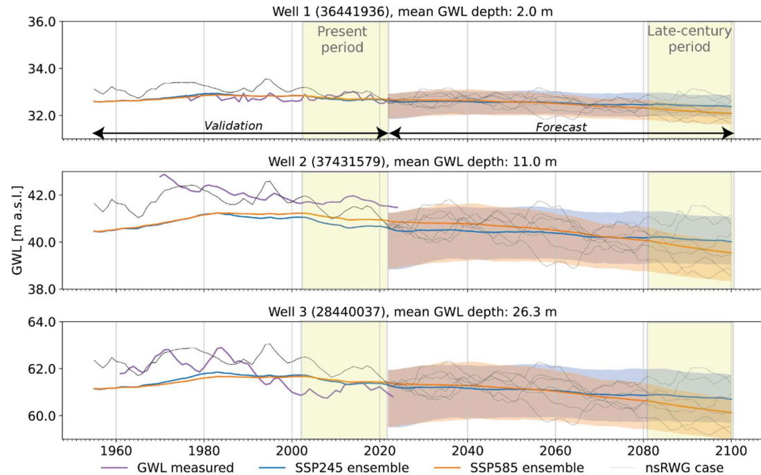
Figure 6: GWL time series for (a) shallow, (b) intermediate, and (c) deep monitoring wells (locations shown in Figure 7a). Colored lines indicate ensemble mean, shaded areas represent P10-P90 range of the ensemble distribution, black lines are examples of individual nsRWG realizations. Numbers in brackets denote well ID from the state groundwater monitoring network (LfU, 2023).
