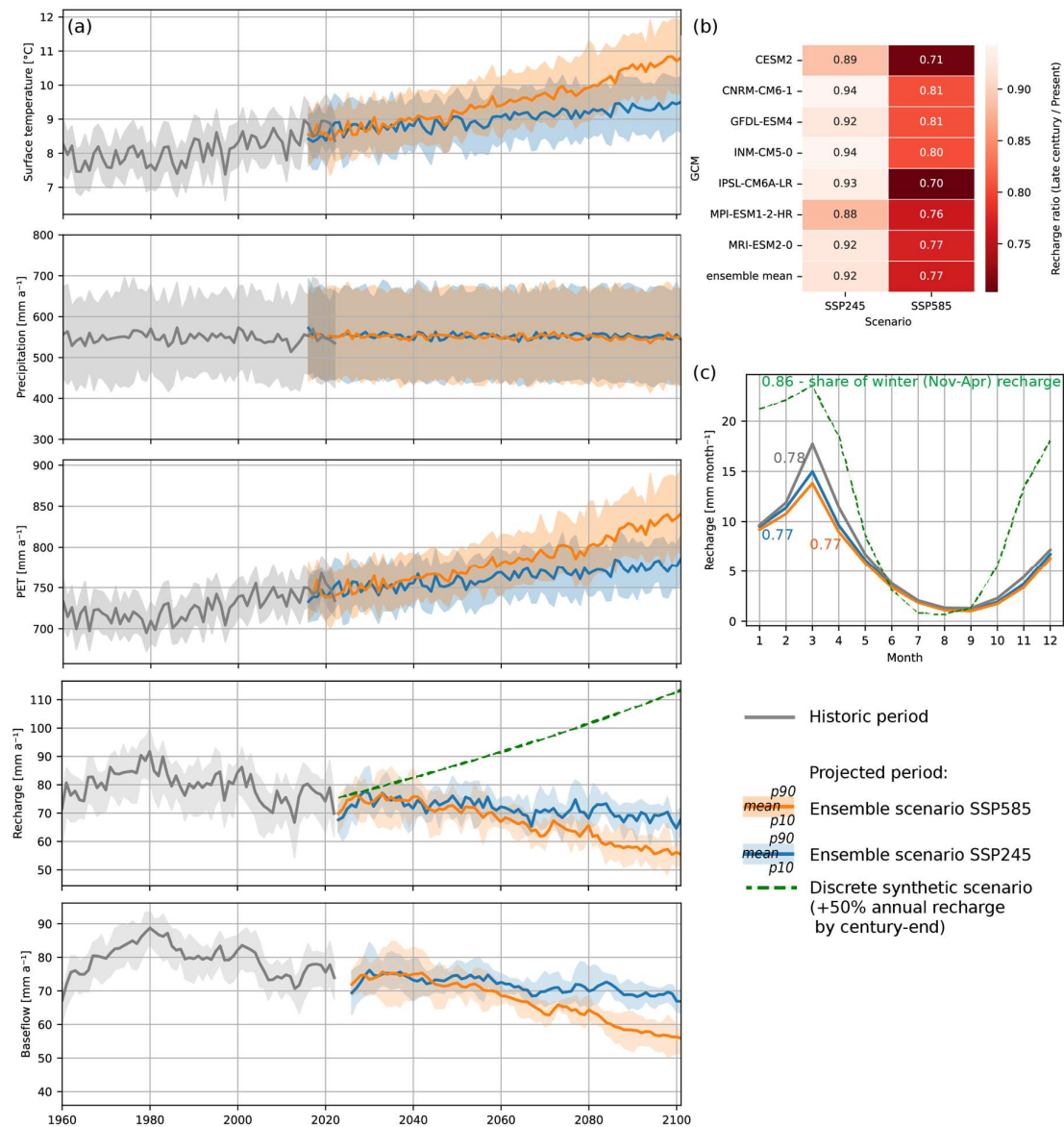
Figure 3: (a) historical and projected annual time series of surface temperature, precipitation, and groundwater recharge, and baseflow. Solid lines represent the ensemble mean (historical: across nsRWG realizations; SSP scenarios:
