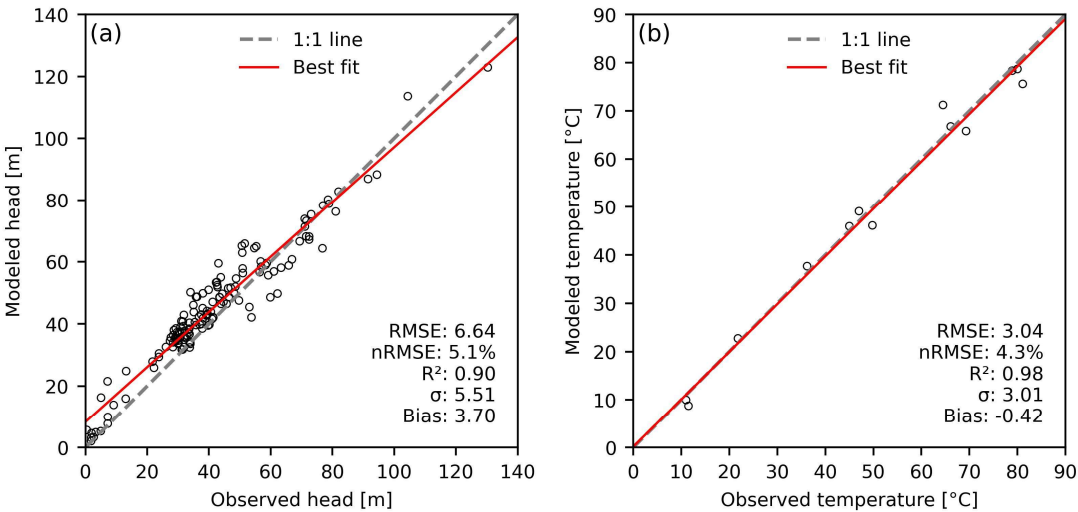
Figure 5: Steady-state groundwater model calibration results: simulated versus observed hydraulic head and temperature at monitoring points (locations shown in Figure 1c. RMSE – Root Mean Square Error, nRMSE – normalized to value range; R² – coefficient of determination; σ – standard deviation.
