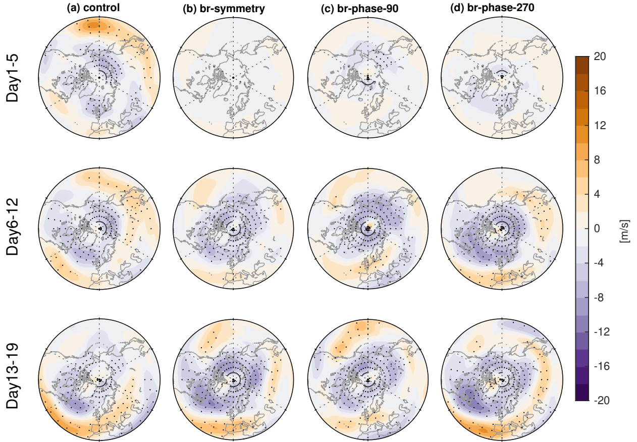
Figure 10. Zonal wind anomalies at 321 hPa during days 1 to 19 for (a) control run, (b) symmetric-branch symmetry ensemble, (c) phase-90 ensemble, and (d) phase-270 ensemble. Stippling indicates statistically significant anomalies at the 95% level based on Student's t test.
