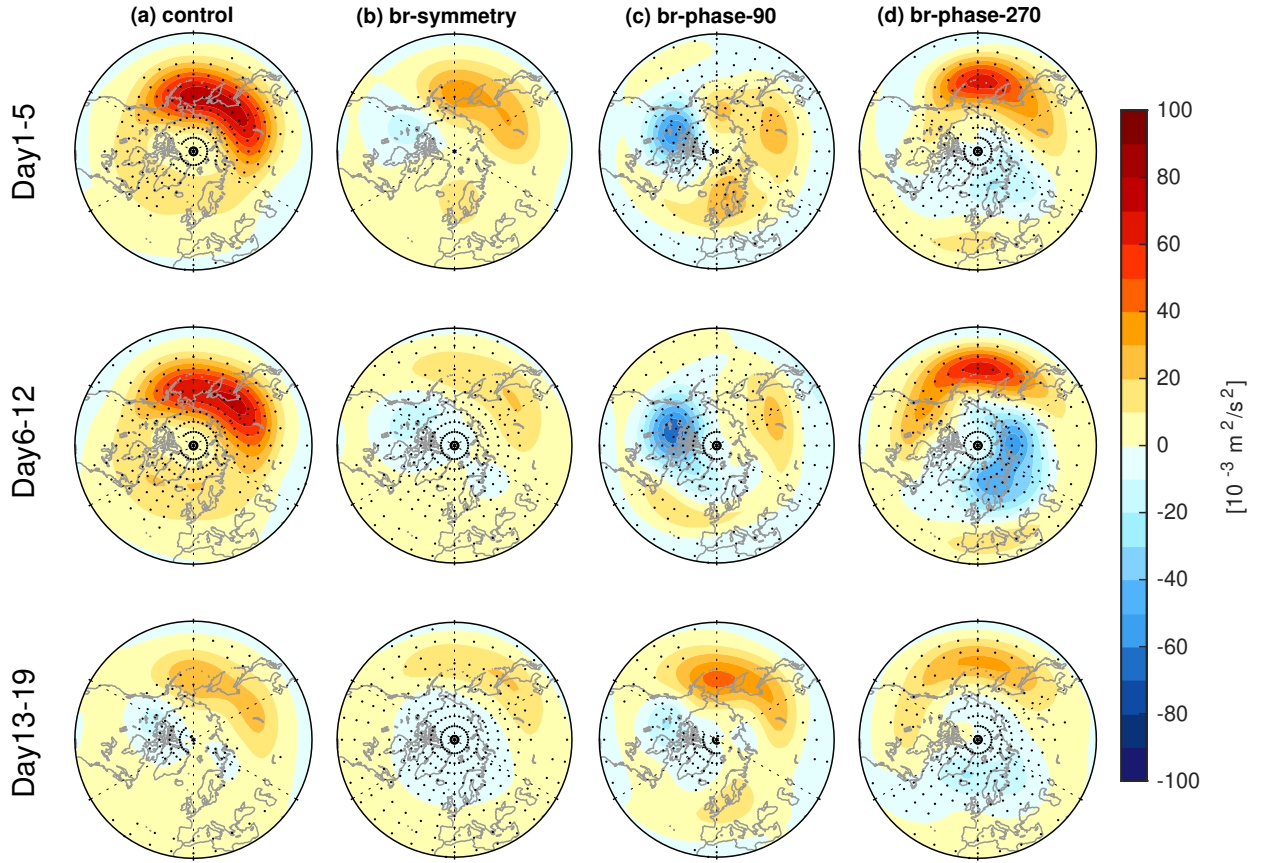
Figure 7. F_z (raw field) at 93 hPa during days 1 to 19 for (a) control run, (b) symmetric-branch-symmetry ensemble, (c) phase-90 ensemble, and (d) phase-270 ensemble. Stippling indicates the raw values are statistically significantly different from the climatologies (not shown) at the 95% level based on Student's t test.
