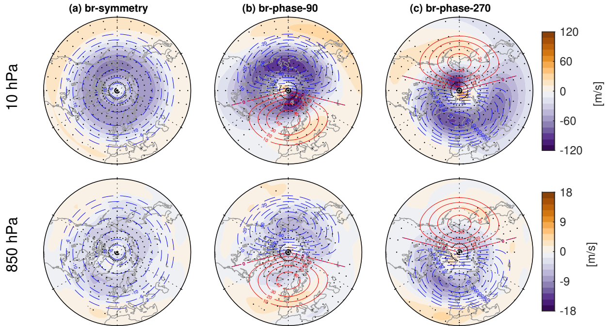
Figure 1. Zonal wind anomalies (shading; \text{m s}^{-1} ) at 10 hPa (upper row) and 850 hPa (bottom row) during averaged over days 6 to 12 for (a) symmetric-branch-symmetry ensemble, (b) phase-90 branch ensemble, and (c) phase-270 branch ensemble. The blue dashed (red solid) contour indicates the applied negative (positive) wave forcing (contours; \text{m s}^{-1} \text{ day}^{-1} ) at 10 hPa. The contour interval for wave forcing is 4 \text{ m s}^{-1} \text{ day}^{-1} in (a) and 10 \text{ m s}^{-1} \text{ day}^{-1} in (b) and (c). Stippling indicates anomalies that are statistically significant at the 95% level based on Student's t test. Note that the forcing is applied only above 100 hPa but displayed at 850 hPa for visual comparison.
