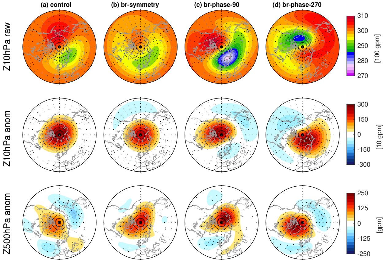
Figure 2. Geopotential height raw fields at 10 hPa (upper row) and anomalies at 10 hPa and 500 hPa (middle and bottom rows) during averaged over days 6 to 12 for (a) control run, (b) symmetric-branch-symmetry ensemble, (c) phase-90 ensemble, and (d) phase-270 ensemble. Stippling indicates that anomalies at 10 hPa and 500 hPa (middle and bottom rows) are statistically significant at the 95% level, while raw fields at 10 hPa (upper row) are statistically significantly different from the climatologies (not shown) at the 95% level, both - all based on Student's t test.
