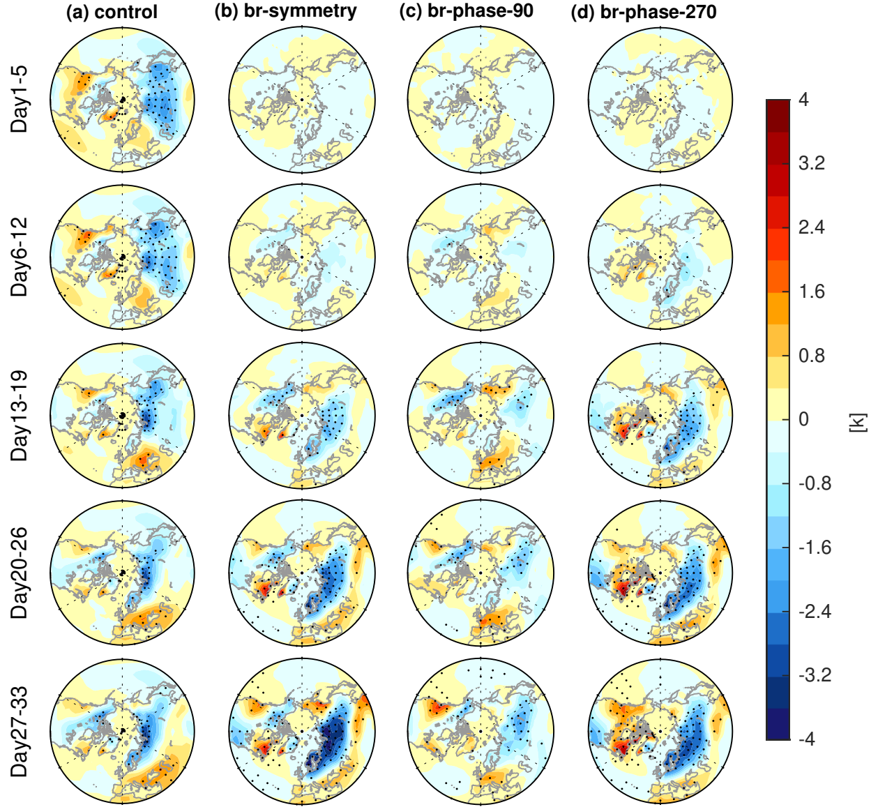
Figure 4. Temporal evolution of 2-m temperature anomalies during days 1 to 33 for (a) control run, (b) symmetric branch symmetry ensemble, (c) phase-90 branch ensemble, and (d) phase-270 branch ensemble. Stippling indicates statistically significant anomalies at the 95% level based on Student's t test. Recall that the forcing in the branch ensembles is applied only from days 1 to 12 and is switched off from day 13 onward. Hence, we show the response from days 1 to 5 and from days 6 to 12 during the forcing stage, and weeks from day 13 onward during the recovery stage.
