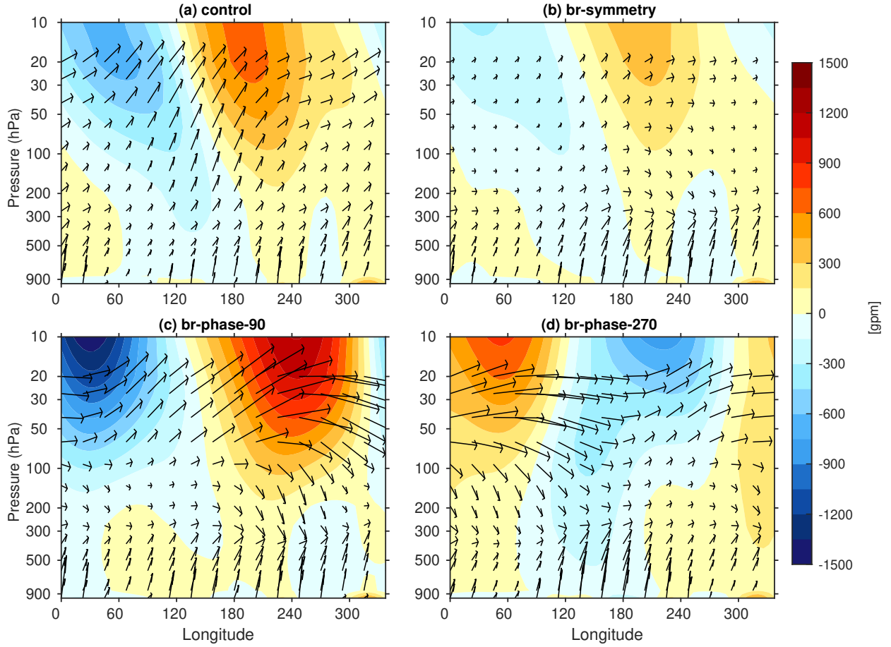
Figure 6. Longitude-pressure cross section of raw F_x and F_z (arrows) and raw geopotential height eddy (shading; remove deviation from the zonal mean) area averaged between 55^\circ\text{N} and 80^\circ\text{N} during averaged over days 6 to 12 for (a) control run, (b) symmetric-branch symmetry ensemble, (c) phase-90 ensemble, and (d) phase-270 ensemble.
