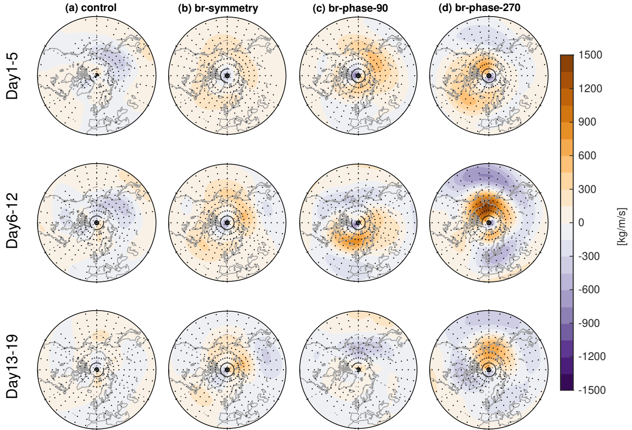
Figure 8. Mass streamfunction (derived from divergent part - component of meridional wind) anomalies pressure-weighted over 34-10 hPa during days 1 to 19 for (a) control run, (b) symmetric-branch - symmetry ensemble, (c) phase-90 ensemble, and (d) phase-270 ensemble. Stippling indicates statistically significant anomalies at the 95% level based on Student's t test. Based on the conventions in section 3, positive anomalies indicate poleward meridional flow, and negative anomalies indicate equatorward flow.
