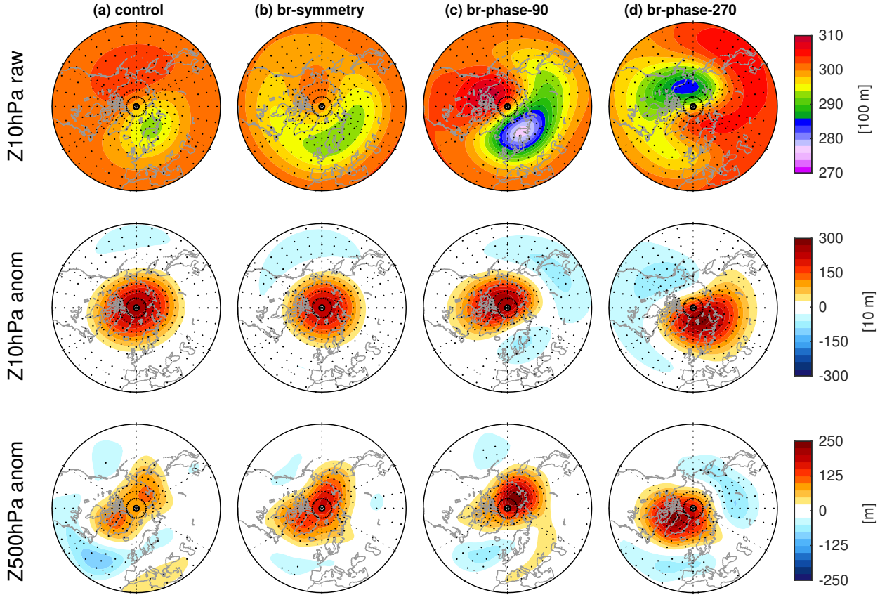
Figure 2. Geopotential height raw fields at 10 hPa (upper row) and anomalies at 10 hPa and 500 hPa (middle and bottom rows) during days 1 to 12 for (a) control run, (b) symmetric branch ensemble, (c) phase-90 ensemble, and (d) phase-270 ensemble. Stippling indicates that anomalies at 10 hPa and 500 hPa (middle and bottom rows) are statistically significant at the 95% level, while raw fields at 10 hPa (upper row) are statistically significantly different from the climatologies (not shown) at the 95% level, both based on Student's t test.
