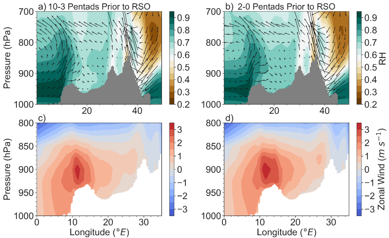
Figure 8: Relative humidity (shades) and vectors of u and \omega \cdot 10^2 for (a) 10-3 pentads prior to the spring RSO; (b) 2-0 pentads prior to the spring RSO. Zonal wind ( u ) for (c) 10-3 pentads prior to the spring RSO; (d) 2-0 pentads prior to the spring RSO. Grey shading in (a)-(b) and white shading in (c)-(d) denotes the topography of the region.
