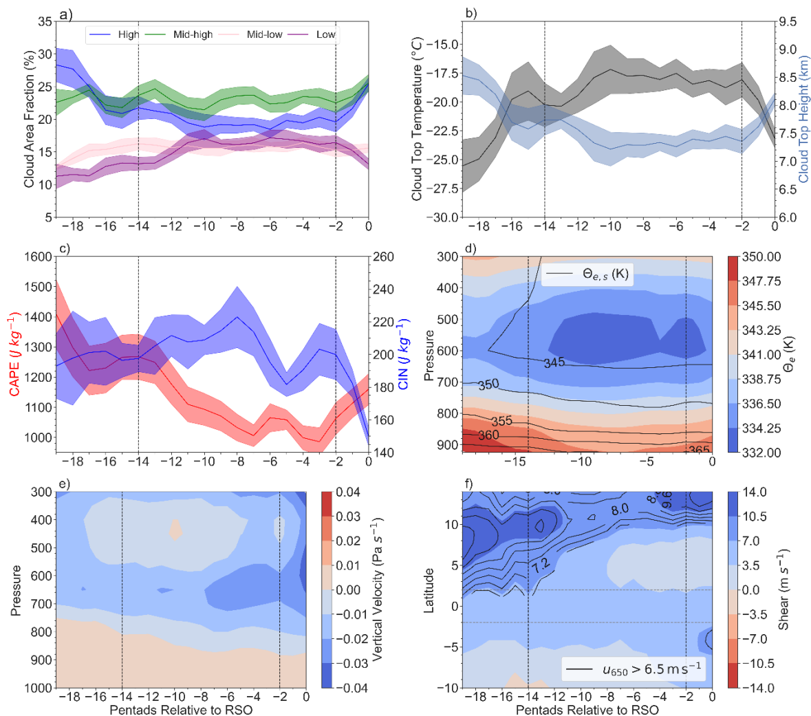
Figure 12: Prior to the fall RSO: (a) cloud area fraction for high, mid-high, mid-low, and low clouds; (b) cloud top temperature and cloud top height; (c) CAPE; and CIN; (d) equivalent potential temperature ( \theta_e ; shades) and saturated
