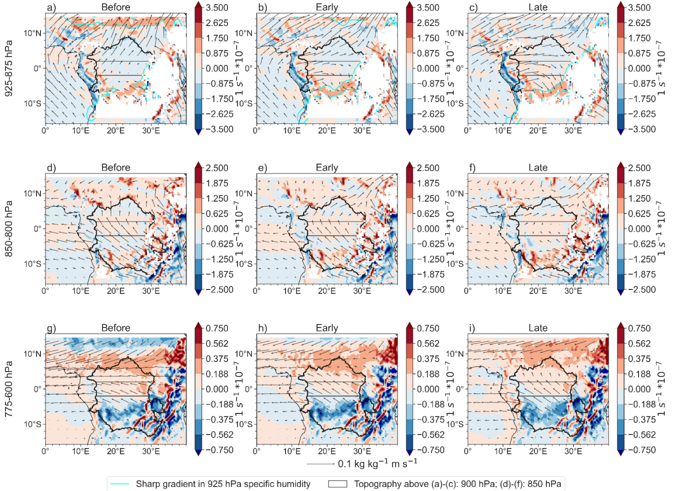
330 Figure 10: Moisture transport vectors ( q * v ) and moisture convergence ( q * DIV ; shades, positive means convergence) for (a)-(c) average of 925-875 hPa. The westerly winds represent the lower branch inflow of the Congo Basin Cell; the aqua shades denote areas of sharp 925 hPa specific humidity gradients. The southern aqua gradients therefore note the rough location of the Congo Air Boundary. (d-f) average of 850-800 hPa; and (g-i) average of 775- 600 hPa. The easterly winds represent the upper branch return flow of the Congo Basin Cell. Vectors have been 335 multiplied by a scale factor of 2 in all panels. Area of convergence between 4°S and 8°S in a-c) represents the rough location of the Congo Air Boundary (CAB). Mainly zonal moisture transport between 6°N – 15°N represents the AEJ- N.
