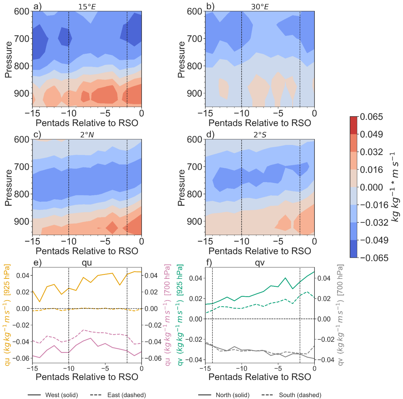
565 Figure B1: (a) Zonal moisture transport ( q * u ) across 15^{\circ}\text{E} and between 2^{\circ}\text{S} - 2^{\circ}\text{N} ; (b) zonal moisture transport ( q * v ) across 30^{\circ}\text{E} and between 2^{\circ}\text{S} - 2^{\circ}\text{N} . Note that contours below 875 hPa should not be considered as they are below the East African Rift, but all pressure levels are shown to emphasize the mid-level moisture transport. (c) meridional
