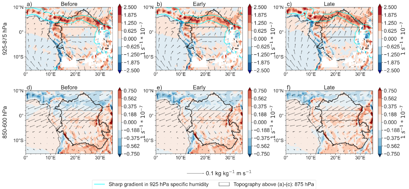
255 Figure 4: Moisture transport vectors ( q * v ) and moisture convergence term ( q * DIV ; shades, positive means convergence) for (a)-(c) average of 925-875 hPa for the “before” (15-11 pentads prior to the spring RSO), early, and late transition periods, respectively; (d)-(f) average of 850-600 hPa for the “before,” early, and late transition periods, respectively. Vectors are scaled up by a factor of 2 to better visualize the changes in magnitude and direction between periods. White masks in (a)-(c) represent areas where the elevation is higher than 875 hPa. Aqua contours in (a)-(c) represent sharp 925 hPa specific humidity gradients, which overlap with the area of convergence.
