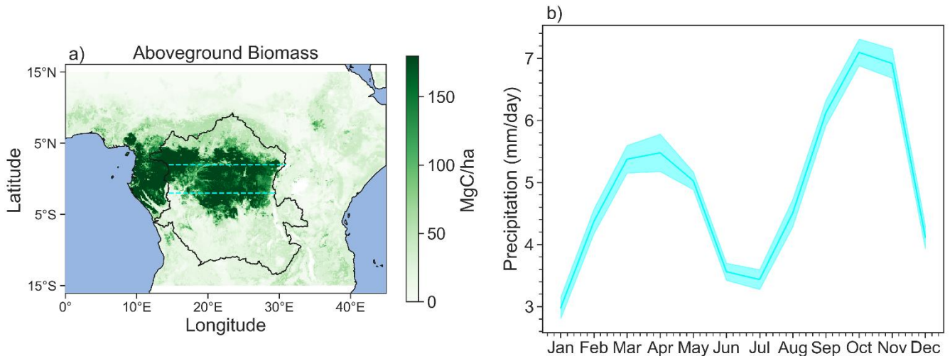
Figure 1: (a) Above-ground biomass averaged between 2000-2019. Black outline denotes the Congo Basin watershed and the dashed lines at 2°S and 2°N represent the boundary of the equatorial region. (b) Precipitation climatology for the equatorial region. Shades are the standard error of the mean over of the different years.
