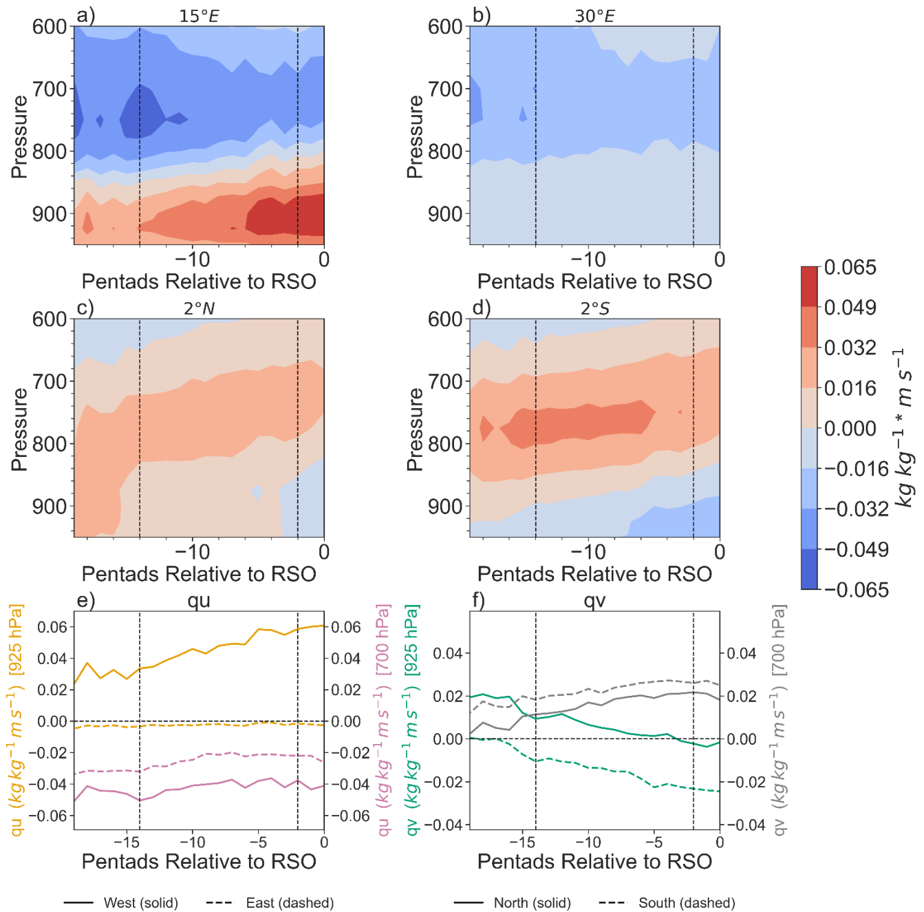
Figure B2: a) zonal moisture transport ( q * u ) across 15^\circ E and between 2^\circ S - 2^\circ N ; b) zonal moisture transport ( q * v ) across 30^\circ E and between 2^\circ S - 2^\circ N . Note that contours below 875 hPa should not be considered as they are below the East African Rift, but all pressure levels are shown to emphasize the mid-level moisture transport. c) meridional moisture transport ( q * v ) across 2^\circ N and between 15^\circ E - 30^\circ E ; and d) meridional moisture transport ( q * v ) across 2^\circ S and between 15^\circ E - 30^\circ E ; e) zonal moisture transport at 925 hPa (orange) and 700 hPa (purple) across the western and eastern boundaries; and f) meridional moisture transport at 925 hPa (green) and 700 hPa (grey) across the
