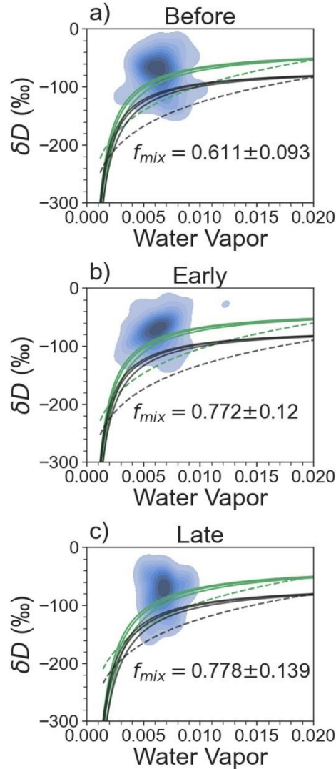
270 Figure 5: Fraction of observed \delta D above a series of mixing (solid) and Rayleigh (dashed) models. Blue shades represent a density map of the TES \delta D observations. Green indicates land-based water vapor models, while black indicates ocean-based water vapor models. f_{mix} is the fraction of observed \delta D above the uppermost, land-based mixing
