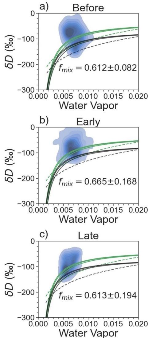
345 Figure 11: Fraction of observed \delta D above a series of mixing (solid) and Rayleigh (dashed) models. Blue shades represent a density map of the TES \delta D observations. Green indicates land-based water vapor models, while black indicates ocean-based water vapor models. f_{mix} is the fraction of observed \delta D above the uppermost, land-based mixing
