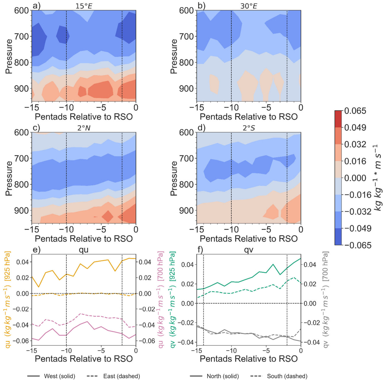
615 Figure B1: (a) Zonal moisture transport ( q \cdot u ) across 15^\circ E and between 2^\circ S - 2^\circ N ; (b) zonal moisture transport ( q \cdot v ) across 30^\circ E and between 2^\circ S - 2^\circ N . Note that contours below 875 hPa should not be considered as they are below the East African Rift, but all pressure levels are shown to emphasize the mid-level moisture transport. (c) meridional
