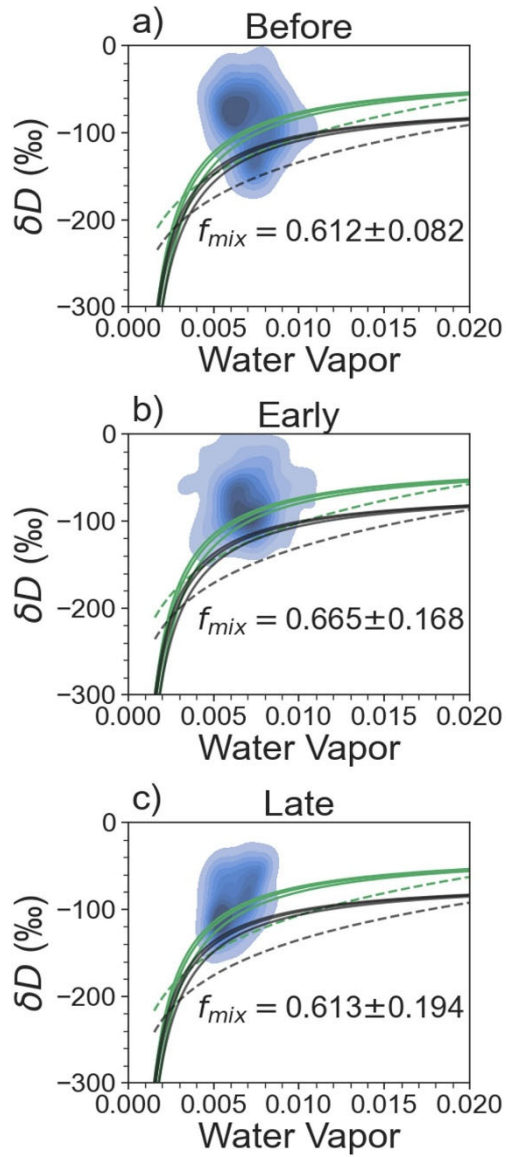
380 Figure 11: Fraction of observed \delta D above a series of mixing (solid) and Rayleigh (dashed) models. Blue shades represent a density map of the TES \delta D observations. Green indicates land-based water vapor models, while black indicates ocean-based water vapor models. f_{mix} is the fraction of observed \delta D above the uppermost, land-based mixing model. For (a) the “before” period (19-14 pentads prior to the fall RSO); (b) the early-transition; and (c) the late-transition.
