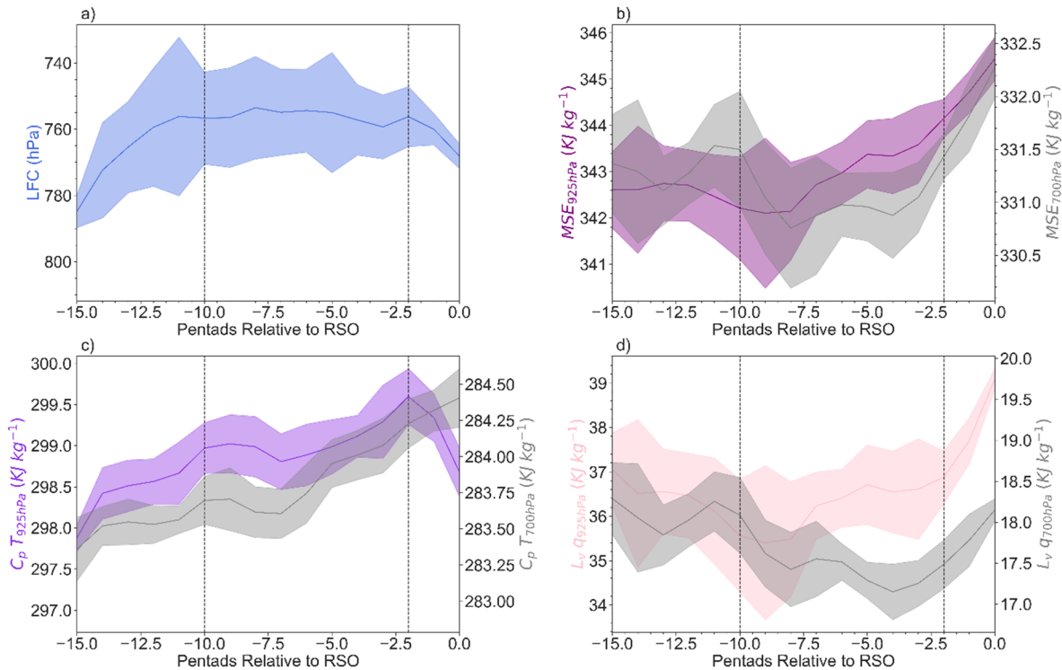
330 Figure 7: Evolution of (a) the level of free convection (LFC); (b) MSE at 925 hPa and 700 hPa; (c) MSE component C_p T at 925 hPa and 700 hPa; and (d) MSE component L_v q at 925 hPa and 700 hPa. All are relative to the spring RSO, averaged between 14^\circ E - 26^\circ E to avoid topography errors in the calculations, and smoothed using the Savitsky-Golay filter. Shades represent the standard error of the mean of the different years.
