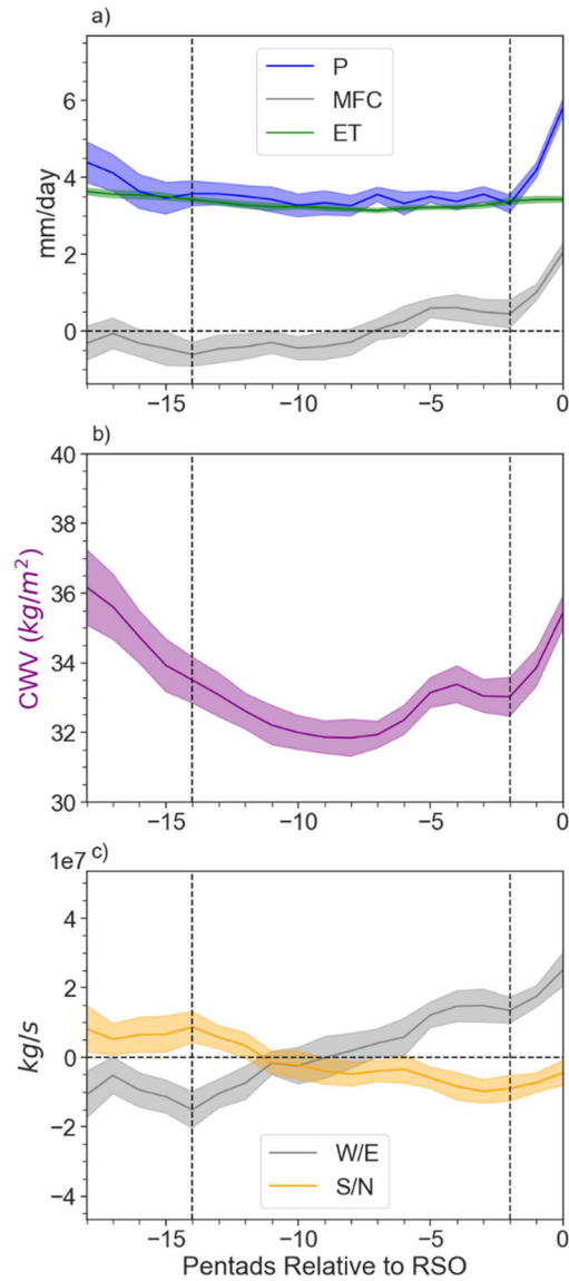
Figure 9: For the transition to the fall RSO: (a) Precipitation (P), vertically integrated MF convergence ( MFC ), and evapotranspiration (ET); (b) column water vapor (CWV); (c) Net MF across the zonal (West—East) and meridional (South—North) boundaries Q_{zonal} and Q_{meridional} (Methods; Units: \text{kg/s} \cdot 10^7 ). Positive means convergence, negative means divergence. All are relative to the RSO (denoted as '0' in the graph). All have been
