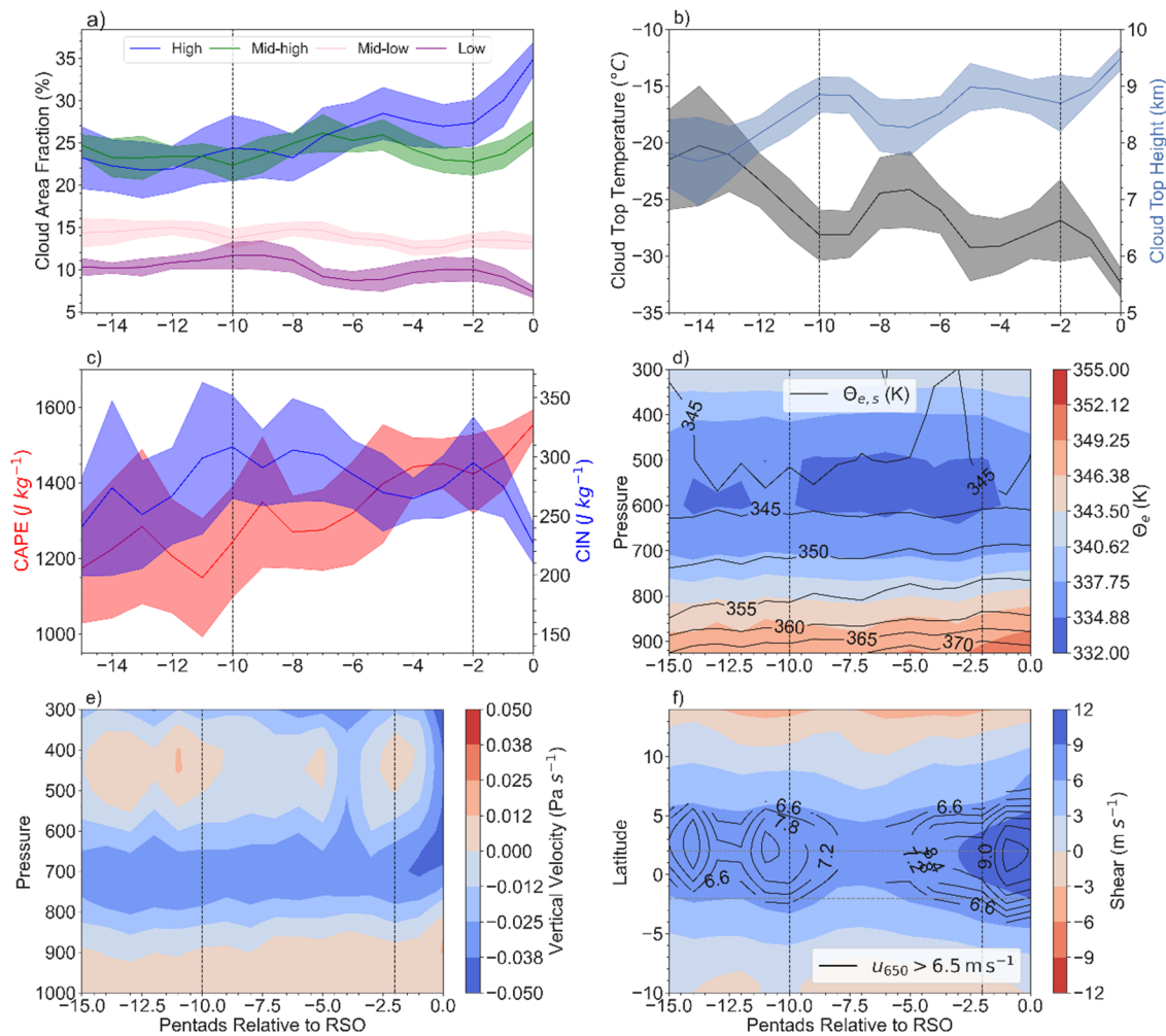
310 Figure 6: Prior to the spring RSO: (a) cloud area fraction for high, mid-high, mid-low, and low clouds; (b) cloud top temperature and cloud top height; (c) convective available potential energy CAPE; and CIN convective inhibitive energy; (d) equivalent potential temperature ( \theta_e ; shades) and saturated equivalent potential temperature ( \theta_{e,s} ); (e) vertical velocity; and (f) black contours: 650 hPa zonal wind ( u_{650} ) greater than 6.5 \text{ m s}^{-1} , denoting the AEJ-N. Shaded contours represent the wind
