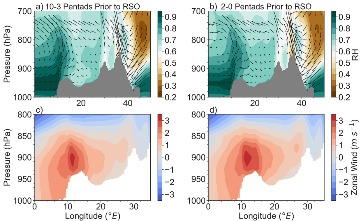
345 Figure 8: Relative humidity (shades) and vectors of u and \omega * 10^2 for (a) 10-3 pentads prior to the spring RSO; (b) 2-0 pentads prior to the spring RSO. Zonal wind ( u ) for (c) 10-3 pentads prior to the spring RSO; (d) 2-0 pentads prior to the spring RSO. Grey shading in (a)-(b) and white shading in (c)-(d) denotes the topography of the region.
