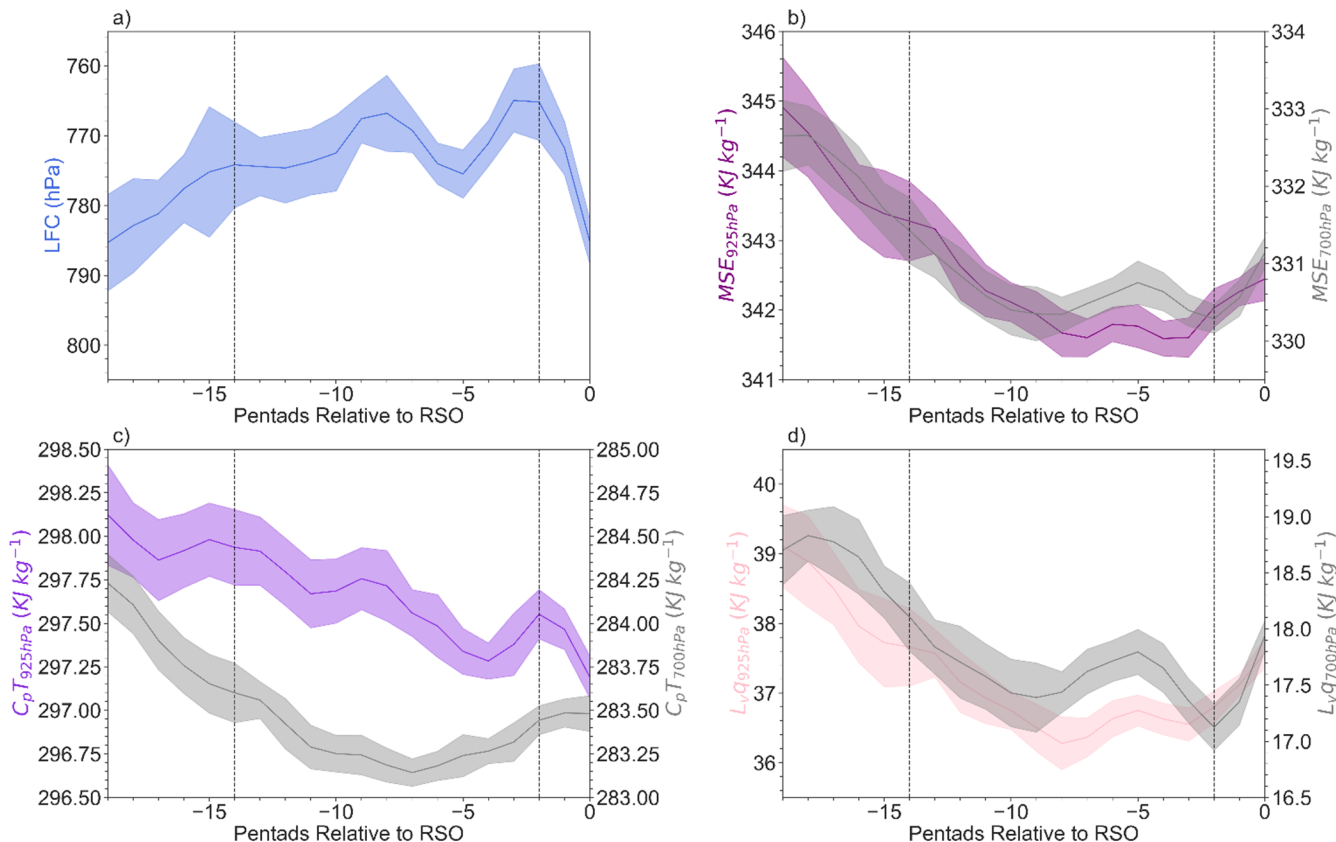
400 Figure 13: Evolution of (a) level of free convection (LFC), (b) MSE at 925 hPa and 700 hPa; (c) C_pT at 925 hPa and 700 hPa; and (d) L_vq at 925 hPa and 700 hPa. All are prior to the fall rainy season. All are averaged between 14E^\circ - 26^\circ E to account for effects of topography in the eastern part of the region. All have been smoothed using a Savitsky-Golay filter. Shades represents the standard error of the mean of the different years.
