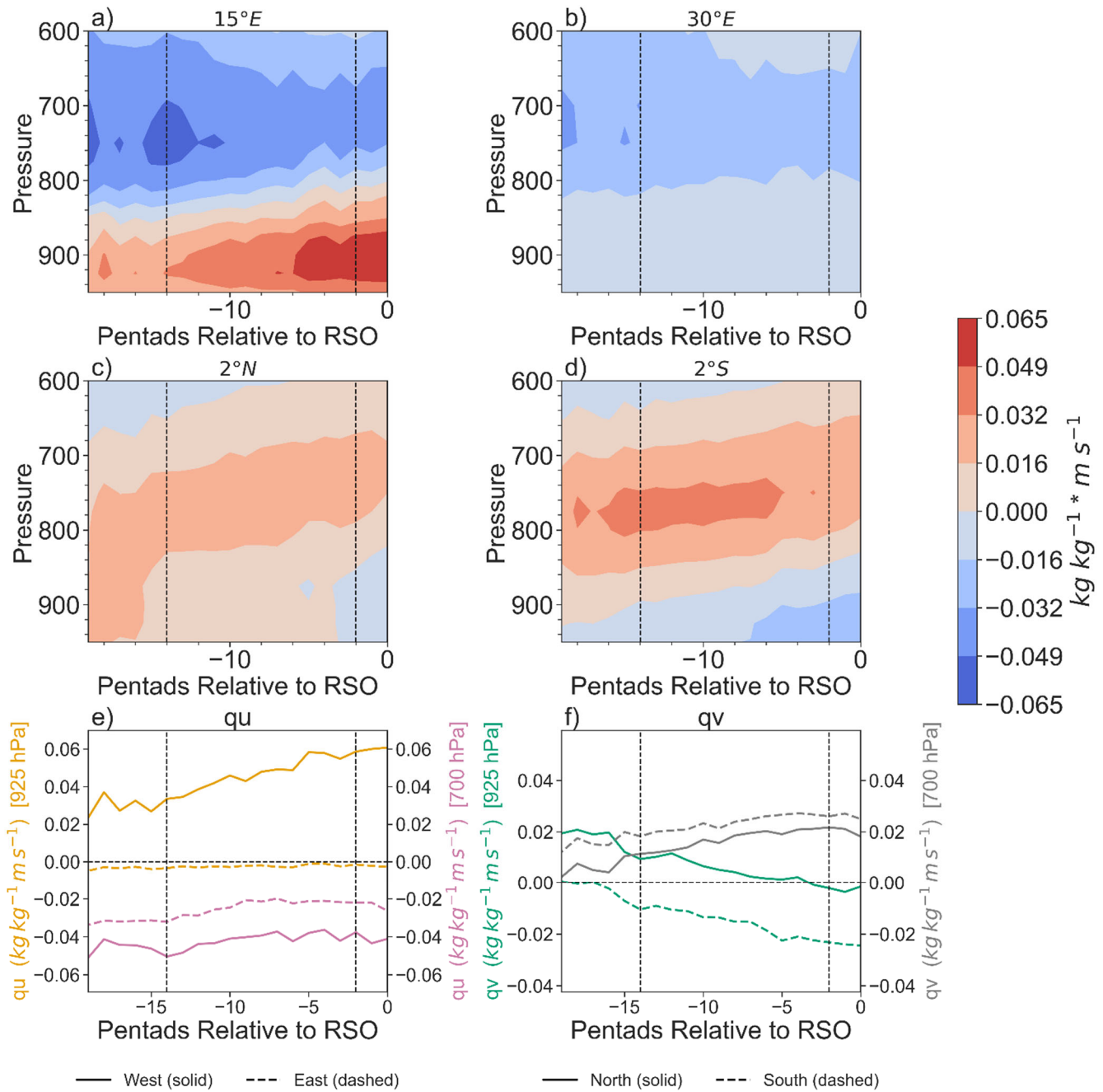
625 Figure B2: a) zonal moisture transport ( q * u ) across 15^{\circ}E and between 2^{\circ}S - 2^{\circ}N ; b) zonal moisture transport ( q * v ) across 30^{\circ}E and between 2^{\circ}S - 2^{\circ}N . Note that contours below 875 hPa should not be considered as they are below the East African Rift, but all pressure levels are shown to emphasize the mid-level moisture transport. c) meridional moisture transport ( q * v ) across 2^{\circ}N and between 15^{\circ}E - 30^{\circ}E ; and d) meridional moisture transport ( q * v ) across 2^{\circ}S and between 15^{\circ}E - 30^{\circ}E ; e) zonal moisture transport at 925 hPa (orange) and 700 hPa (purple) across the western and eastern boundaries; and f) meridional moisture transport at 925 hPa (green) and 700 hPa (grey) cross the 630
