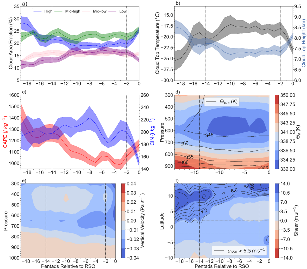
390 Figure 12: Prior to the fall RSO: (a) cloud area fraction for high, mid-high, mid-low, and low clouds; (b) cloud top temperature and cloud top height; (c) convective available potential energy CAPE; and convective inhibitive energy CIN; (d) equivalent potential temperature ( \theta_e ; shades) and saturated equivalent potential temperature ( \theta_{e,s} ); (e) vertical velocity; and (f) black contours: 650 hPa zonal wind greater than 6.5 m/s, denoting the AEJ-N. Shaded contours represent the wind shear ( u_{900} - u_{650} ). Shades of the time series in (a)- (c) represent the standard error of
