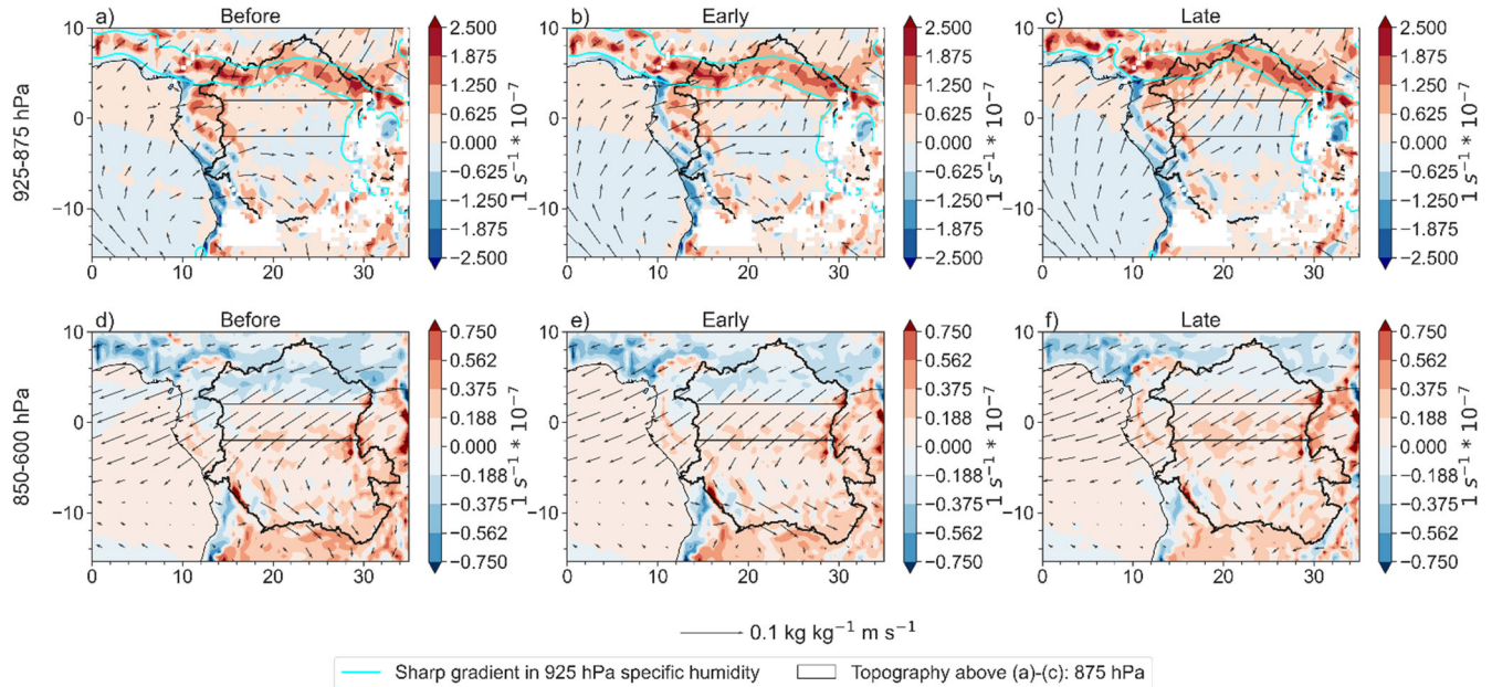
285 Figure 4: Moisture transport vectors ( q * v ) and moisture convergence ( q * DIV ; shades, positive means convergence) for (a)-(c) average of 925-875 hPa for the “before,” early, and late transition period, respectively; (d)-(f) average of 850-600 hPa for the “before,” early, and late transition period, respectively. Vectors are scaled up by a factor of 2 to better visualize the changes in magnitude and direction between periods. White masks in (a)-(c) represent areas where the elevation is higher than 875 hPa. Aqua contours in (a)-(c) represent sharp 925 hPa specific humidity gradients, which overlap with the area of convergence. 290
