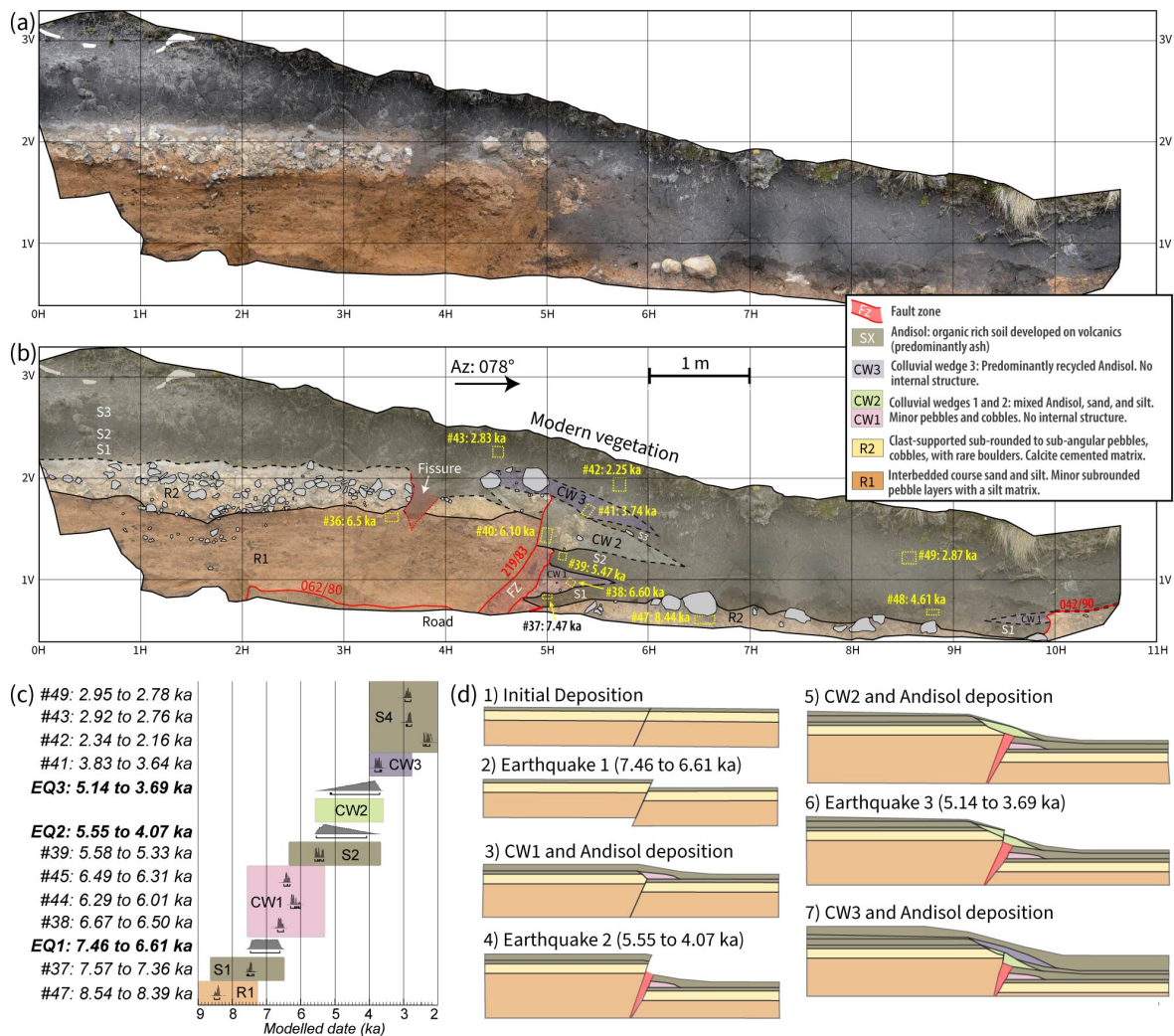
Figure 7. Unannotated (a) and interpreted (b) orthophotomosaics of an exposure of the middle segment of the northern Reservoir faultzone. Local grid coordinates are 1 m by 1 m. Outcrop location shown in Fig. 5d. Bulk radiocarbon sample locations shown with yellow boxes and ages are mean calibrated ages before present (in thousands of years before 1950). c) Results of Bayesian model of radio-carbon-radiocarbon dates showing age ranges for sedimentary units and three earthquakes. The coloured boxes show the maximum possible time range for each stratigraphic unit based on the model. The ages of sample #36 and sample #40 are anomalous as they are out of stratigraphic order likely due to recycling or bioturbation, and the stratigraphic position of sample #48 relative to CW1 is unclear. These sample were not used in the model. Two radiocarbon dates from CW1 are from the exposure of the southern fault branch in Fig. 6c. See Table 2 for the full dataset of uncalibrated and calibrated radiocarbon ages. d) Cartoon illustrating the stratigraphic evolution of the exposed deposits and faults in the exposure shown in (a) and (b).
